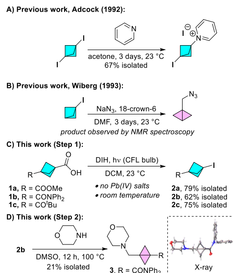
Scheme 2. Substituted BCBs can be prepared in two steps from commercially available BCP carboxylic acids.
