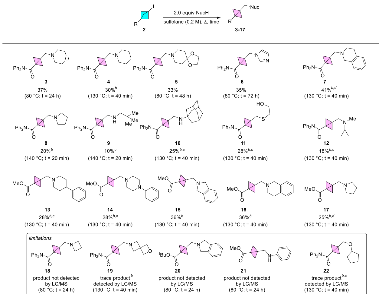
Scheme 3. Substrate scope of BCP to BCB substitution reaction. a
