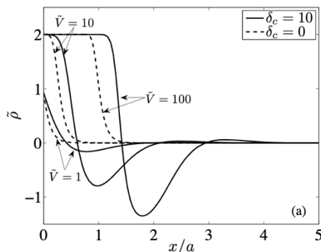
Figure 9. Charge density as a function of distance from the interface, for various surface voltages, and correlation parameters \delta_c = l_c/\lambda_d . Reproduced with permission from reference 59 . Copyright 2011 American Physical Society.
