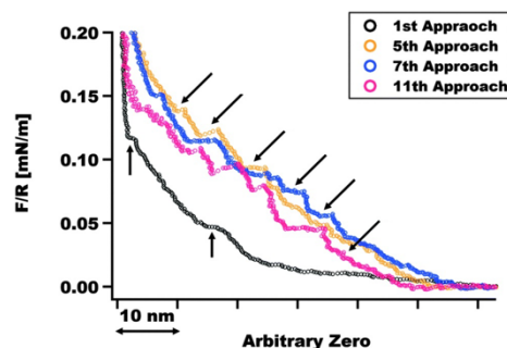
Figure 7. Surface forces measured with a colloidal probe ( \text{SiO}_2 ) on mica in dry [\text{C}_6\text{C}_1\text{Im}][\text{EtSO}_4] by AFM. The measurements were taken at an offset position of 50 \mu\text{m} from the location of the initial measurement. The results from the 1 st , 5 th , 7 th , and 11 th approach of the colloidal probe to mica are shown here. Adapted with permission from reference 40 . Copyright 2015. Royal Society of Chemistry.
