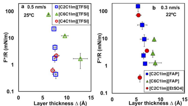
Figure 3. Layer sizes and force applied to squeeze out IL layers in a) [\text{C}_2\text{C}_1\text{Im}][\text{TFSI}] , [\text{C}_4\text{C}_1\text{Im}][\text{TFSI}] and [\text{C}_6\text{C}_1\text{Im}][\text{TFSI}] and b) [\text{C}_2\text{C}_1\text{Im}][\text{FAP}] , [\text{C}_6\text{C}_1\text{Im}][\text{FAP}] and [\text{C}_2\text{C}_1\text{Im}][\text{EtSO}_4] . Abbreviation: 1-n-alkyl 3-methylimidazolium [\text{C}_n\text{C}_1\text{Im}]^+ , with n=2, 4 and 6 for ethyl, butyl and hexyl, respectively; [\text{TFSI}] =bis(trifluoromethanesulfonyl)imide. Adapted with permission from reference 28 . Copyright 2018 American Chemical Society.
