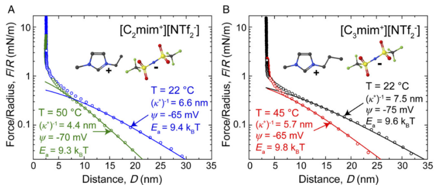
Figure 4. Surface forces across (A) [C_2C_1Im][TFSI] at T=22\text{ }^\circ\text{C} and 50\text{ }^\circ\text{C} , and (B) [C_3C_1Im][TFSI] at T=22\text{ }^\circ\text{C} and 45\text{ }^\circ\text{C} , using the nomenclature for ILs in this article. Reproduced with permission from reference 37 . Copyright 2015 National Academy of Sciences of the United States of America.
