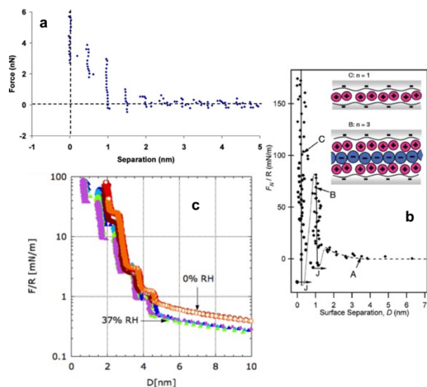
Figure 2. a) Surface forces measured with an AFM tip approaching a mica surface in EAN. Adapted with permission from reference 12. Copyright 2007 American Chemical Society. b) Surface forces between mica surfaces in [\text{C}_2\text{C}_1\text{Im}][\text{EtSO}_4] measured by SFB. Reproduced with permission from reference 22. Copyright 2010 Royal Society of Chemistry. c) Surface forces between mica surfaces in [\text{C}_2\text{C}_1\text{Im}][\text{FAP}] at 0 and 37% RH. Abbreviations: FAP= tris(pentafluoroethyl)trifluorophosphate. Adapted with permission from reference 23. Copyright 2014 American Chemical Society.
