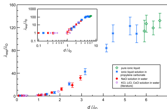
Figure 5. Experimental decay length over the Debye length, \lambda_{\text{exp}}/\lambda_{\text{D}} , versus d/\lambda_{\text{D}} for [\text{C}_4\text{C}_1\text{Pyrr}][\text{NTf}_2] , its mixtures with propylene carbonate, aqueous NaCl, LiCl, KCl, and CsCl solutions. Adapted with permission from reference 17. Copyright 2016 American Chemical Society.
