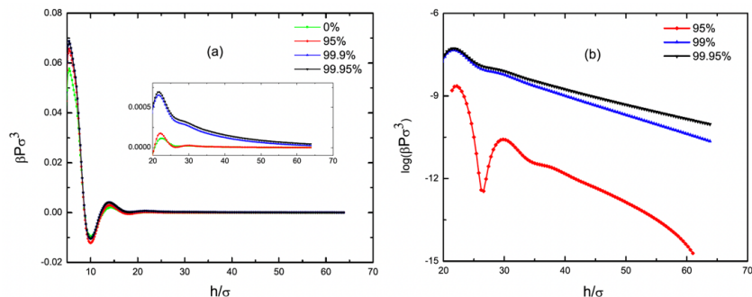
Figure 12. Surface pressure calculated between like-charged interfaces, for various extents of ion pairing. Reproduced with permission from reference 69 . Copyright 2015 AIP Publishing.
