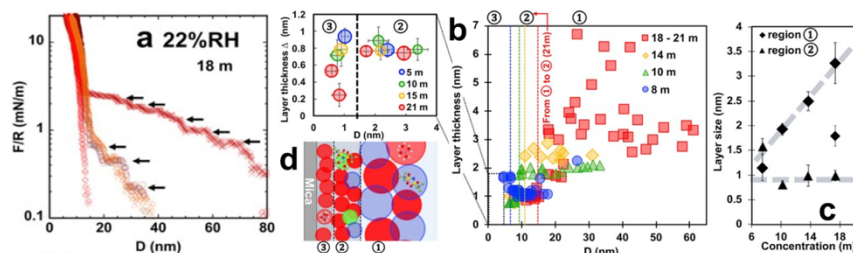
Figure 14. a) Surface forces in LiTFSI 18m in water between mica surfaces measured by eSFA, b) Layer size vs. separation between the mica surfaces. The inset shows the size of the layers at separations smaller than 4 nm. c) Layer thickness as a function of the concentration of LiTFSI in water. d) Cartoon of the interfacial structure of superconcentrated LiTFSI in water. There are three different regions based on the interfacial layers inferred from short-range and long-range forces. Adapted with permission from reference 42 . Copyright 2021 American Chemical Society.
