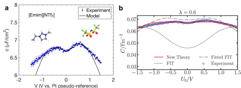
Figure 13. a) Differential capacitance of [C_2C_1Im][TFSI] with the markers representing the experiment and the solid lines corresponding to the fit of the extended mean-field model to experimental results. Reproduced with permission from reference 87 . Copyright 2018 American Chemical Society. b) The new theory by Goodwin et al. is in better agreement with the experimental differential capacitance than the free ion theory (FIT). Reproduced with permission from reference 81 . Copyright 2022 AIP Publishing.
