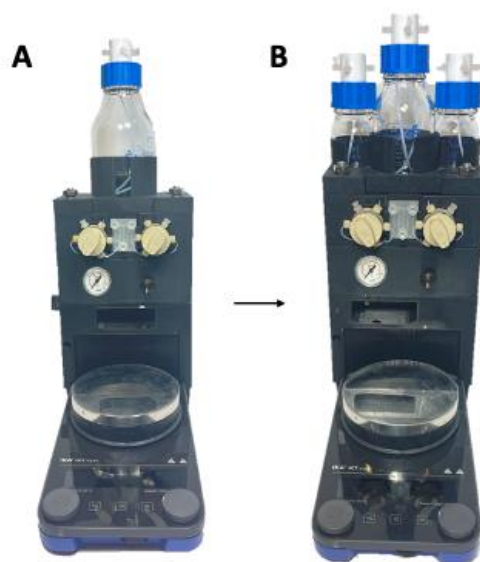
Figure 3: A) Digitised flow chemistry system on the left, B) scaled-up version of the continuous flow system on the right.
