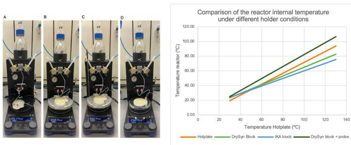
Figure 6: Temperature measurements set up. A) With the IKA Block. B) With the DrySyn Block. C) With the DrySyn Block and the temperature probe connected. D) Directly on top of the Hotplate. Graph 1: temperature variations depending on holder conditions.
