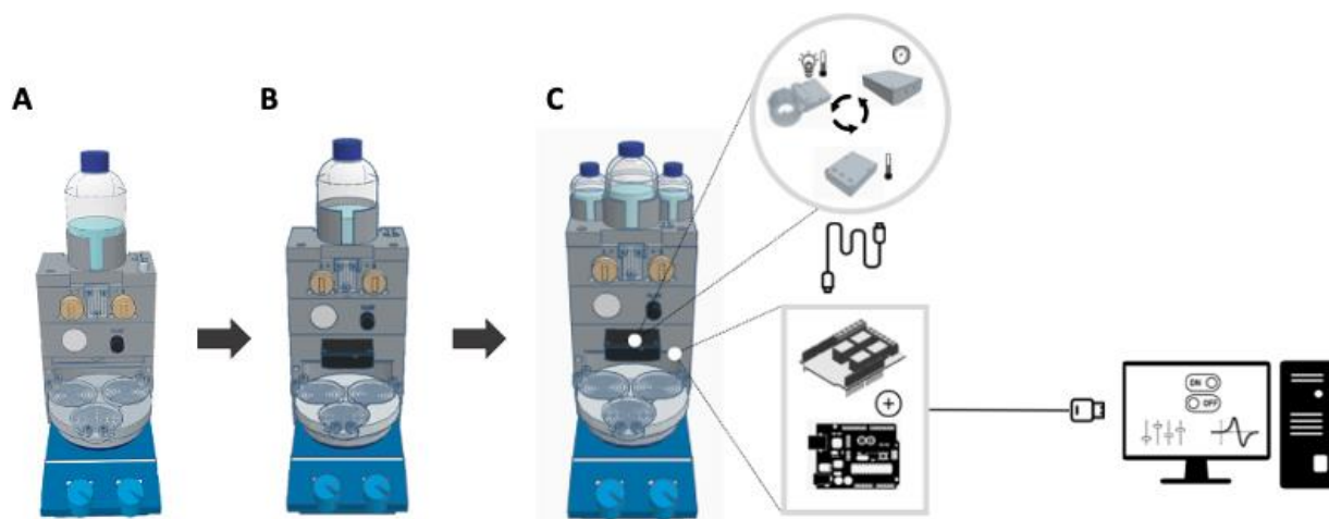
Figure 1: Tinkercad representative design of the proposed modular continuous flow chemistry system. A) Analog system. B) Digital system. C) Scale-up version of the digital system.
