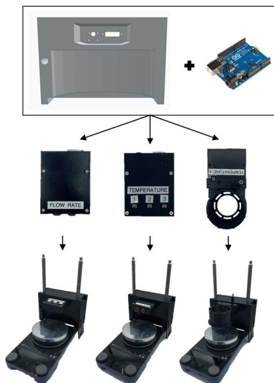
Figure 2: 3D design of continuous flow base block. Top designs correspond to the Tinkercad design of the digital system in addition to the Arduino Uno Rev 2 and bottom designs correspond to the digitized base block with the three different modules plugged in.
