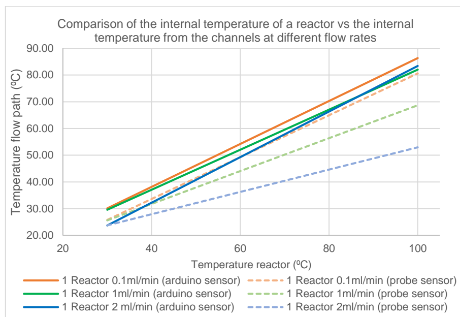
Graph 1: Correlation between the internal temperatures of a reactor and the internal temperature from the reactors channel at different flow rates.
