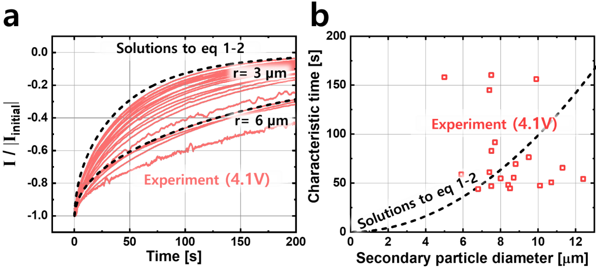
Fig. 5. Direct estimates of characteristic electrochemical timescales from PITT measurements a) The PITT current traces for all particles at 4.1V normalized to the initial current at t=0.1 s. The solutions to equation (1-2) under the assumption that D_{Li} = 3.8 \cdot 10^{-10} \text{ cm}^2 \text{ s}^{-1} and j_0 = 0.014 \text{ mA cm}^{-2} , which are the median of D_{Li} and j_0 obtained at 4.1V (Table S1), are plotted in black. b) The characteristic electrochemical timescale as a function of particle diameter. The characteristic time is defined as when I/I_{\text{initial}} = \exp(-1) , and represents a convolution of \tau_D and \tau_R . Whereas equations (1-2) suggest that large particles require longer timescales, our results show no size dependence. This result shows that the diameter-independent \tau_D and \tau_R found in Fig. 4 can be observed in the raw data and are not artifacts of our analysis procedure. The same trends are measured for the other voltages (Fig. S17).
