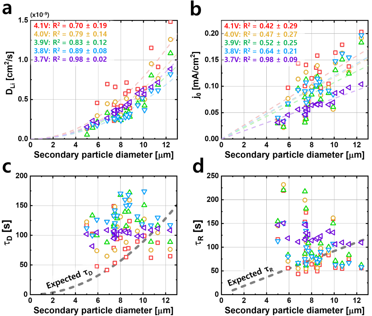
Fig. 4. The dependence of the measured electrochemical parameters as a function of particle diameter a, b) The relation between the measured D_{Li} and j_0 with the diameter of each particle under five different target voltages. Dashed lines are linear (quadratic) fitting lines that pass through the origin. The R^2 is calculated along with its 95% confidence interval. c, d) The computed diffusion \tau_D and reaction \tau_R times. The diffusion time is computed using \tau_D = l^2/4D_{Li} , where l equals the radius of the secondary particle. The reaction time is computed from j_0 using an effective RC time constant (detailed in Methods).
