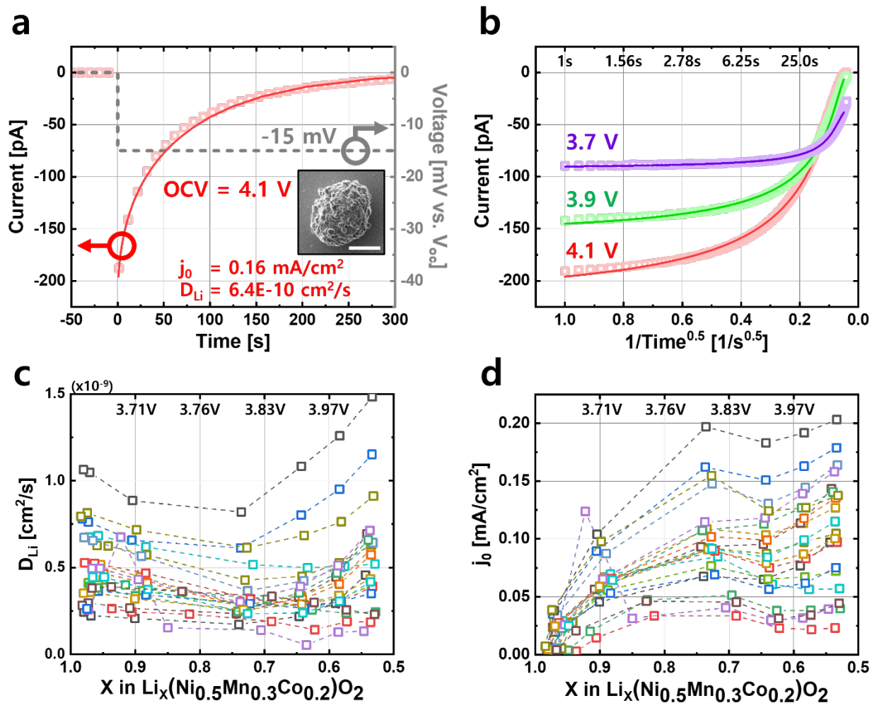
Fig. 3. Obtaining single-particle exchange current density ( j_0 ) and lithium diffusivity ( D_{Li} ) using potentiostatic intermittent titration (PITT) a) Each particle was discharged to a given voltage and held for 1 hour at open-circuit voltage ( V_{oc} ). Afterwards, a -15 mV PITT voltage was applied, and the electrochemical current was recorded over 1200 seconds. We fit the data to equations (1-2) to obtain j_0 and D_{Li} . The inset image is an SEM image of the particle used in this PITT measurement. b) Current responses of PITT measurement and fits to equations (1-2) under three different target voltages. The time scale is converted to an inverse root scale. c, d) The exchange current density j_0 and lithium diffusivity D_{Li} estimated from the PITT fitting for 21 particles at various voltages. We assume that the radius parameter in equation (1-2) equals the radius of the secondary particle computed from SEM images, or r_{Secondary} . Each color represents a different particle.
