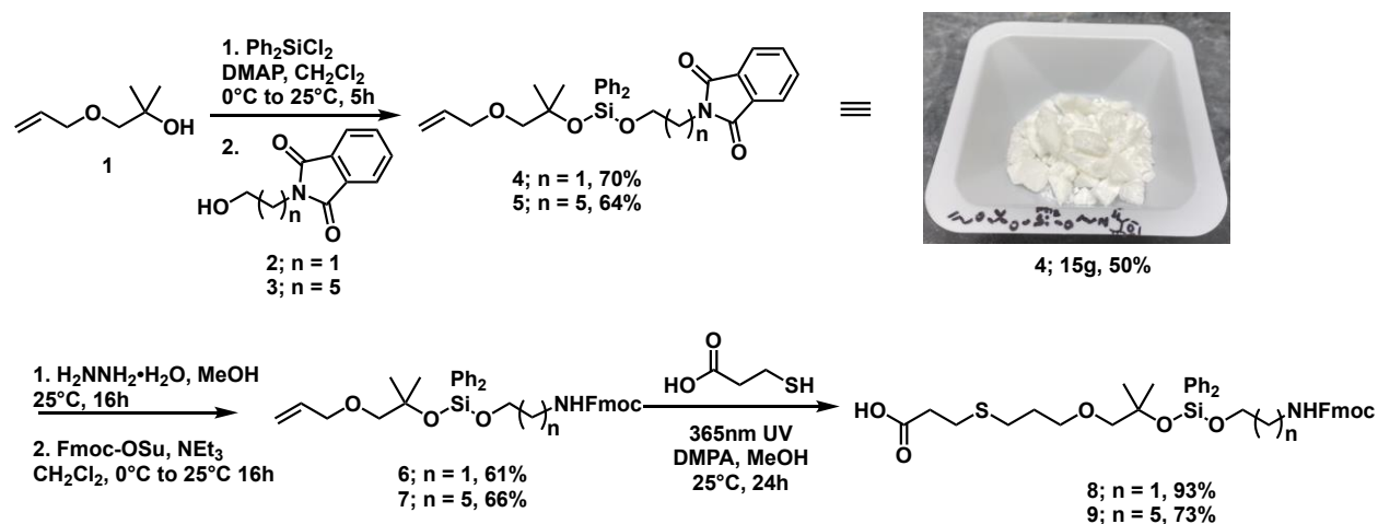
Scheme 1. Synthesis of solid-phase compatible DADPS-Fmoc reagents 8 and 9 , which were obtained in 39% and 31% overall yields, respectively.
