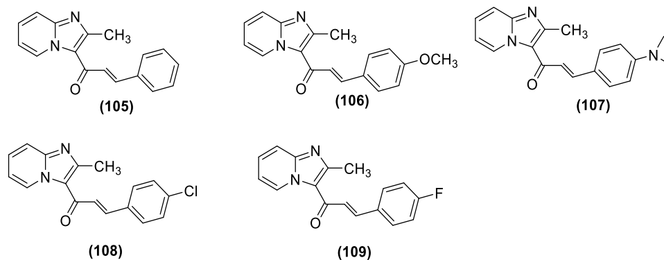
Figure 21: 3-(phenyl)-1-(2-methyl H -imidazo[1,2- a ]pyridin-3-yl)prop-2-en-1-one derivatives against Plasmodium Falciparum
