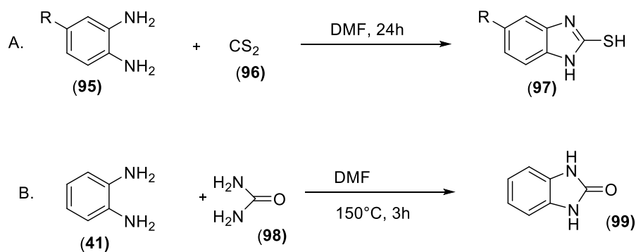
Figure 17: A. Synthesis of mercapto-1H-benzimidazole according to Van Allan et al. B. Synthesis of 1,3-dihydrobenzimidazol-2-one according to Bhanage et al.
