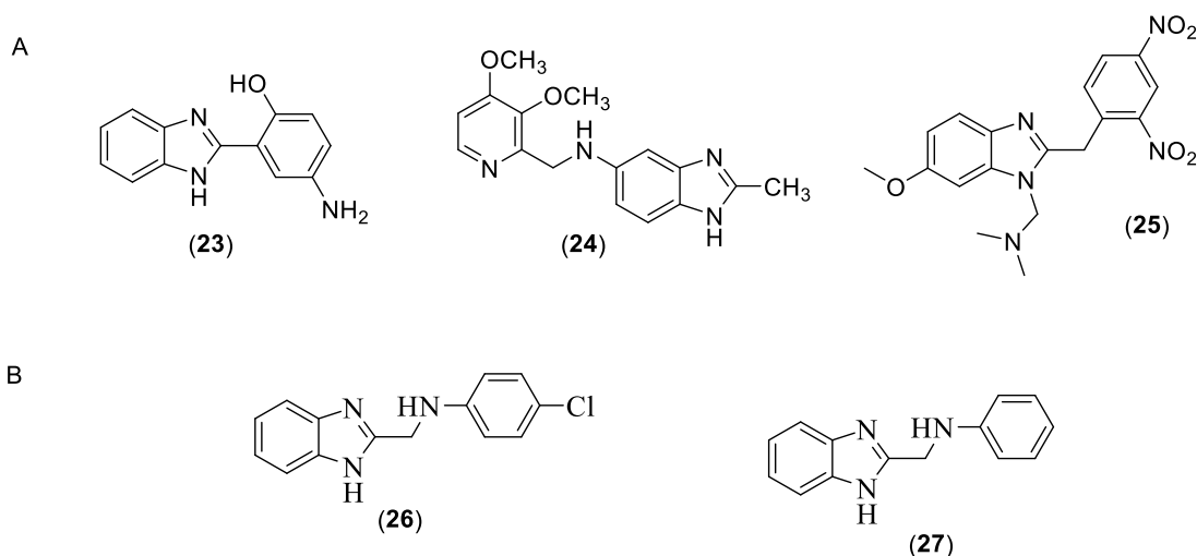
Figure 7 : A. Benzimidazole derivatives ( 23-25 ). ref.43 B. N-((1 H -benzimidazol-2-yl)methyl)aniline derivatives with good anti-inflammatory activities ( 26-27 ). ref.44
