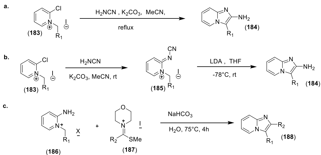
Figure 33: a. Synthesis method of 2-aminoimidazopyridine derivatives from pyridinium salt according to Juan A. Vega et al. b. Synthesis method of 2-aminoimidazopyridine derivatives from pyridinium salt according to Juan A. Vega in two steps. c. Synthesis method of 2-aminoimidazopyridine derivatives from pyridinium salt according to Zali-Beoini
