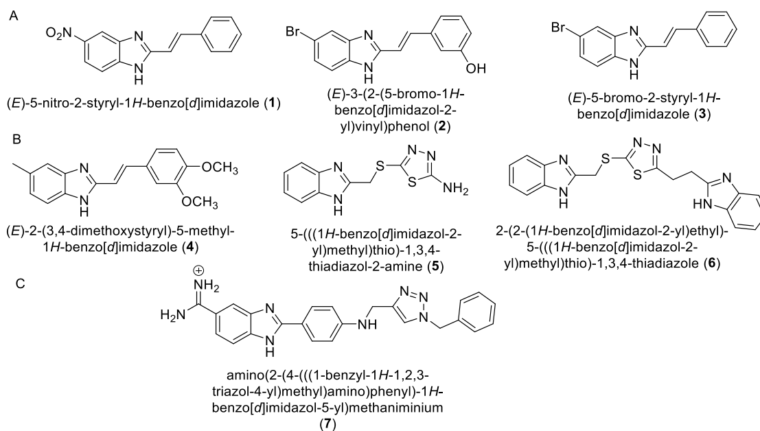
Figure 2: Compound with good antimicrobial activities-A. 2-styryl-1H-benzimidazole derivatives, B. 5-(((1H-benzimidazol-2-yl)methyl)thio)-1,3,4-thiadiazol-2-amine derivatives, C. Amino-(2-(4-(((1-benzyl-1H-1,2,3-triazol-4-yl)methyl)amino)phenyl)-1H-benzimidazol-5-yl) methaniminium.
