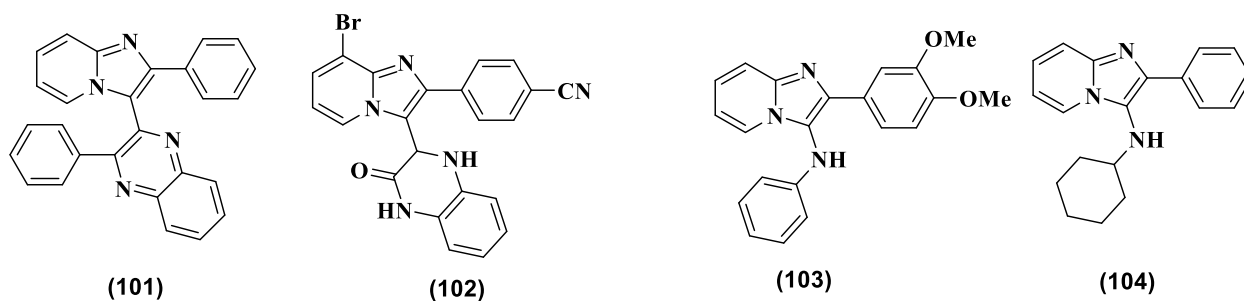
Figure 20 : Modulations around the imidazopyridine core conferring anticancer activities.
