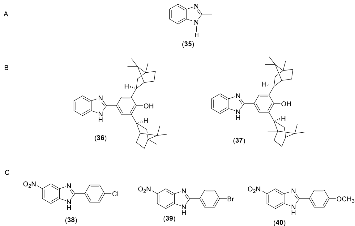
Figure 10: A. 2-methyl-1 H -benzimidazole B. 2-hydroxylphenyl benzimidazole derivatives C. 5-nitrobenzimidazole derivatives
