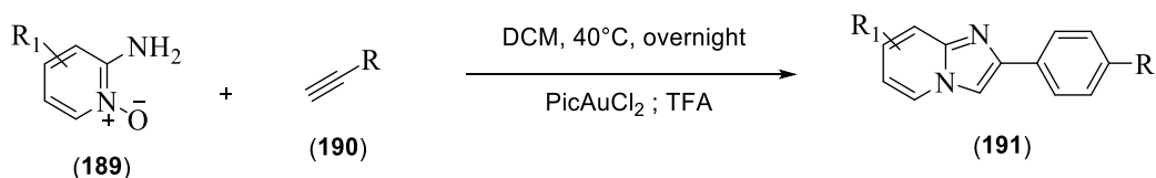
Figure 34 : Synthesis method of 2-phenyl imidazopyridine derivatives from N-oxides
