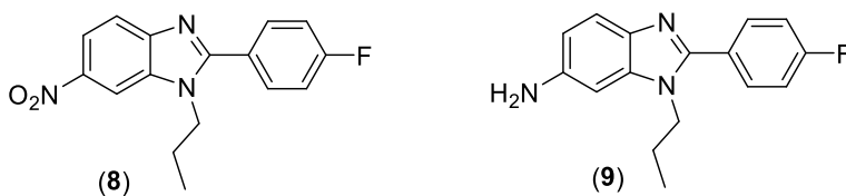
Figure 3: 2-(4-fluorophenyl)-1-propyl-1 H -benzimidazole derivatives with antifungal activities.
