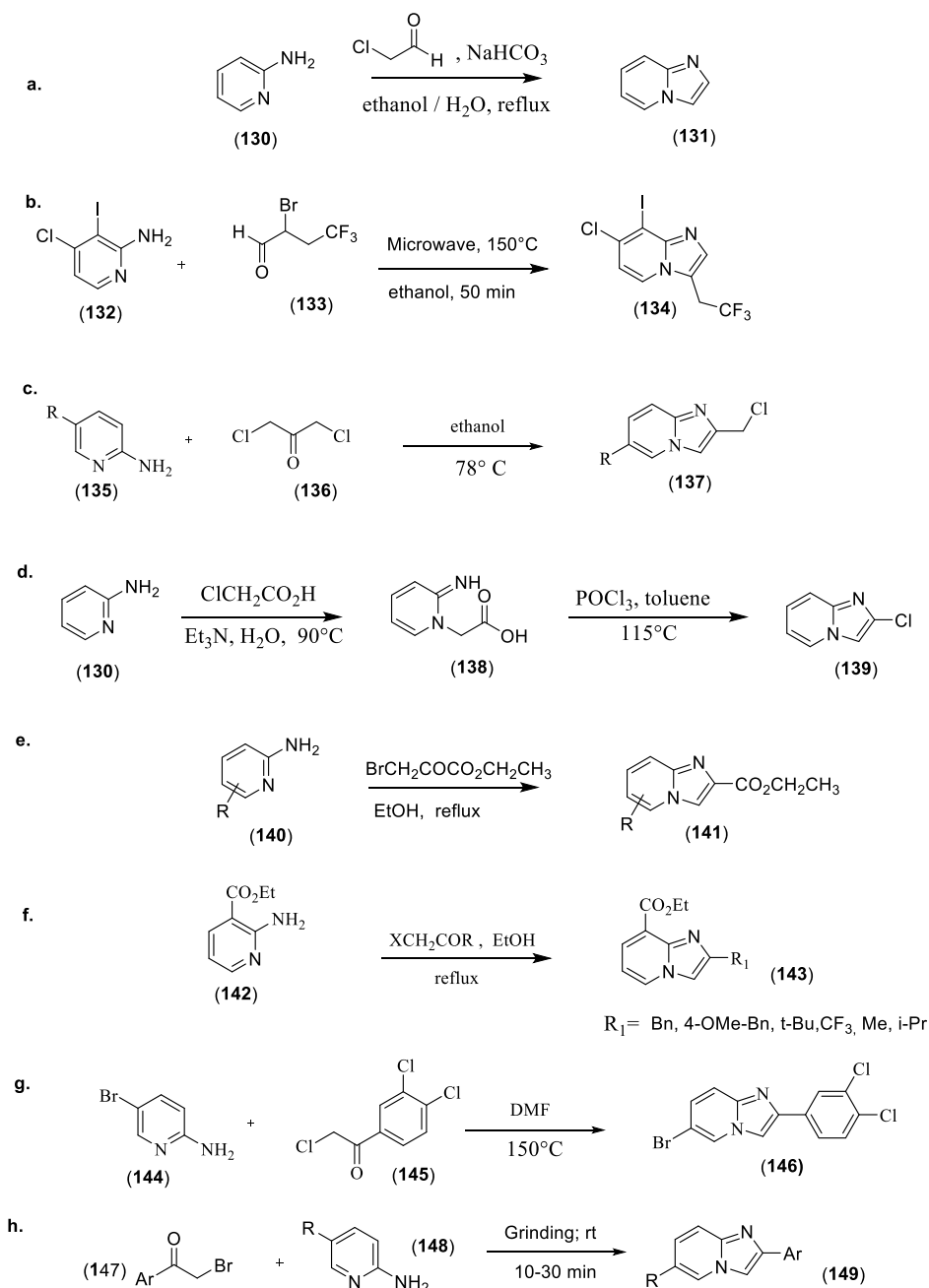
Figure 29: a. Chichibabin method of imidazopyridine synthesis b. synthesis of 3-(2,2,2-trifluoroethyl) H -imidazo[1,2- a ]pyridine according to Andrés A. Trabanco et al. c. Synthesis method of 2-chloromethyl imidazopyridine derivatives according to Caroline Castera-Ducros et al. d. Synthesis method of 2-chloroimidazopyridine according to Brad D. Maxwell et al. e. Synthesis method of ethyl H -imidazo[1,2- a ]pyridine-2-carboxylate derivatives f. Synthesis method of 2-substituted imidazopyridine according to Chezal et al. g. Synthesis method of 2-(3,4-dichloro)-6-bromo imidazopyridine according to Shankarrapa et al. h. Synthesis method of 2-substituted imidazopyridine according to Dongjian Zhu.
