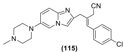
Figure 23 : Structure of 4-(4-chlorophenyl)-3-((6-(4-methylpiperazin-1-yl) H -imidazo[1,2-a]pyridin-2-yl)methyl)but-3-enitrile with anthelmintic activity
