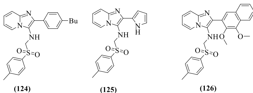
Figure 27: N-substitued- 2-aryl-imidazopyridine derivatives with antifungal activity
