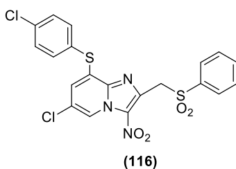
Figure 24: Structure of 6-chloro-8-((4-chlorophenyl)thio)-3-nitro-2-((phenylsulfonyl)methyl)imidazo[1,2-a]pyridine
