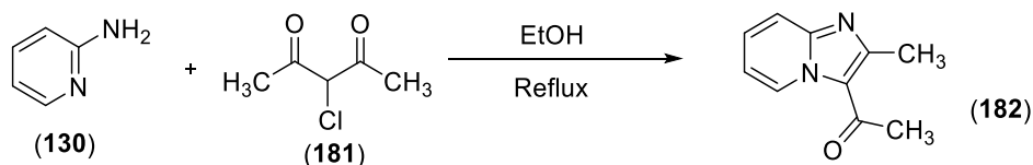
Figure 32: Synthesis method of 1-(2-methylH-imidazo[1,2-a]pyridin-3-yl)ethanone via an \alpha -chloro- \beta -diketone
