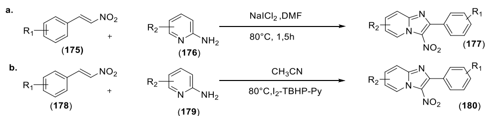
Figure 31: a.Synthesis method of 3-nitro-2-phenyl-imidazopyridine derivatives according to Prashant B. Jagadhane et al. b.Synthesis method of 3-nitro-2-phenyl-imidazopyridine derivatives according to Litao An et al.
