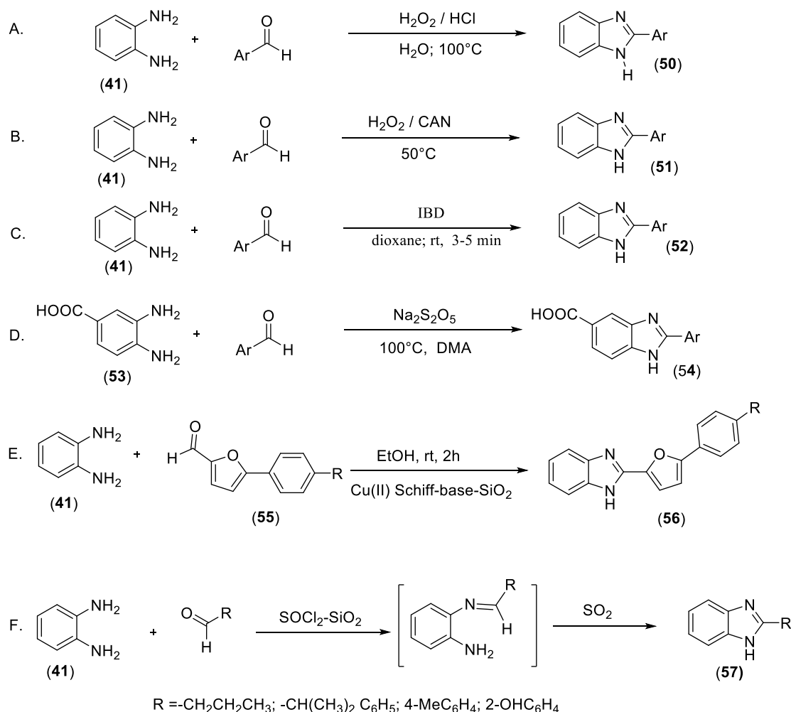
Figure 12: A. Synthesis of 2-aryl-1 H -benzimidazole according to Kiumars Bahrami et al. B. synthesis of 2-aryl-1 H -benzimidazole. C. Synthesis of the derivatives of 2-phenyl-1 H -benzimidazole according to Li-Hua Du et al. D. Synthesis of derivatives of 2-aryl-1 H -benzimidazole according to Karthikeyan et al. E. Synthesis of 2-substituted benzimidazole catalyzed by a Schiff base. F. 2-substituted benzimidazole synthesis according to Alloum et al.
