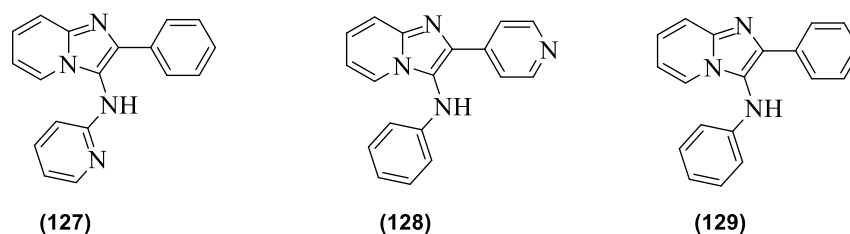
Figure 28: Imidazo[1,2-a]pyridin-3-amine derivatives with anti-inflammatory activities
