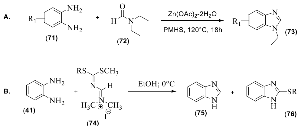
Figure 14: A. Synthesis of N-substituted benzimidazole derivatives according to Deepak Nale. B. Synthesis of benzimidazole and 2-thiobenzimidazole according to Sissouma et al
