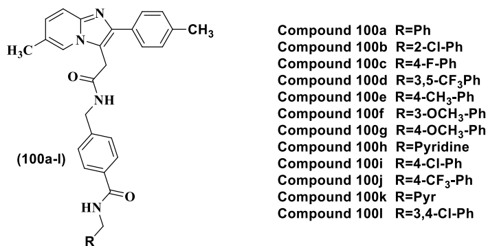
Figure 19 : Imidazo[1,2-a]pyridine derivatives by Pushpalatha Budumuru et al. against E. coli (ATCC-25922), S. aureus (ATCC-9144), K. pneumoniae (ATCC-13883) and B. subtilis (ATCC-6051)
