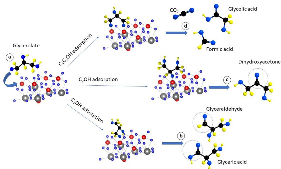
Figure 15: The scheme shows the attack of a polyol (in this specific example glycerolate) to the perovskite B-site (a) to form three of the several possible de-hydrogenated intermediates (b, c and d). It is important to notice that the glycerol molecule is completely hydrogenated in (a) but, depending on the pH of the solution the main reactant can be the de-hydrogenated specie (in this specific example the ion glycerolate). If the molecule adsorbs only through the -OH group of one of the primary carbons (b), depending on the site's properties, it will generate the corresponding aldehyde or acid (in this specific example glyceraldehyde and glyceric acid). If the molecule adsorbs only through the -OH group of one of the secondary carbons (c), it will generate a ketone (in this specific example only di-hydroxyacetone can be formed as glycerol has only one secondary carbon). Finally, if the molecule adsorbs from more than one -OH at the same time, it can promote the C-C bond breaking to generate C 2 and C 1 products. The extension of the oxidation will depend on the surface acid-basic and redox properties as discussed for the case of methanol.
