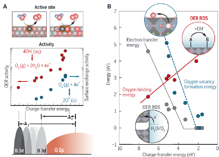
Figure 8: (A) A simplified view of the dependence of two rate-determining steps in OER, i.e., oxygen binding energy and oxygen vacancy formation as a function of the charge-transfer energy. (B) Trends in the oxygen vacancy formation, electron transfer energy, and oxygen binding energy as a function of charge-transfer energy. Adapted from ref. 150
