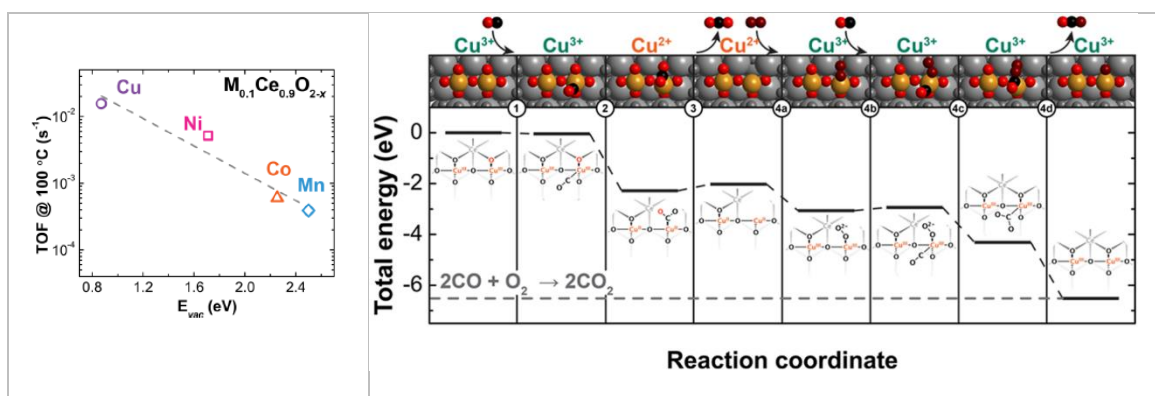
Figure 11. (Left) Correlations between computed E_{vac} and the intrinsic CO oxidation activity on M 0.1 Ce 0.9 O 2-x and (right) DFT computed reaction mechanism of CO oxidation on {111}-terminated copper substituted ceria. The total energy of the system is the sum of the energies for the slab, gas molecules and adsorbates. Image extracted from Elias et al. 170 .
