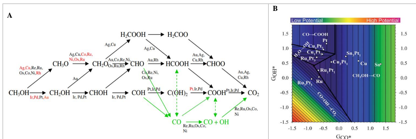
Figure 4: (A) Pathways for the MEOR on different metals and (B) volcano plot pointing the best catalyst candidates considering G OH and G CO as descriptors and the indirect mechanism found for Pt(111) surface. The green lines in (a) correspond to the indirect pathway, involving the formation of CO as intermediate. Images adapted from Ferrin et al. 38 and Rossmeisl et al. 69
