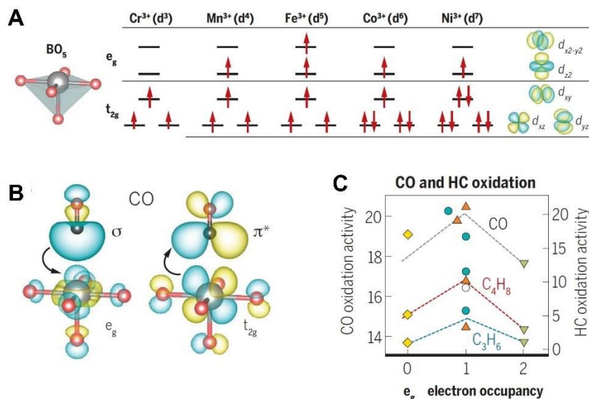
Figure 10: (A) Electronic configuration and d-orbitals for metallic cations of first-row transition metals in a BO 5 configuration. (B) CO \sigma orbital in the top left. In the right, the \pi^* orbital of CO receives electrons from the occupied perovskite t_{2g} orbital. (C) Correlation of perovskite e_g occupancy with catalytic activity for CO, propene (C 3 H 6 ), and isobutylene (C 4 H 8 ) oxidation (164,167,168) . Image adapted from Hwang et al. 143 .
