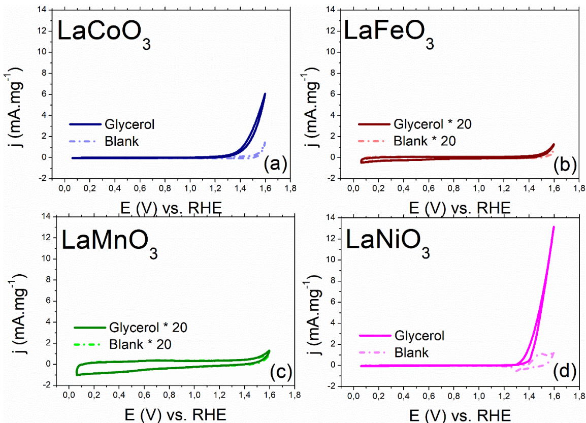
Figure 16: Cyclic voltammetry of (a) \text{LaCoO}_3 , (b) \text{LaFeO}_3 , (c) \text{LaMnO}_3 , and (d) \text{LaNiO}_3 in the presence (solid lines) and absence (dash lines) of 0.1M glycerol in 0.1M NaOH. The currents for \text{LaFeO}_3 and \text{LaMnO}_3 are multiplied by a factor of 20.
