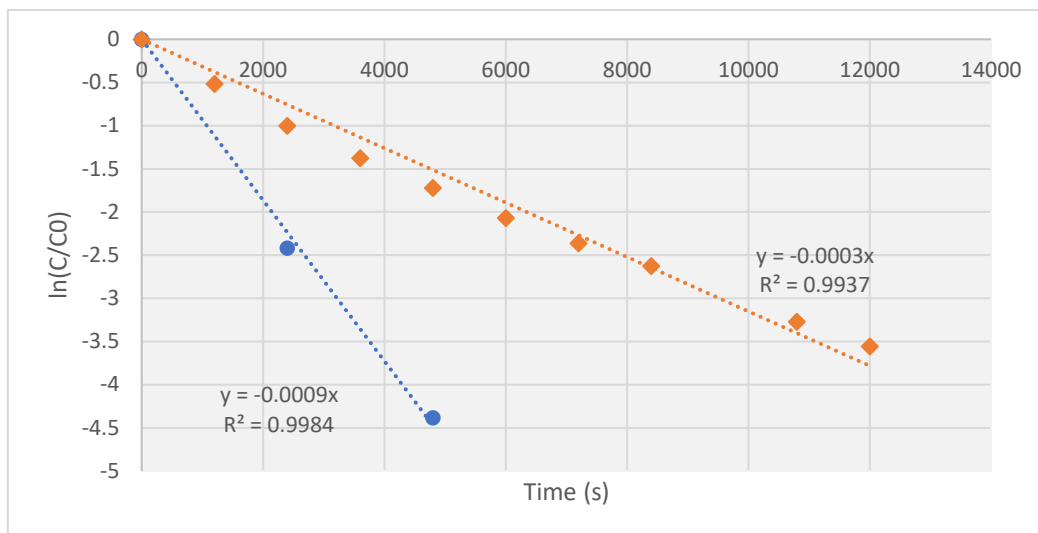
Supplementary Figure 3. Graphical determination of pseudo-first order reaction k' . \ln(C/C_0) as a function of time (seconds) for the reaction of 2-methylsulfonylpyrimidine ( 4q , 2 mM) with NACME (20 mM, blue) and GSH (20 mM, orange), at pH 7.0. C: concentration of 4q at t; C 0 : concentration of 4q at t 0 .
