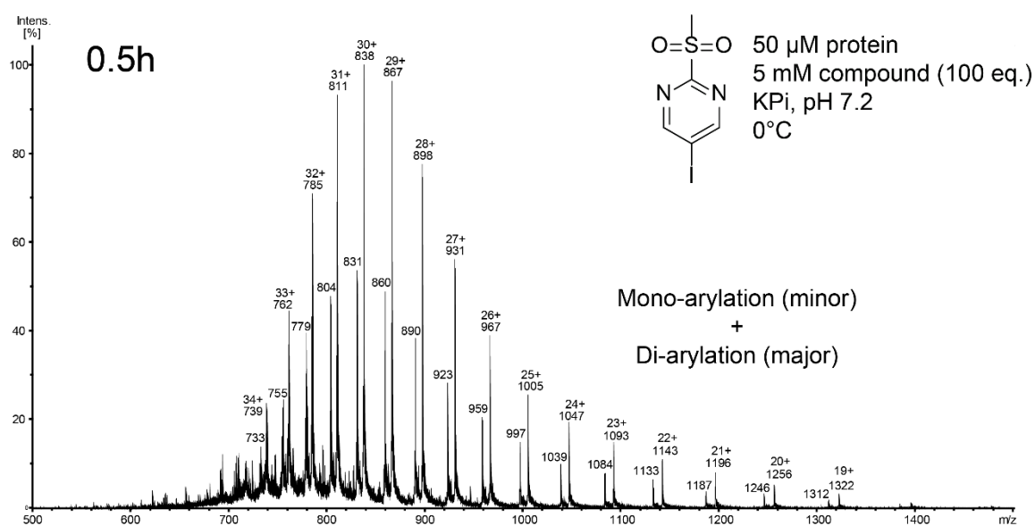
Supplementary Figure 5. Representative ESI data prior to deconvolution showing the multiple charge states of unmodified p53-Y220C (top), mono- and di-arylated p53-Y220C (bottom) following treatment with 5-iodo-2-(methylsulfonyl)pyrimidine 4u . See Figure 5A in the main text for the associated deconvoluted data.
