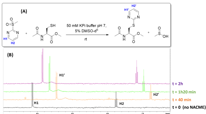
Supplementary Figure 1. (A) Reaction of 4q with NACME with pyrimidine protons assigned in both starting material and product; (B) Staggered NMR spectra of 10 equivalents NACME reacting with 4q over 2 hours in 50 mM KPi buffer, 5% v/v DMSO-d 6 , pH 7.0. Black
