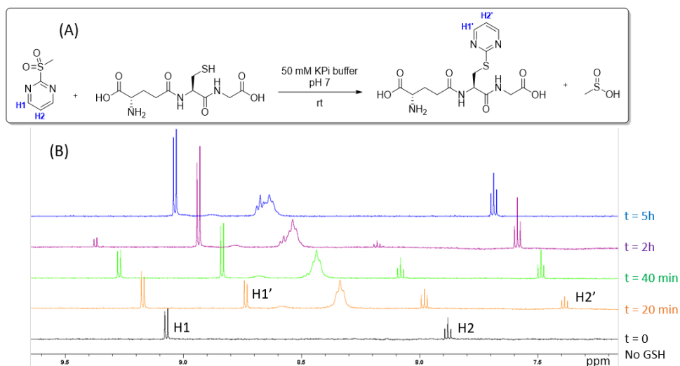
Supplementary Figure 2. (A) Reaction of 4q with GSH with pyrimidine protons assigned in both starting material and product; (B) Staggered NMR spectra of 10 equivalents GSH reacting with 4q over 5 hours in 50 mM KPi buffer, 5% v/v DMSO-d 6 , pH 7.0.
