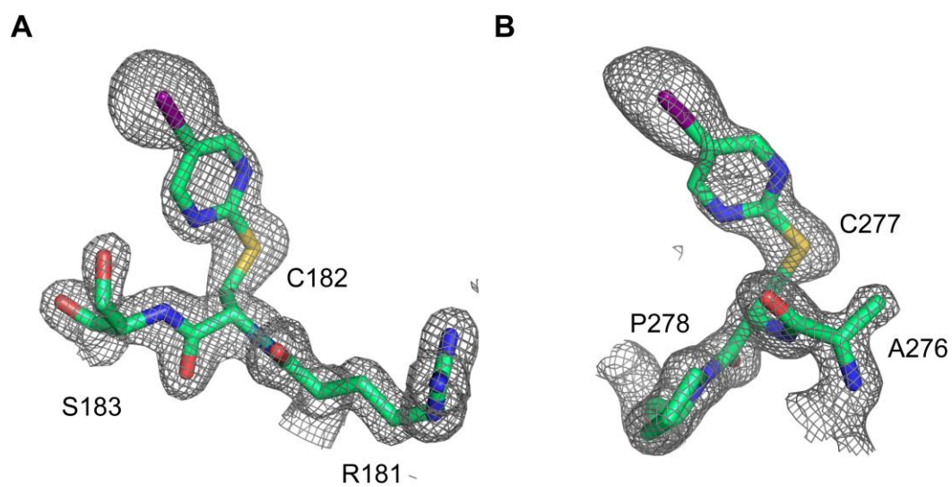
Supplementary Figure 6. Electron density at modified cysteine residues in the p53-Y220C mutant structure after treatment with compound 4u . 2Fo-Fc electron density maps are shown at a contour level of 1.3 \sigma for segments of chain B including the modified residues Cys182 (A) and Cys277 (B).
