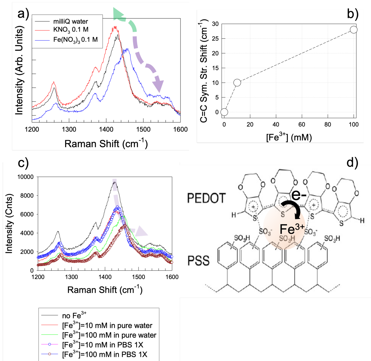
Figure 6. a) Raman spectra of PEDOT:PSS films in \text{KNO}_3 and \text{Fe}(\text{NO}_3)_3 solutions at the same concentration (100 mM); b) Shift of C=C symmetric stretching of Raman modes at 10 and 100 mM; c) Evolution of Raman spectra of PEDOT:PSS immersed in \text{Fe}^{3+} solutions in either ultrapure (milliQ) water or PBS 1X; d) Scheme of \text{Fe}^{3+} induced oxidation of the PEDOT chains.
