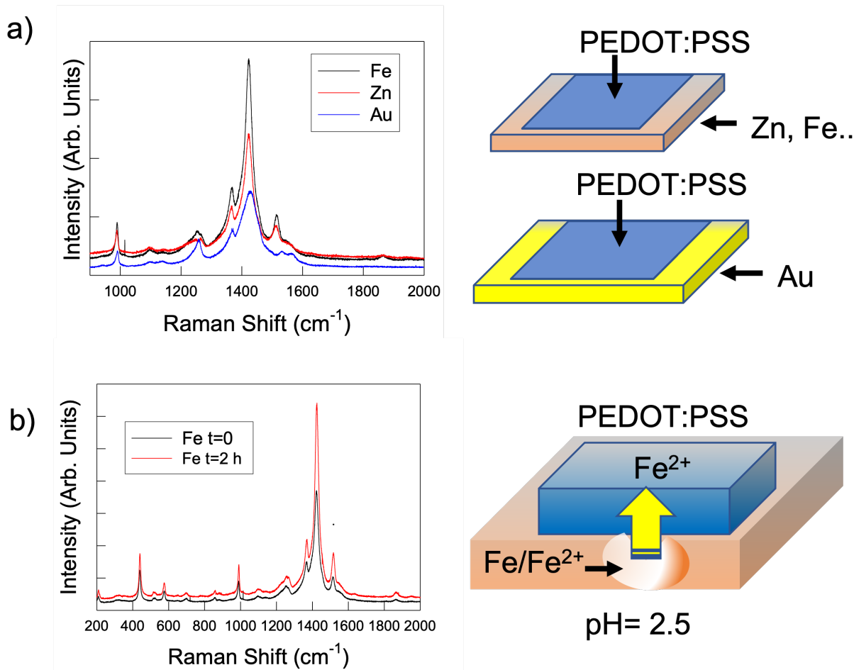
Figure 4. a) Raman spectra of PEDOT:PSS films deposited on different metals; b) Evolution of the Raman spectrum of films deposited onto Fe substrates as a function of time (see the main text for details).
