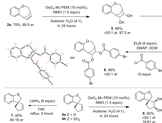
Scheme 2. Synthetic derivatizations of a) tricyclic Heck product 2a and b) spirocyclic Heck product 4a .
