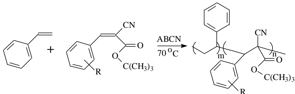
Scheme 2. Copolymerization of ST and the tert-butyl phenylcyanoacrylates, where R is 3,5-dibromo, 2,4-dichloro, 2,6-dichloro, 3,4-dichloro, 2,4-difluoro, 2,5-difluoro, 2,6-difluoro, 3,4-difluoro, 3,5-difluoro.
