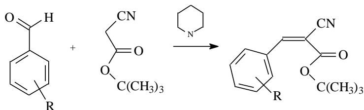
Scheme 1. Synthesis of tert-butyl phenylcyanoacrylates where R is 3,5-dibromo, 2,4-dichloro, 2,6-dichloro, 3,4-dichloro, 2,4-difluoro, 2,5-difluoro, 2,6-difluoro, 3,4-difluoro, 3,5-difluoro.
