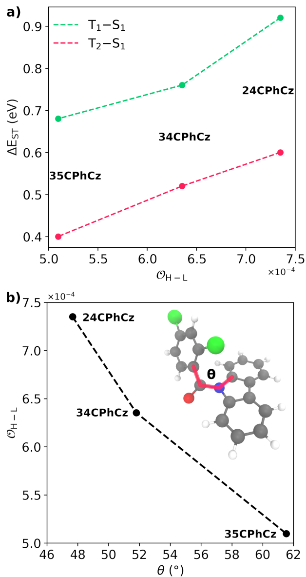
Figure 9: a) Singlet-triplet energy gap, computed in the strong coupling limit ( \Delta E_{ST} ), between S_1-T_1 (green) S_1-T_2 (pink) as a function of the HOMO-LUMO overlap ( \mathcal{O}_{H-L} , Equation 5). b) \mathcal{O}_{H-L} versus the dihedral between the planes along Cz and Ph moieties, \theta_{Cz_2NC_\alpha C_{Ph}} (shown in panel b).
