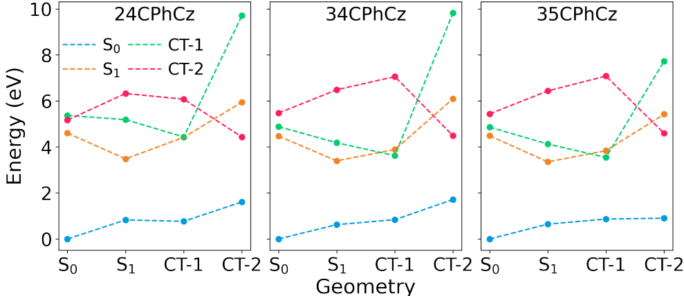
Figure 3: Energies of S_0 , S_1 , CT-1 and CT-2 states computed at the critical points of the PES in solution of DCM. The states CT-1 and CT-2 are computed using constrained DFT as explained in Section 2.
