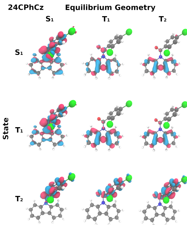
Figure 2: Transition densities of 24CPhCz with respect to the ground state. An isovalue of 0.002 is used, with negative isovalues represented in blue and positive in red.
