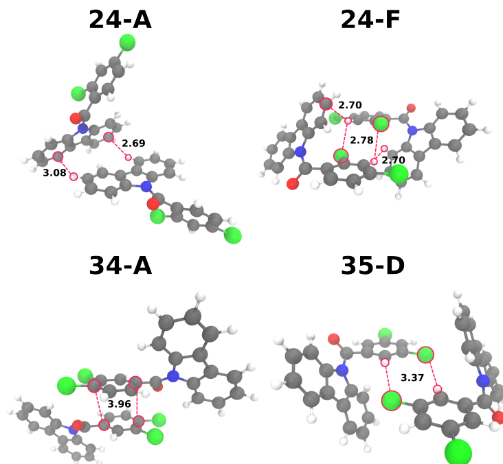
Figure 5: Dimers with higher exciton couplings for 24PhCz, 34CPhCz and 35CPhCz. Distances in Å.
