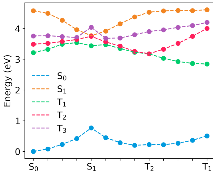
Figure 6: Linear interpolated pathway between the S_0 geometry and excited state equilibrium geometries in 24CPhCz
