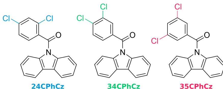
Figure 1: Dichloro derivatives of (9H-carbazol-9-yl)(phenyl)methanone investigated in this work.
