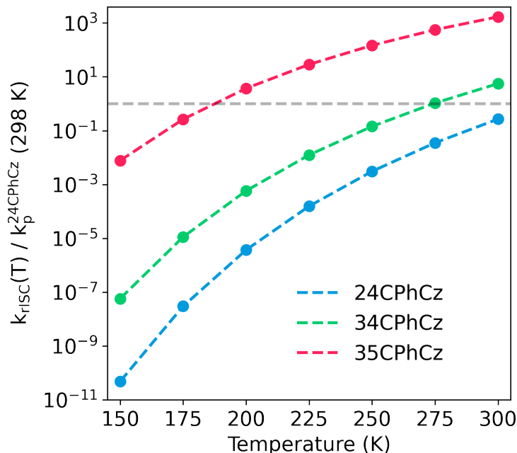
Figure 7: Temperature dependence of rISC rate constant ( k_{rISC} , computed with Eq 2). Note that k_{rISC}(T) is rescaled by using the phosphorescence rate constant ( k_p^{24CPhCz} ) of 24CPhCz determined experimentally at room temperature in ref 13.
