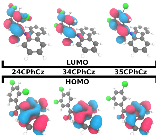
Figure 8: HOMO and LUMO orbitals for the three systems.
