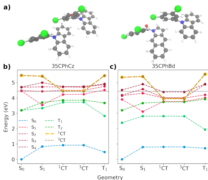
Figure 11: (a) 35-C molecular dimer for the pure (35\text{CPhCz})_2 and impurified (35\text{CPhCz}-35\text{CPhBd}) systems. (b) and (c) Energy profiles for singlet and triplet states including the 35\text{Cz}-35\text{Bd}^+ ( ^1\text{CT} and ^3\text{CT} ) states computed at the critical points for dimer 35-C embedded in the crystal environment using the OEC model. The grey line signals the energy of the S_1 FC region energy of the pure dimer.
