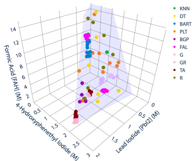
Fig. 2. Convex hull of experiments for 4-Hydroxyphenethyl amine. The blue polygon represents the stateset of all achievable concentrations due to volume and solubility limits. Points represent successful experiments predicted by different models. Models such as BART, BGP, FAL, FALGP and GRYF, are clustered together in chemical space. The exploitation recommender optimizes for experiments with the highest probability of success which tend to have similar experimental conditions to those already sampled. Each model mentioned above has two clusters of points corresponding to the initialization experiments used to train the model. These models explore a small fraction of the chemical space and cluster in different parts of the space due to the sensitivity to initialization samples
