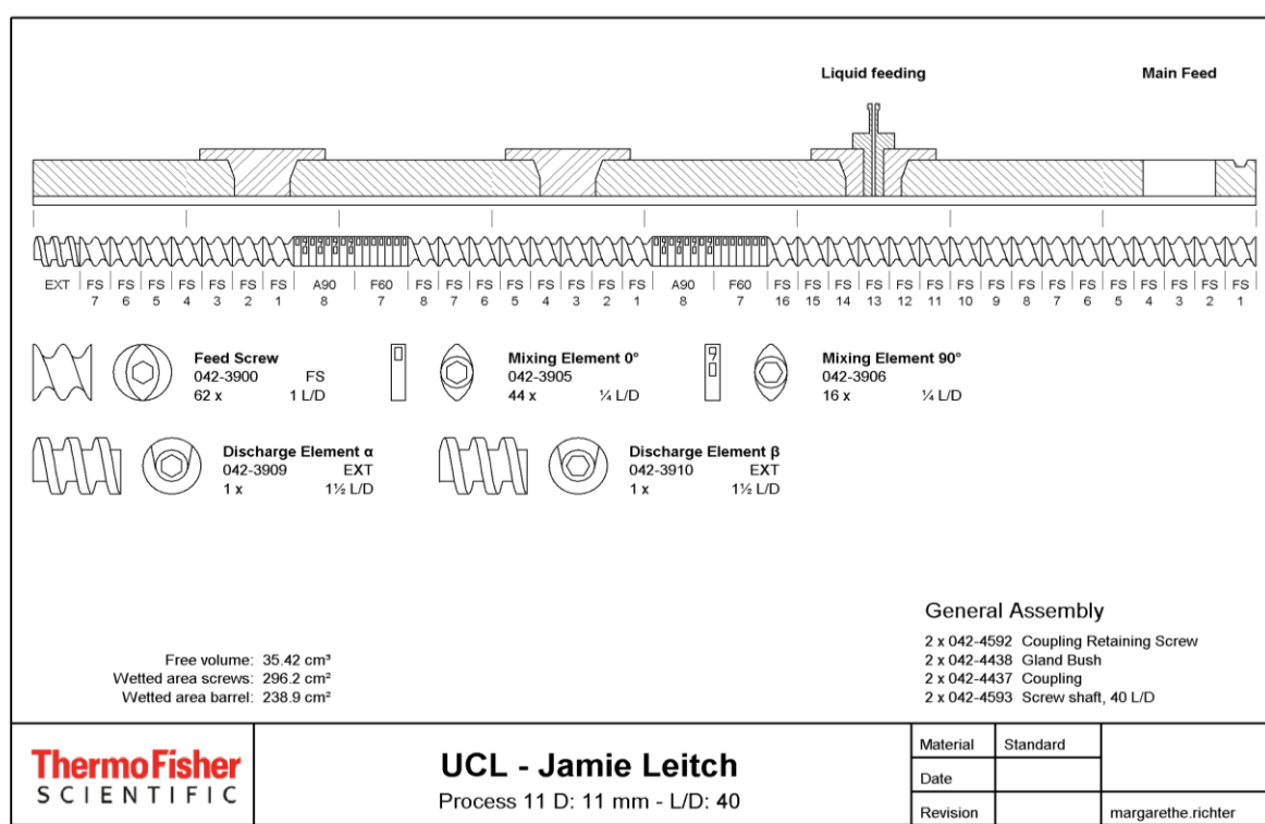
Figure S2: Screw configuration utilised in this process, provided by Thermo Fisher Scientific
