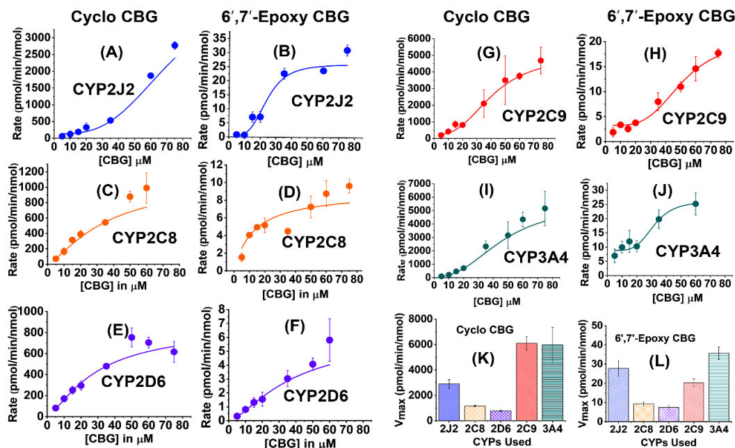
Figure 4. Metabolism of CBG in presence of CYPs: CBG metabolism leads to the formation of cyclo-CBG (7) and 6',7'-epoxy CBG (5). The kinetics of CBG metabolism are shown in the presence of CYP2J2 (blue), CYP2C8 (orange), CYP2D6 (purple), CYP2C9 (red), and CYP3A4 (green). Cyclo-CBG formation for all the CYPs are shown in (A), (C), (E), (G), (I) and 6',7'-epoxy CBG in (B), (D), (F), (H), (J). Comparison of product formation: Maximum rate ( V_{\text{max}} ) for (K) cyclo-CBG formation and 6',7'-epoxy CBG formation are shown in (K) and (L) respectively. V_{\text{max}} is represented in pmol/min/nmol of protein in both the cases. The concentration of substrate (CBG) was varied 5-75 \mu\text{M} . Data has been fitted to either Michaelis-Menten or Hill equation and error bars represent \pm SD
