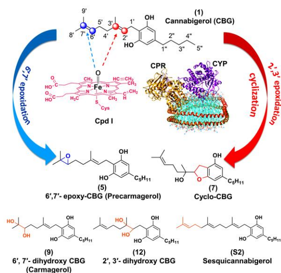
Figure 1. Schematic representation of metabolism of cannabigerol (CBG) in presence of Cytochrome P450 enzyme (CYP). Epoxidation of CBG in presence of oxo-heme complex (prosthetic group of CYP, known as compound I or Cpd I) can occur either at the 2',3' position to give (7) cyclo-CBG or at 6',7' position to give (5) 6',7'-epoxy-CBG. The sites of metabolism are shown in blue and red spheres. Along with these two, other CBG based compounds like: (9) 6',7'-dihydroxy CBG (Carmagerol); (12) 2',3'-dihydroxy CBG; and (S2) sesquicannabigerol have also been used in this work to study their anti-inflammatory properties. The protein nanodisc shown in this figure have: CYP (magenta), CPR (golden yellow) present in POPC/POPS nanodisc (cyan) which is bound by membrane scaffold protein MSPE3D1 (orange). For our study we have used CYP2J2, CYP2C8, CYP2C9, CYP2D6 and CYP3A4.
