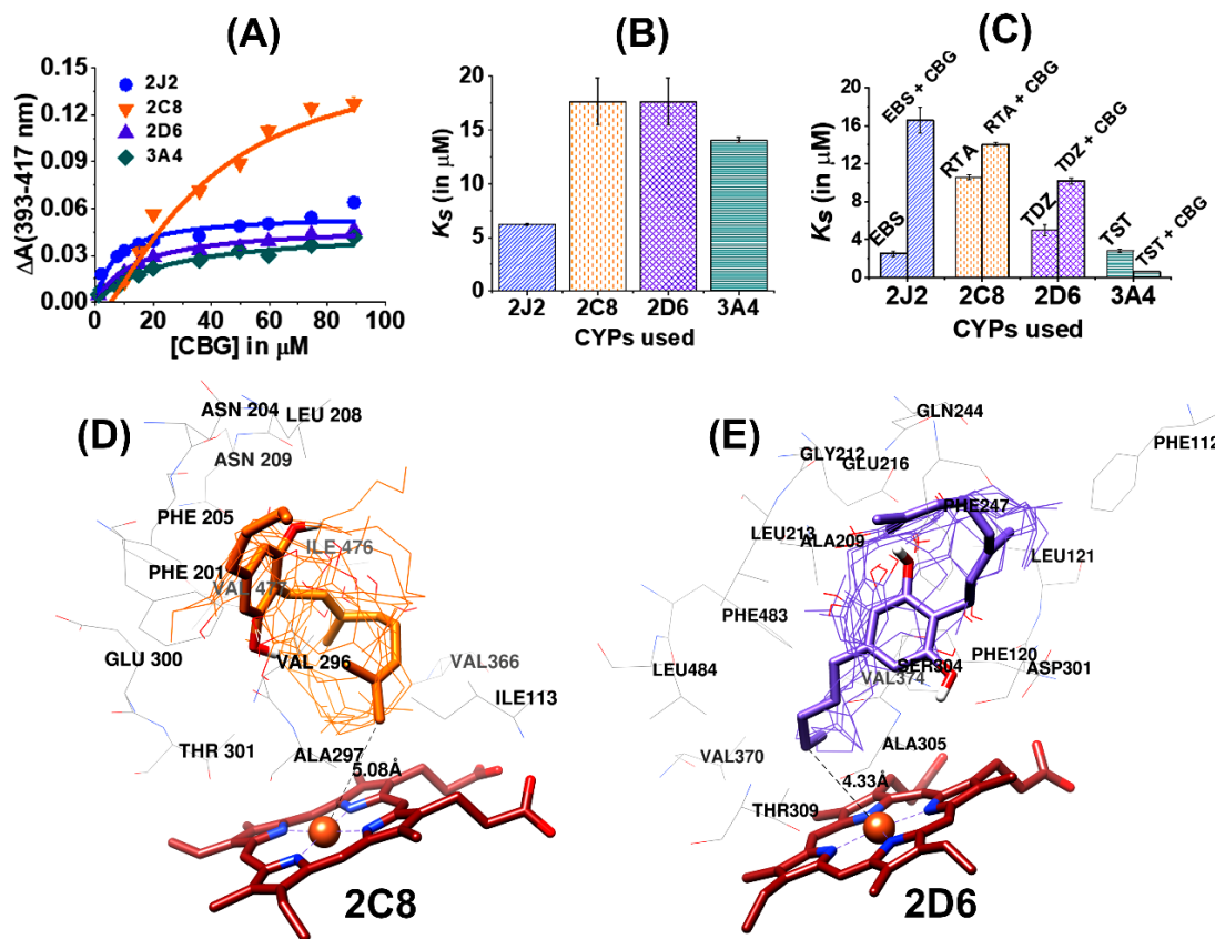
Figure 5. Binding of CBG to different CYPs. (A) Soret titration binding curves for CBG with all four CYPs. 2J2 is shown in blue circles, 2C8 in orange inverted triangles, 2D6 in purple triangles and 3A4 in green diamonds. (B) Comparison of K_s (in \mu M ) among four different CYPs. (C) Competitive binding study of ligands to different CYPs in presence and absence of CBG: Ebastine (EBS) with CYP 2J2 in the presence (EBS + CBG) and absence (EBS) of CBG; all trans -retinoic acid (RTA) with CYP 2C8 in the presence (RTA+CBG) and absence (RTA) of CBG; Thioridazine (TDZ) with CYP 2C8 in the presence (TDZ+CBG) and absence (TDZ) of CBG; Testosterone (TST) with CYP 3A4 in the presence (TST+CBG) and absence (CBG) of CBG. (G). All the binding spectra were fitted to a single binding isotherm. CBG was added incrementally from 0 to 90 \mu M . The change of absorbance ( \Delta A ) from 393 to 417 nm was calculated for each titration and plotted CBG concentration ( \mu M ). Data were fitted with Origin Lab to the single binding isotherm to determine the K_s . All experiments were done in triplicate and data were produced from the means of three repeats ( N=3 ). The error represents the standard error of the mean of three experiments. Comparison of K_s (in \mu M ) among four different CYPs in the presence and absence of CBG. Docking Study of CBG: Protein-ligand docking between (D) CYP2C8 and (E) CYP2D6 with CBG (using AutoDock Vina) and the different docked poses of CBG are shown. The docked structures closest to Fe are shown as sticks models whereas the remaining CBG structures are shown as wires. The heme moiety is shown in brown. The nearby residues that are located within a distance of 5 Å are shown in the figures. The distance from Fe to CBG molecule indicates the closest distance between protein and ligand for various CYPs.
