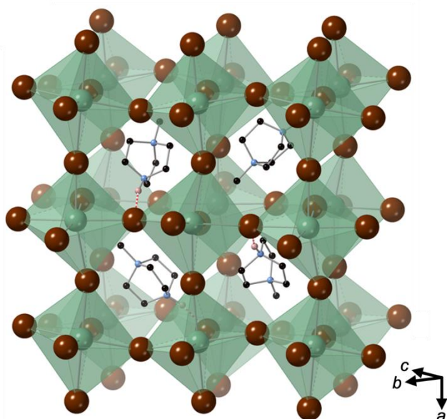
Figure 2. Extended unit cell of [MDABCO]RbBr 3 , showing the tilted orientations of four MDABCO dications within the pseudo-cubic framework of corner-sharing RbBr 6 octahedra. C, N, Rb and Br are shown in black, blue, green and brown, respectively. H atoms are omitted for clarity, apart from N–H atoms (pink) involved in hydrogen bonds, which are indicated by dashed red lines.
