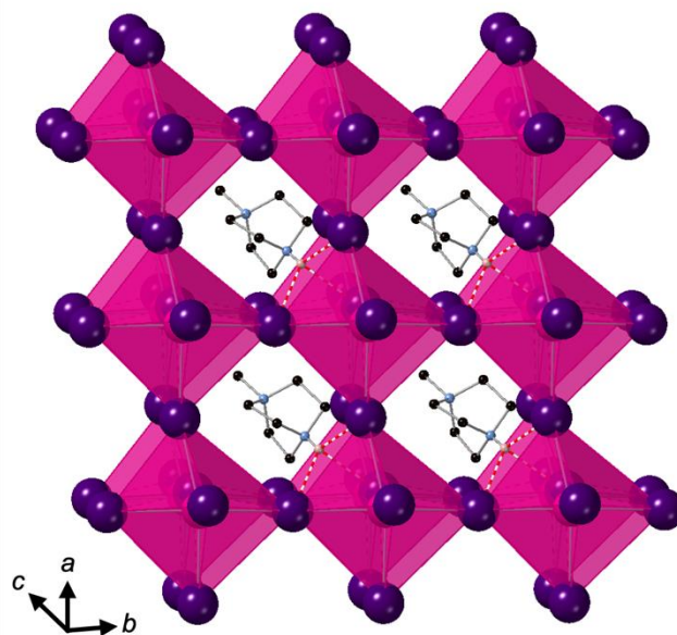
Figure 1. Four adjacent pseudo-cubic motifs of [MDABCO]CsI 3 , showing alignment of the MDABCO N–N axes along the unique axis ( c ). C, N, Cs and I are shown in black, blue, pink and purple, respectively. H atoms are omitted for clarity, apart from N–H atoms (pink) involved in hydrogen bonds, which are indicated by dashed red lines.
