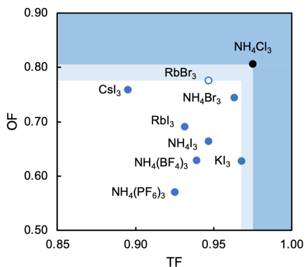
Figure 4. Phase behaviour of MDABCO-based perovskites as a function of tolerance factor (TF) and octahedral factor (OF), showing B- and X-site compositions. Blue circles are pseudo-cubic perovskites with \langle 111 \rangle MDABCO orientations. The open circle is the pseudo-cubic perovskite with \langle 110 \rangle MDABCO orientations. The black circle is the hexagonal-type structure, which defines upper limits of ranges for pseudo-cubic perovskite formation, 0.97 < TF < 0.98 and 0.78 < OF < 0.81 , shown in light blue. Darker blue shaded regions lie above of these limits.
