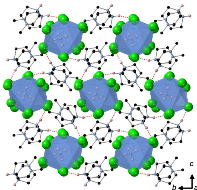
Figure 3. Crystal structure of [MDABCO]NH 4 Cl 3 containing a hexagonal array of chains of face-sharing NH 4 Cl 6 octahedra aligned along the a -axis, showing the orientations of MDABCO dications between them. C, N and Cl are shown in black, blue and green, respectively. H atoms are omitted for clarity, apart from ammonium and MDABCO N–H atoms (pink) involved in hydrogen bonds, which are indicated by dashed red lines.
