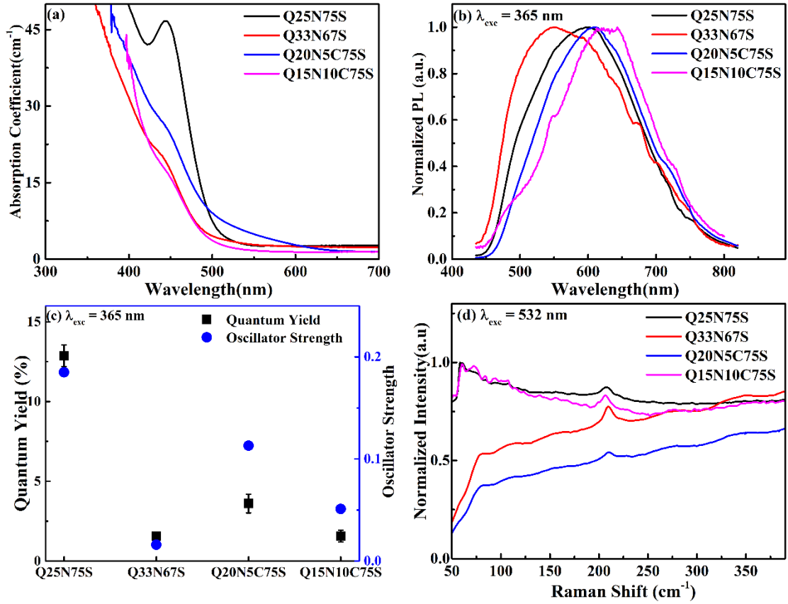
Figure 7 (a) Absorption spectra, (b) Normalized photoluminescence spectra (recorded under 365 nm excitation), (c) Quantum yield (left y-axis) and oscillator strength (right y-axis) of the lowest-energy states in our model, and (d) Raman spectra (recorded under 532 nm excitation) of Q25N75S, Q33N67S, Q20N5C75S, and Q15N10C75S glasses heat-treated at 530°C for 20 h, 480°C for 20 h, 560°C for 10 h and 580°C for 40 h, respectively. The error bar reflects the standard deviation of the measurement of PLQY. The PLQYs of the experimental fabricated glass samples are consistent with the oscillator strength as computational simulation predicted.
