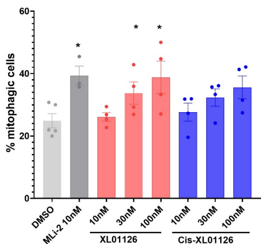
Figure 13. Effects of XL01126 and cis -XL01126 on mitophagy in Mito-QC MEFs. Quantitation of the percentage of mitophagic cells in mito-QC MEFs after 24h treatment with DMSO, MLI-2, XL01126 or cis -XL01126 at the indicated concentrations. Data are represented as mean ± SEM from 3-5 independent experiments. Statistical significance is displayed as * p < 0.05 comparing with DMSO treated sample.
