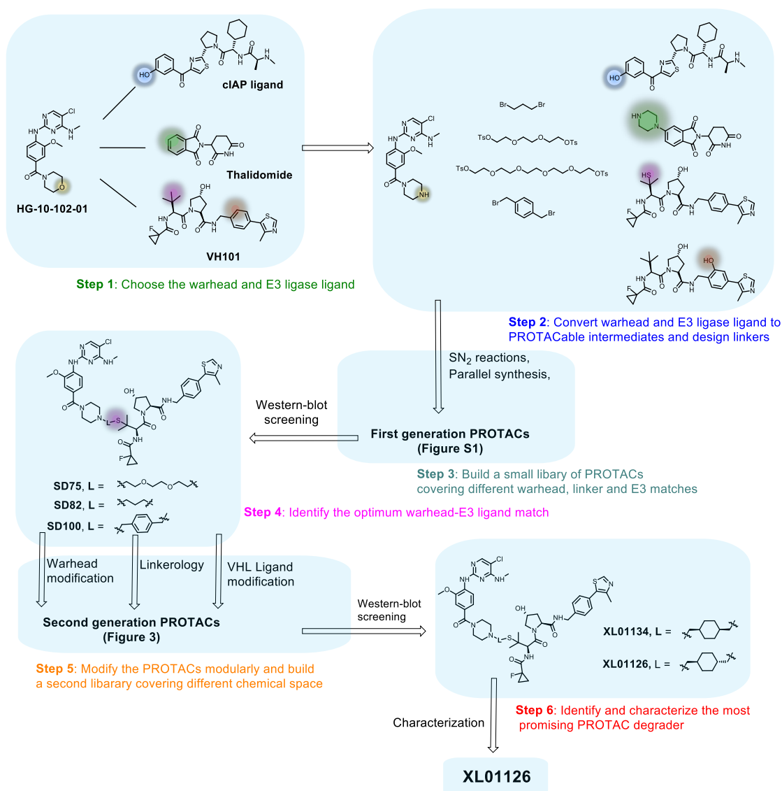
Figure 1. Our Step-by-step PROTAC discovery strategies.
