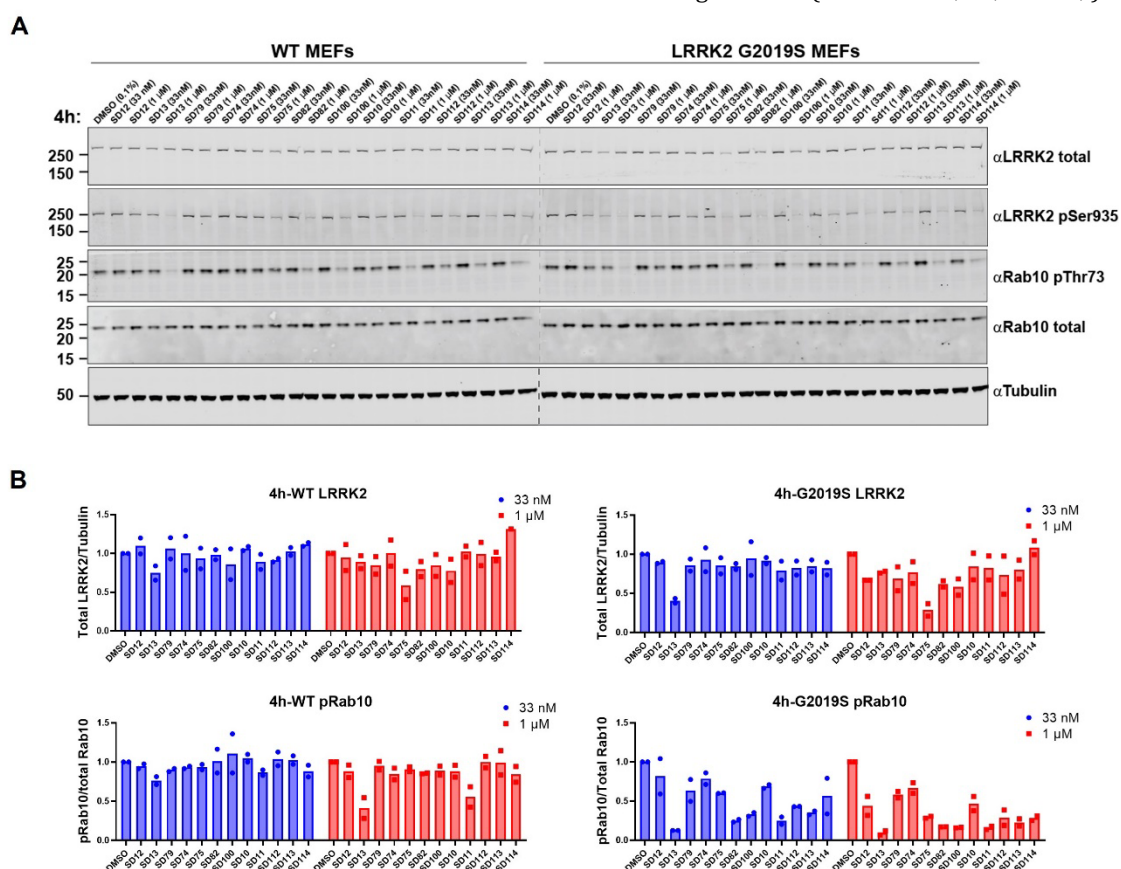
Figure 2. Screening of the first-generation PROTACs in WT and G2019S LRRK2 MEFs. (A) Representative Western blots monitoring total LRRK2, LRRK2-pSer935, Rab10-pThr73, total Rab10, and Tubulin levels following the treatment of WT and G2019S MEFs with the indicated compounds at 33 nM, 1 μM, or DMSO for 4h. (B) Quantitative analysis of the relative LRRK2 protein and Rab10-pThr73 levels, which are presented as ratios of total LRRK2/Tubulin or Rab10-pThr73/total Rab10, normalized to the DMSO treated sample. Data were obtained from two biological independent experiments.
