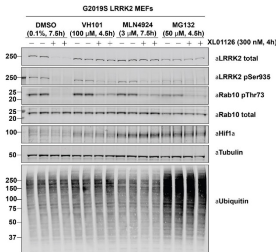
Figure 12. XL01126 induced LRRK2 degradation is rescued by VH101, MLN4924, and MG132 pre-treatment. Representative Western blots of total LRRK2, LRRK2-pSer935, pRab10, total Rab10, HIF1 \alpha , Tubulin, and Ubiquitinated protein after treating the G2019S LRRK2 MEFs with 300 nM XL01126 for 4h with or without VH101, MLN4924, and MG132 pre-treatment.
