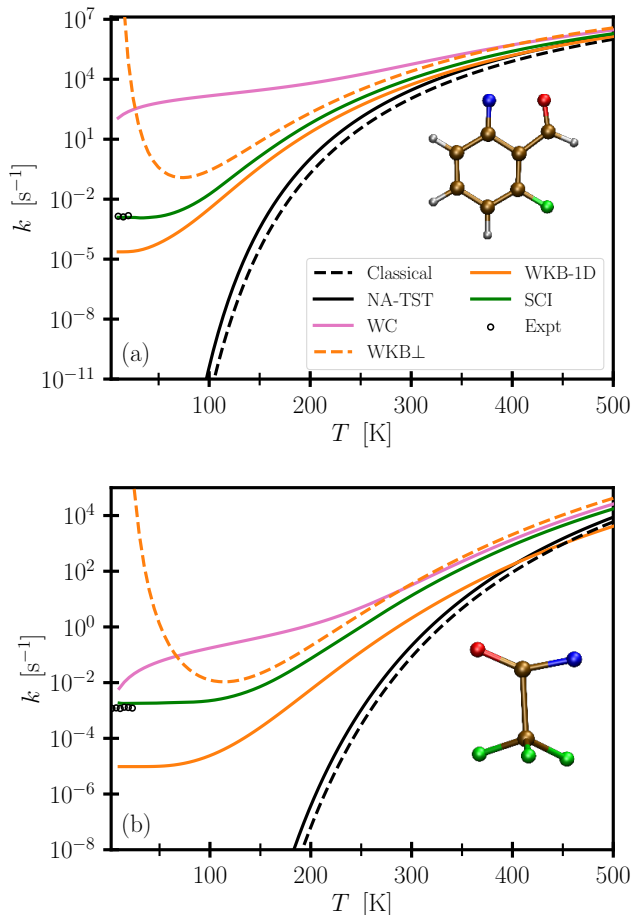
Figure 2: Reaction rates for the cyclization (top) and isomerization reaction (bottom) computed with various methods, including semi-classical golden-rule instanton theory (SCI), and compared to experiment. 42,43 All calculated rates have been corrected with the MRMP2 barrier height as described in the text; the uncorrected results can be found in the SI. The insets show the molecular structure at the MECP of the respective reaction.
