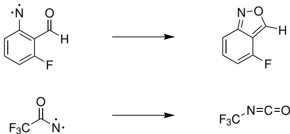
Scheme 1: Cyclization (top) and isomerization reaction (bottom).
