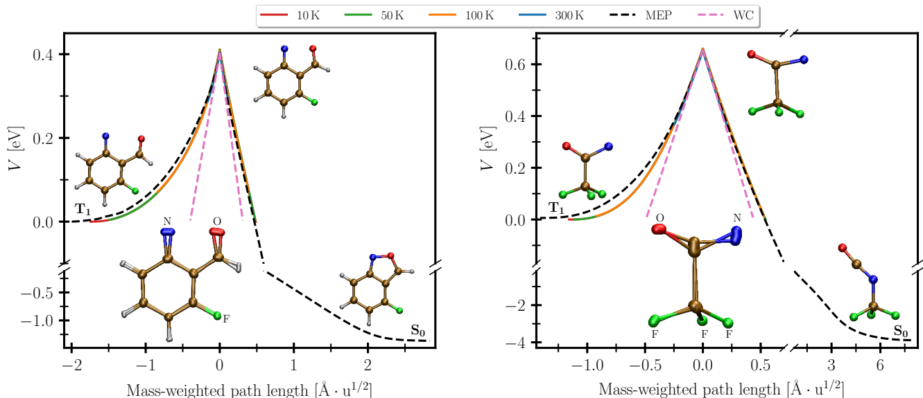
Figure 1: Potential energy computed with double-hybrid DFT along the MEPs and instanton pathways at various temperatures as well as the linear WC approximation of the PESs around the MECP for the cyclization (left) and isomerization reaction (right). The insets below the barriers depict the change in the molecular structure along the instantons in the low-temperature limit. All atoms except for the carbons and hydrogens are labelled. Bonds are drawn for the structures at the turning points of the path. The structures of the triplet and singlet minima are shown in the respective wells and the MECP structure is illustrated near the barrier top.
