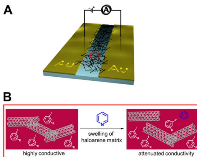
Figure 36. A) Schematic depiction of a chemiresistive sensor based on a carbon nanotube matrix between two gold electrodes. B) Incorporation of haloaryl XB selectors into the sensor matrix enables sensing of pyridine vapours by recognition-induced swelling of the matrix and an associated decrease in conductance. Reproduced with permission from Ref. 159 Copyright 2016 American Chemical Society.
