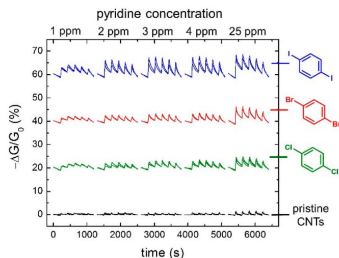
Figure 37. Conductance response of chemiresistive gas sensors containing different dihaloaryl XB selectors in the repeating presence of increasing concentrations of pyridine in N_2 carrier gas. For clarity the relative conductance responses are offset by 20%. Reproduced with permission from Ref. 159 Copyright 2016 American Chemical Society.
