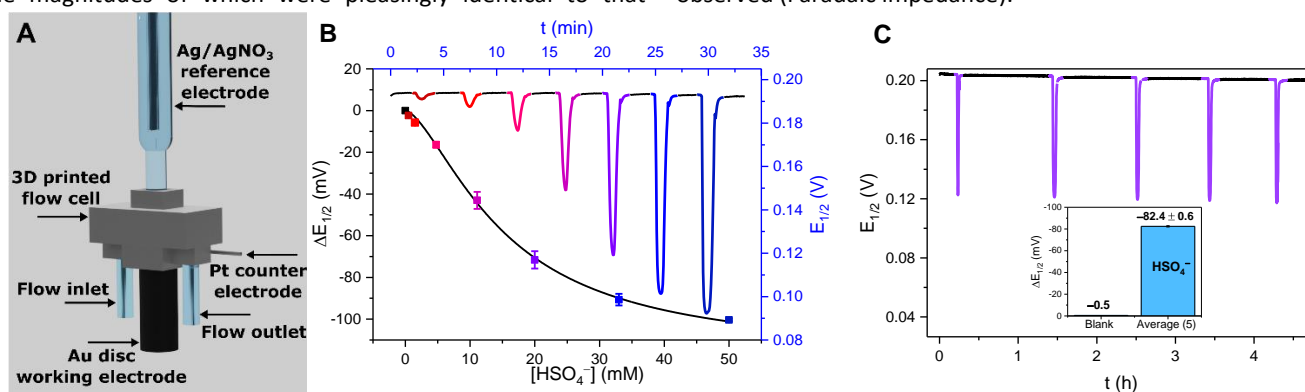
Figure 30. A) Schematic depiction of the 3D-printed electrochemical flow cell. B) Sensogram (blue axes) and corresponding isotherm (black axes) of 28.XB SAM under continuous flow to increasing concentrations of \text{HSO}_4^- in ACN/ \text{H}_2\text{O} 99:1 as measured by continuous SWV. Each spike corresponds to injections of increasing [\text{HSO}_4^-] up to 50 mM. C) Voltammetric response of 28.XB SAM towards five additions of \text{HSO}_4^- under continuous electrolyte flow over 4.5 h. Each spike represents the response towards aliquots of 20 mM \text{HSO}_4^- . The inset shows the voltammetric shift in response to the blank electrolyte and the average of all five \text{HSO}_4^- additions. Reproduced from ref. 61 under the terms of the CC BY license.
