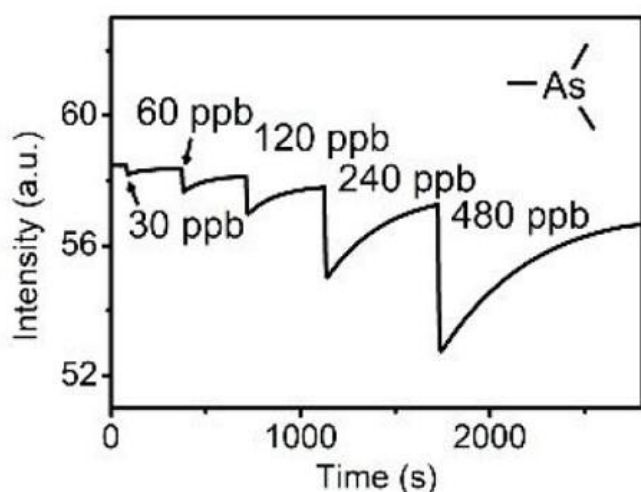
Figure 19. Fluorescence emission intensity of bundled nanoribbons of 16.ChB upon exposure of increasing concentration of trimethyl arsine gas. Reproduced with permission from Ref. 120 Copyright 2021 American Chemical Society.
