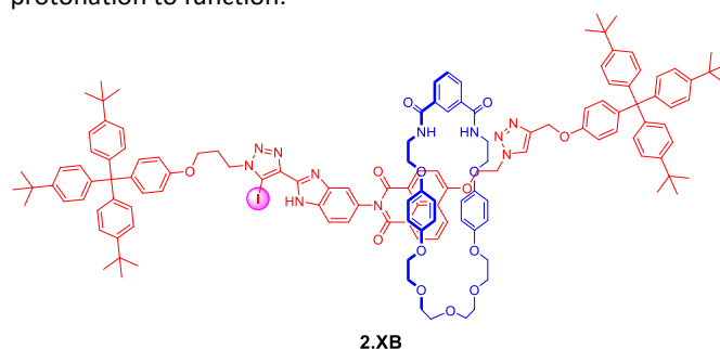
Figure 7. XB [2]rotaxane molecular shuttle 2.XB for colorimetric anion sensing in CHCl 3 . Only in the presence of a coordinating Cl - anion as well as acid-induced protonation of the benzimidazole does the macrocycle shuttle towards the XB anion binding site, resulting in a disruption of the hydroquinone-NDI charge-transfer interaction and a concomitant loss of colour.
