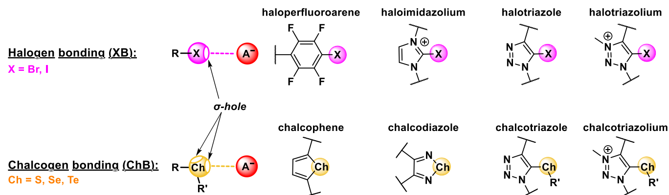
Figure 2. Schematic depiction of halogen (XB) and chalcogen bonding (ChB) interactions with an anion as archetypical Lewis base. Shown are also commonly employed XB and ChB donor motifs.
