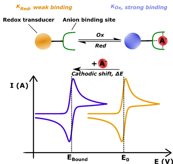
Figure 20. Schematic depiction of voltammetric anion sensing at a redox active anion receptor. Receptor oxidation/reduction is reflected in binding enhancement/decrease. In the presence of a binding anion the half-wave potential is perturbed cathodically, whereby the shift magnitude is directly proportional to the ratio of anion binding constants to the different receptor oxidation states: \Delta E \propto K_{Ox}/K_{Red} .
