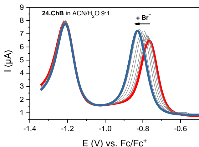
Figure 27. SWVs of telluroviologen ChB sensor 24.ChB in ACN/ \text{H}_2\text{O} 9:1 upon addition of up to 50 mM \text{Br}^- . Only the first reductive couple is responsive, indicative of complete ChB deactivation upon mono-reduction. Reproduced from Ref. 63 under the terms of the CC BY license.
