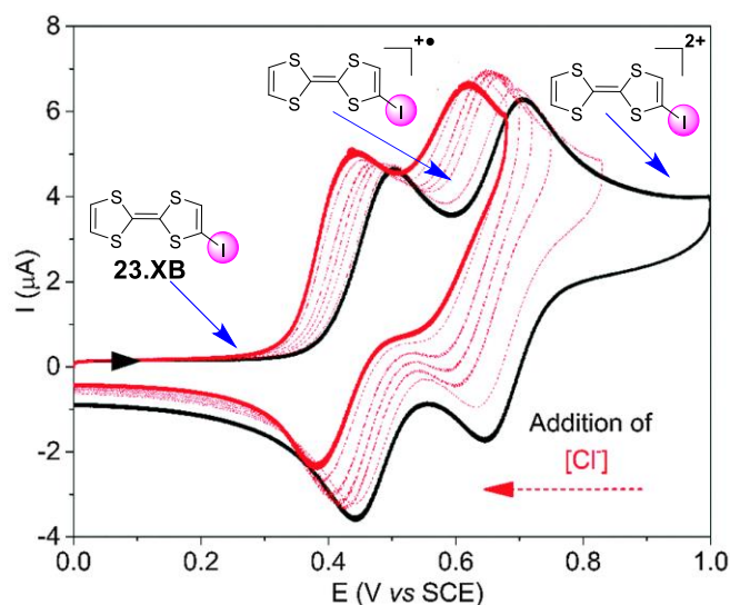
Figure 24. Chemical structure of iodo-TTF 23.XB and its corresponding CV in DMF in the absence (black) and presence (red) of increasing concentrations of \text{Cl}^- . Depicted are also the different redox states at different potentials (structures and blue arrows). Adapted from Ref. 126 with permission from the PCCP Owner Societies.
