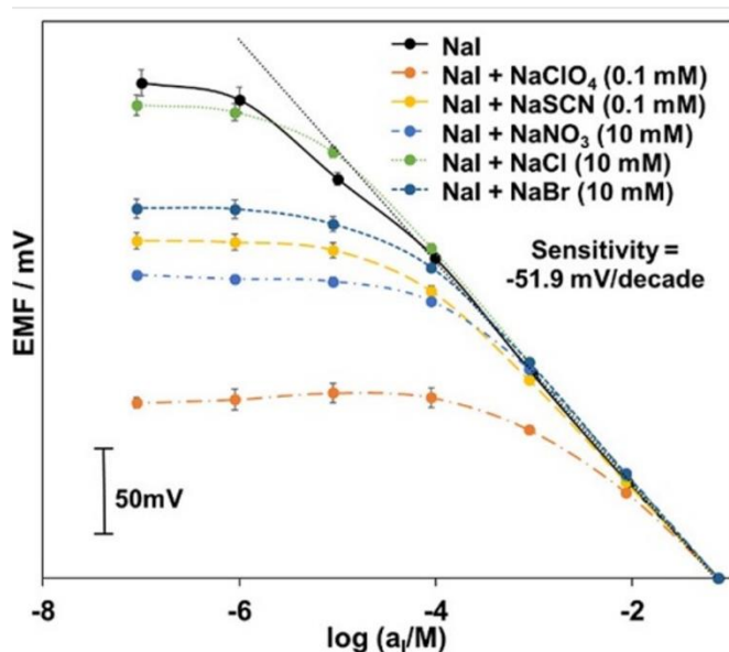
Figure 35. Response of an ISE containing ionophore 30.XB toward iodide in the absence of presence of competing anions. Reproduced with permission from Ref. 154 Copyright 2021 American Chemical Society.
