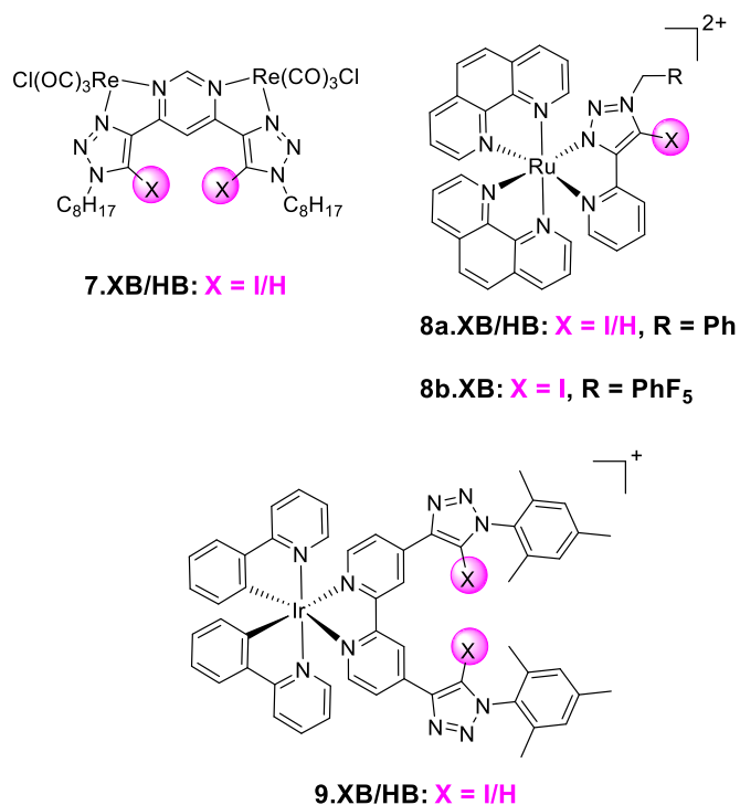
Figure 12. Chemical structures of acyclic transition metal-containing luminescent XB anion receptors.
