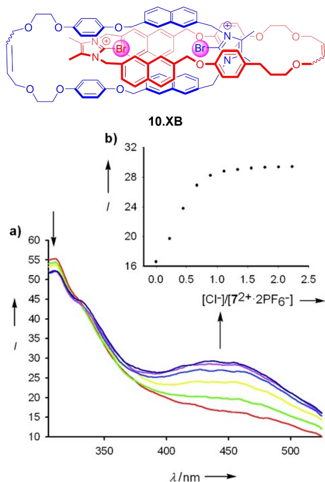
Figure 13. All-XB bromo-imidazolium-naphthalene catenane 10.XB for fluorescent halide sensing. A) Emission spectra of 10 \mu\text{M} 10.XB upon addition of \text{Cl}^- in ACN. B) The corresponding response isotherm at 445 nm. Reproduced with permission from ref. 111 Copyright 2011 Wiley.
