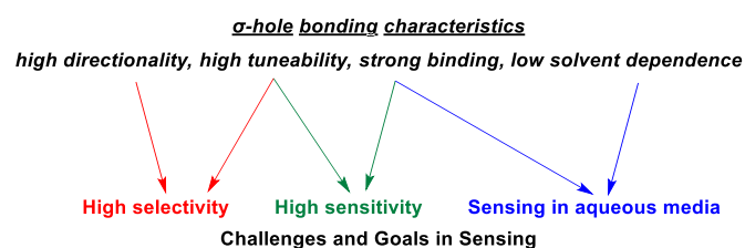
Figure 3. Important \sigma -hole bonding characteristics and their impact on relevant challenges and goals in sensor development.
