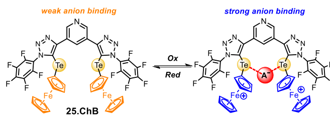
Figure 26. ChB-mediated voltammetric anion sensing was very recently achieved for the first time as demonstrated for both reductive switch-OFF of ChB in telluroviologen 24.ChB as well as oxidative switch-ON of ChB in pyridine bis(ferrocenyltelluroviologen) 25.ChB .
