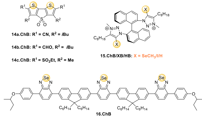
Figure 17. ChB fluorescent anion sensors.
