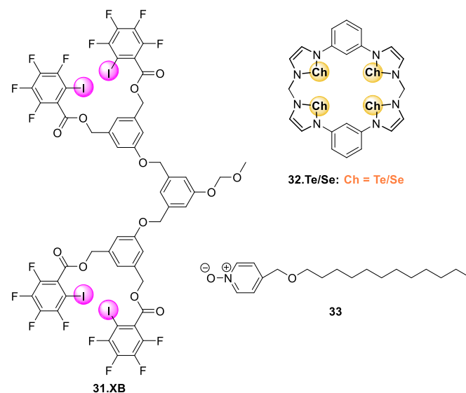
Figure 38. Chemical structures of XB organogelator 31.XB , a visual Cl^- sensor by anion induced gel-sol transition and ChB quasi-calix[4]-chalcogenadiazole host 32.Te/Se which upon interaction with surfactant 33 form supramolecular fibres or vesicles in water, respectively. Cl^- or Br^- induced disassembly of 32.Te-33 vesicles, releases the fluorescent doxorubicin cargo, presenting a stimuli-responsive drug carrier and indirect optical halide sensor.
