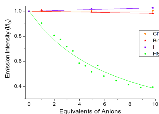
Figure 11. Fluorescence emission intensity response of 10 \mu\text{M} hydrosulfide-selective coumarin-containing 6.XB in the presence of 10 equiv. of various anions in 10 mM HEPES buffer (pH = 7.4). Reproduced from Ref. 91 under the terms of the CC BY license.
