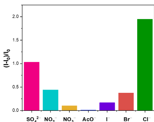
Figure 10. Relative emission intensity increase of 10 \mu\text{M} tetraphenylethene AIE anion sensor 5.XB in the presence of 10 equiv. of various anions in THF. Reproduced from Ref. 90 under the terms of the CC BY license.
