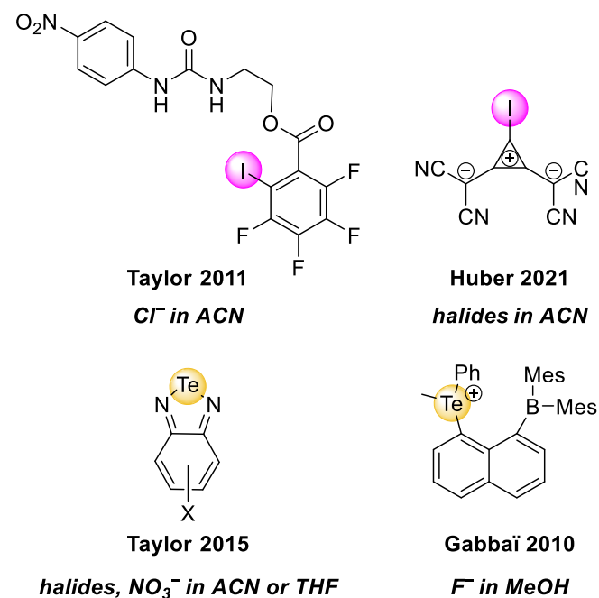
Figure 5. Selected examples of XB and ChB receptors that undergo changes in UV-vis absorbance upon exposure to the highlighted anions.
