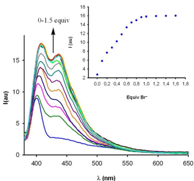
Figure 9. Fluorescence emission response of macrocyclic iodo-imidazolium host 3c.XB ( 10 \mu\text{M} ) in \text{CH}_3\text{OH}/\text{H}_2\text{O} 9:1 in the presence of increasing concentrations of bromide. Reproduced with permission from ref. 82 Copyright 2012 American Chemical Society.
