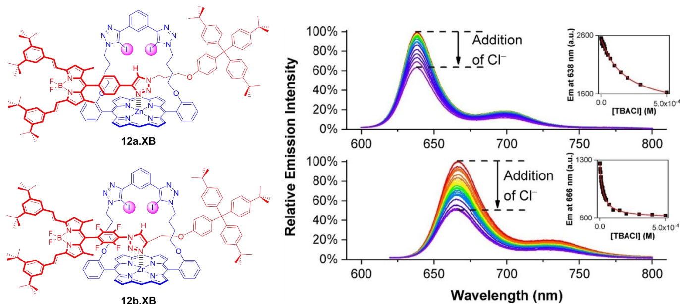
Figure 15. Fluorescence response of 1 \mu M XB BODIPY-containing strapped porphyrin rotaxanes 12a.XB (top) and 12b.XB (bottom) towards Cl - in acetone. The insets show the corresponding response isotherms, highlighting stronger binding and a larger response for the more polarised, perfluorobenzene-containing 12b.XB . Reproduced from Ref. 69 under the terms of the CC BY license.
