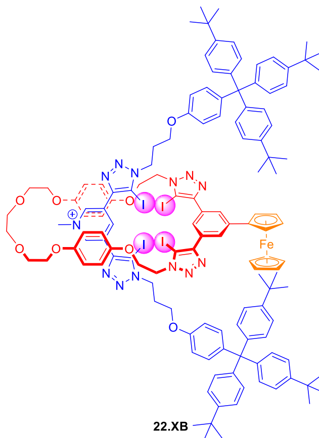
Figure 23. Ferrocene-containing all XB [2]rotaxane for selective voltammetric sensing of bromide in ACN/acetone/H 2 O 45:45:1.
