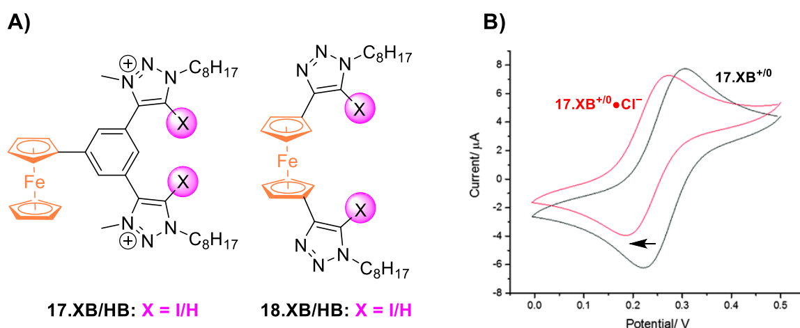
Figure 21. A) Chemical structures of first XB ferrocenyl voltammetric anion sensors. B) CVs of 17.XB in ACN in the absence (black) and presence of 10 equiv. Cl - (red). Adapted from Ref. 129 with permission from the Royal Society of Chemistry.
