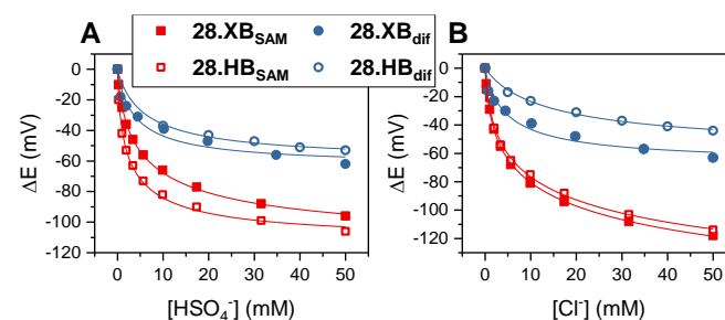
Figure 29. Comparison of cathodic voltammetric shifts under diffusive conditions of 28.XB/HB diff (blue circles) and on the surface ( 28.XB/HB SAM (red squares)) in ACN/ \text{H}_2\text{O} 99:1 upon titration with A) \text{HSO}_4^- and B) \text{Cl}^- . Filled symbol represent the XB receptors while empty symbols represent the HB receptors. Solid lines represent fits to a 1:1 host-guest Nernst model. A pronounced surface enhancement was also observed for all other tested anions ( \text{Br}^- , \text{H}_2\text{PO}_4^- and \text{NO}_3^- ). Adapted from Ref. 125 with permission from the Royal Society of Chemistry.
