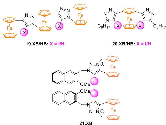
Figure 22. Chemical structures of Fc-based XB and HB voltammetric sensors for oxoanions, azide and chiral anions.
