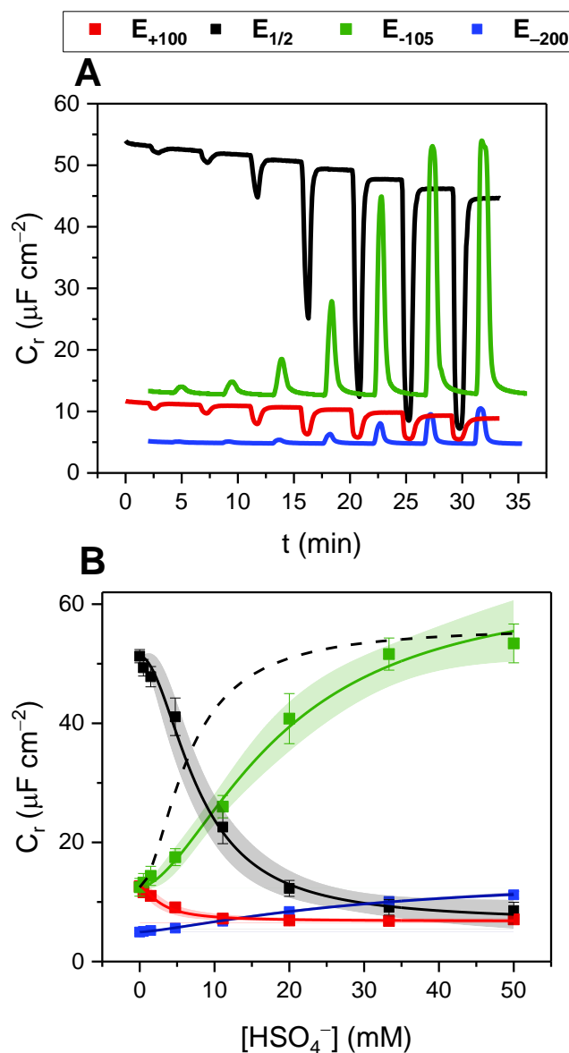
Figure 32. A) Redox capacitance response of 28.XB SAM towards \text{HSO}_4^- at E_{1/2} (black), E_{-105} (green), E_{-200} (blue) and E_{+100} (red) under continuous electrolyte flow in a custom 3D-printed flow cell (see Figure 31A). Each spike in A) represents the response towards aliquots of \text{HSO}_4^- of increasing concentrations with absolute signal increasing or decreasing depending on the initial surface polarisation. B) The corresponding baseline-corrected response isotherms. Solid and dashed lines represent fits according to the Langmuir-Freundlich model. The dashed black line represents, for simpler comparison, the mirrored capacitance response at E_{1/2} , highlighting the steeper response slope and enhanced anion binding magnitude at E_{1/2} vs. at E_{-105} . Reproduced with permission from ref. 60 Copyright 2021 American Chemical Society.
