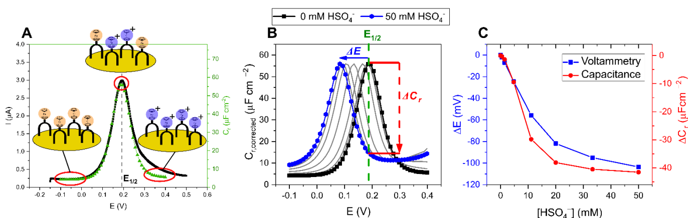
Figure 31. A) Comparison of SWV (black) and redox capacitance C_r (green triangles) as a function of electrode potential (i.e. redox density of states (DOS)) of 28.XB SAM in ACN/ \text{H}_2\text{O} 99:1. Schematically depicted is the ratio of oxidised and reduced anion receptors at different potential regimes whereby ferrocene/ferrocenium units are shown in orange and blue, respectively. B) Normalised redox capacitance C_r as a function of potential (the film density of states, DOS) in response to increasing concentrations of \text{HSO}_4^- . The blue arrow indicates the “standard” potential shift as typically resolved voltammetrically. The dashed red arrow indicates the drop in C_r at E_{1/2} (dotted black line). C) Comparison of voltammetric (blue) and redox capacitive response isotherms at E_{1/2} (red). The C_r response is steeper due to a self-amplification effect. Reproduced with permission from ref. 60 Copyright 2021 American Chemical Society.
