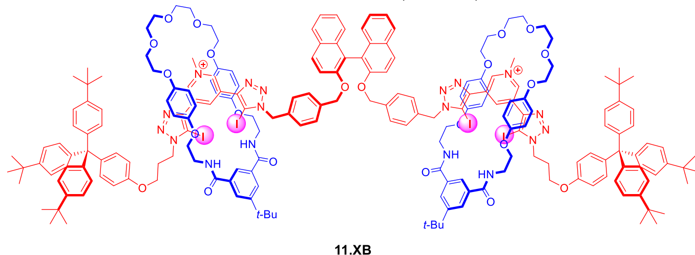
Figure 14. S-BINOL-based fluorescent [3]rotaxane 11.XB for fluorescent discrimination of S/R -glutamate enantiomers and fumarate/maleate geometric dicarboxylate isomers in \text{CHCl}_3/\text{MeOH}/\text{H}_2\text{O} 60:39:1.
