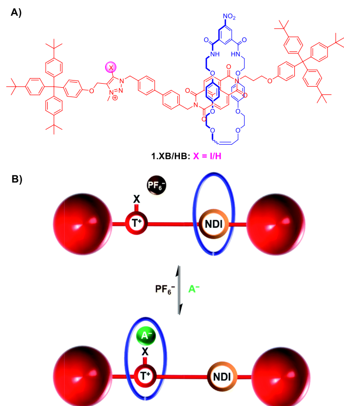
Figure 6. A) Chemical structure of bistable (iodo)triazolium-NDI [2]rotaxanes 1.XB/HB . B) Schematic depiction of anion recognition-induced shuttling of the macrocycle from the NDI to the triazolium, resulting in a naked-eye colour change from orange to colourless due to disruption of the donor-acceptor charge-transfer interactions between the hydroquinone-containing macrocycle and the NDI station. Reproduced from Ref. 80 with permission from the Royal Society of Chemistry.
