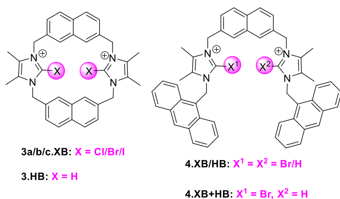
Figure 8. (Halo)imidazolium hosts for fluorescent anion sensing.
