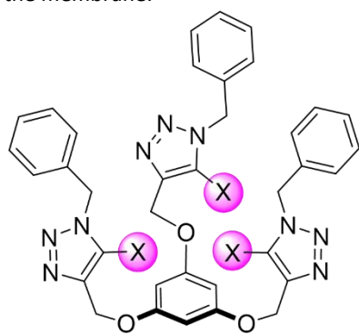
30.XB/HB: X = I/H
