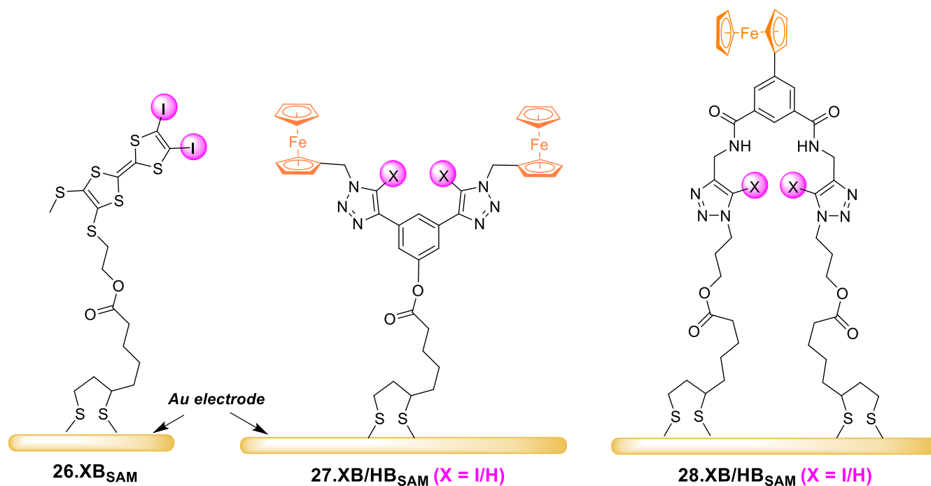
Figure 28. Schematic depiction of recently developed XB redox active self-assembled monolayers on gold electrodes. Note that for comparative solution-phase studies chemically related derivatives of 27.XB/HB and 28.XB/HB were also studied under diffusive conditions.
