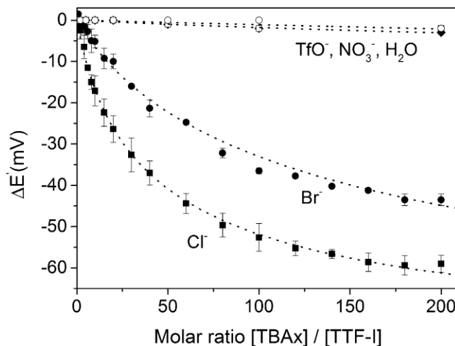
Figure 25. Cathodic voltammetric perturbations of the first oxidative couple of iodo-TTF 23.XB in DMF upon addition of various anions. Dotted lines represent fits according to a 1:1 host-guest stoichiometric Nernst binding model from which absolute anion binding constants to the various receptor oxidation states were obtained. Reproduced from Ref. 126 with permission from the PCCP Owner Societies.
