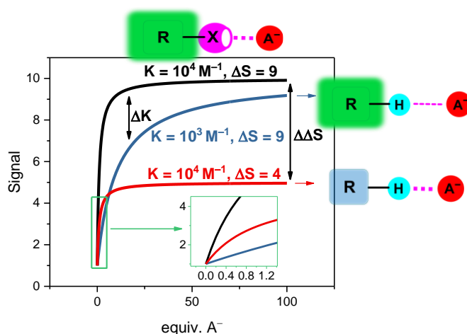
Figure 4. Simulated response isotherms of a generic non-covalent host-guest sensor based on the reporter group approach. The binding isotherms are simulated according to a simple 1:1 host-guest stoichiometric binding model with [\text{H}] = 100 \mu\text{M} and an initial free host signal of S_{\text{H}} = 1 . 59 Depicted are three exemplary cases: Black line: Strong binding ( K = 10^4 \text{M}^{-1} ) and a large signal change of the host-guest complex ( S_{\text{HG}} = 10 , \Delta S = 9 ) as typically encountered in sigma-hole based sensors. The blue and red lines represent typical examples of less potent HB sensors in which either binding is weaker (blue line, K = 10^3 \text{M}^{-1} ) or in which the signal magnitude is smaller (red line, S_{\text{HG}} = 5 , \Delta S = 4 ). This highlights the different mechanisms by which sigma-hole based sensors typically outperform related HB analogues in terms of sensitivity. Inset: magnification at low guest concentrations.
