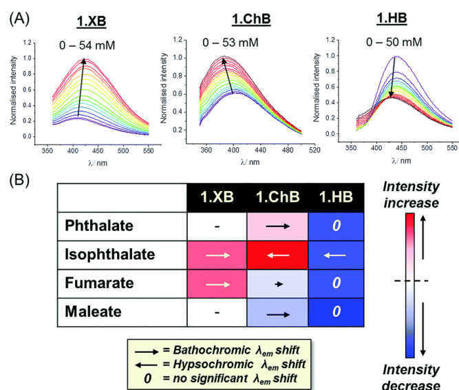
Figure 18. A) Fluorescence emission spectra of 15.ChB/XB/HB (labelled 1.ChB/XB/HB in the figure) in the presence of increasing concentrations of isophthalate in acetone/H 2 O 85:15. B) Summary of fluorescence response patterns of each receptor towards geometric dicarboxylate isomers. The length of the arrows is indicative of the magnitude of the shift in \lambda_{max} while the shade of red/blue denotes the magnitude of fluorescence enhancement/quenching. Reproduced from Ref. 119 with permission from the Royal Society of Chemistry.
