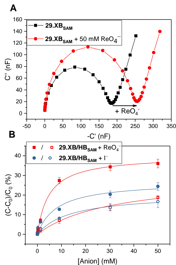
Figure 34. A) Capacitive Nyquist plots of 29.XB SAM in the absence and presence of 50 mM \text{ReO}_4^- showing an increased capacitance in the presence of bound anion. Measurements were performed at open-circuit potential ( \approx 0 \text{ V} ). B) Relative capacitive sensor response of 29.XB SAM (filled symbols) and 29.HB SAM (empty symbols) in response to \text{ReO}_4^- (red) and \text{I}^- (blue). Solid lines represent fits according to the Langmuir model. Reproduced from Ref 150 with permission of the Royal Society of Chemistry.
