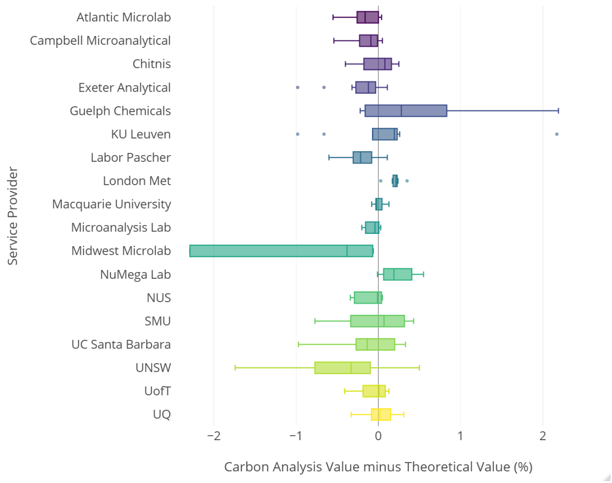
Figure 4. Box plots of observed differences between analysis and theoretical values for C, for all service providers in this study, with the C outlier from Midwest Micro Analytical Labs not shown).
