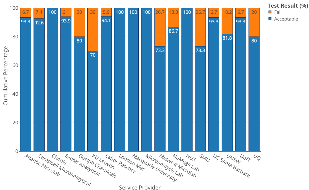
Figure 3. Percentages of “Acceptable” and “Fail” results for each of the 18 service providers used, across all 5 compounds for C, H, and N.
