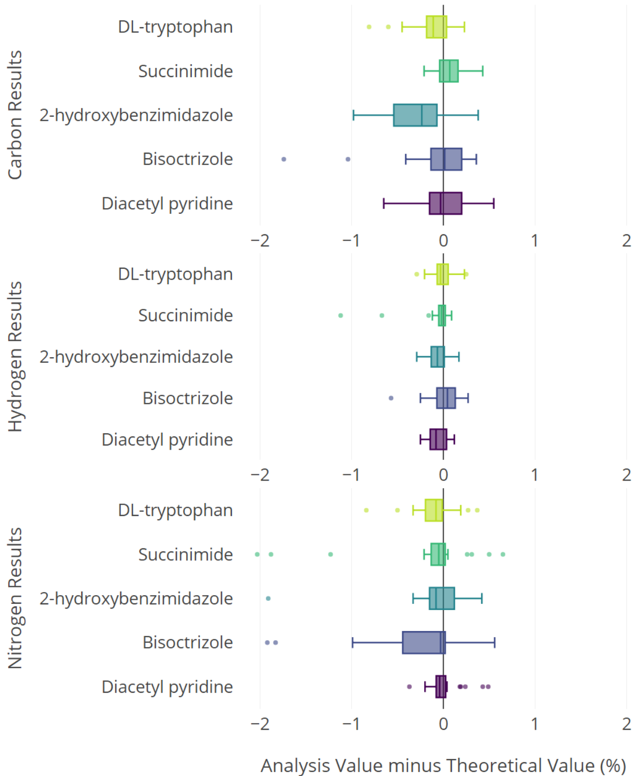
Figure 2. Box Plots of differences between analysis and theoretical values for each element, across the five different compounds.
