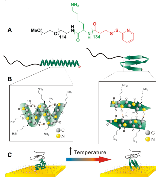
Figure 7. Chemical structure of poly(L-lysine), as well as its schematic representation in \alpha -helical and anti-parallel \beta -sheet conformation. B. Detailed representation of side chains and hydrogen bonding within poly(L-lysine). C. Schematic representation of the \alpha - \beta transition that occurs after the surface functionalized with poly(L-lysine) is exposed to elevated temperatures needed to induce the transition.
