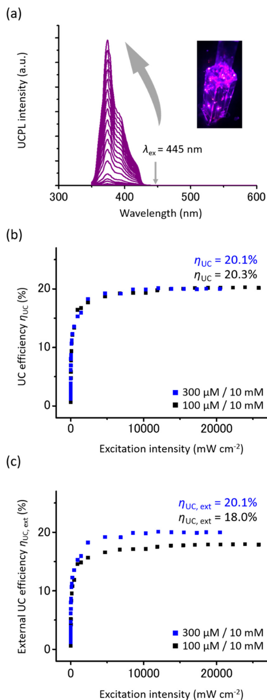
Fig. 3 (a) Upconversion photoluminescence (UCPL) spectra and photograph of the toluene solution of CBDAC (100 \mu\text{M} ) and TIPS-Nph (10 mM) ( \lambda_{\text{ex}} = 445 \text{ nm} , I_{\text{ex}} from 1.33 \text{mW cm}^{-2} to 25.8 \text{W cm}^{-2} , 425 nm short-pass filter). (b) Internal UC efficiency \eta_{\text{UC}} , and (c) external UC efficiency \eta_{\text{UC, ext}} of the mixed solution of CBDAC (100 \mu\text{M} (black), 300 \mu\text{M} (blue)) and TIPS-Nph (10 mM) in deaerated toluene.
