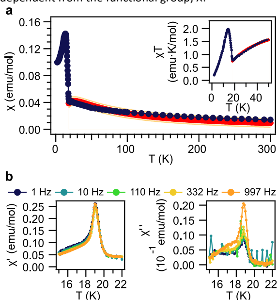
Fig. 3. Magnetic behaviour of MUV-1-F . a) Thermal dependence of \chi . Inset: Thermal dependence of the \chi T product. The data have been fitted (red line) following a Lines expansion for a quadratic-layer Heisenberg antiferromagnet with S = 2 . 21 The red line represents the prediction band with a confidence interval of 95%. b) In-phase (left) and out-of-phase (right) dynamic susceptibility measured at different frequencies.
