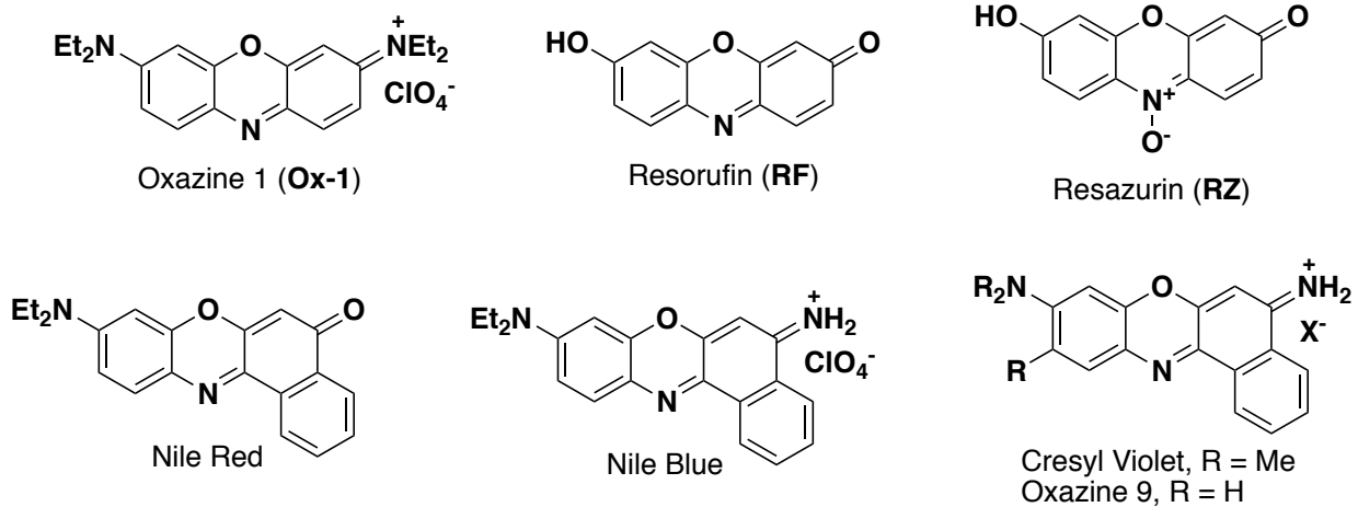
Figure 1. Structures of the most popular phenoxazine dyes currently used in fluorescence-based applications ( \text{X}^- = \text{Cl}^- or \text{ClO}_4^- ).
