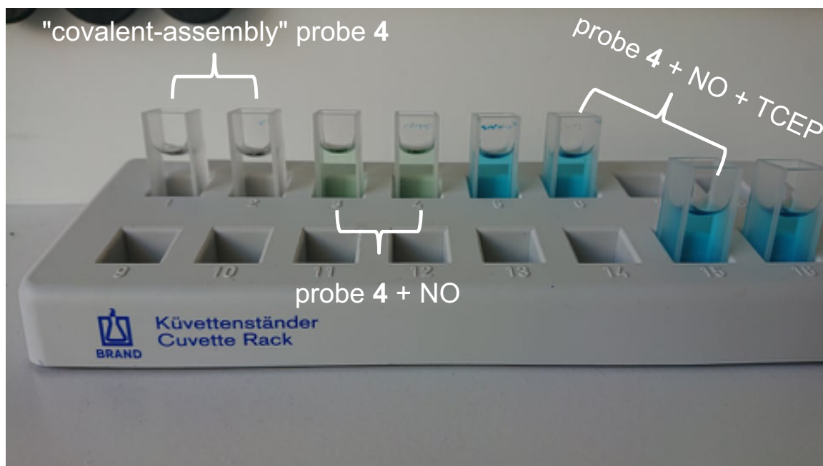
Figure S1. Picture of aq. solutions of "covalent-assembly" fluorogenic probe 4 before and after incubation with either NO (50 equiv.) or NO (50 equiv.) and TCEP (170 equiv.).
