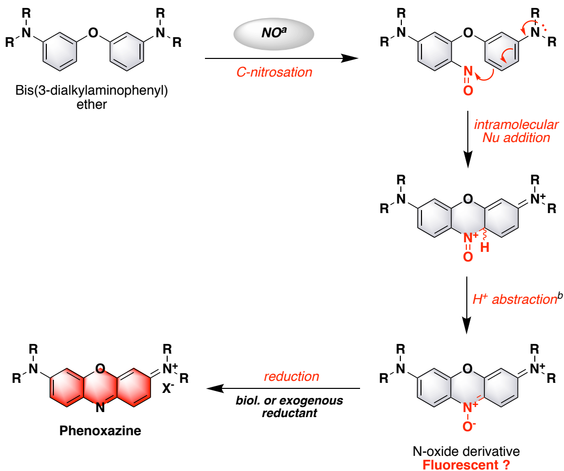
Figure 3. NO-sensing strategy explored in this work based on the use of "covalent-assembly" fluorogenic probes whose activation leads to the in situ formation of phenoxazine dyes [biol. = biological, Nu = nucleophilic, R = alkyl substituent, X - = counter ion not specified]. a Please note: depending the context, the nitrosating species is different: NO + in the case of syntheses using NOBF 4 and probably N 2 O 3 (itself in equilibrium with NO + and NO 2 - ) in the case of experiments performed with freshly prepared aq. solution of nitric oxide. b Please note: depending the context, proton abstraction may be assisted by various species: BF 4 - anion, H 2 O molecule, NO 2 - anion or N-oxide derivative itself.
