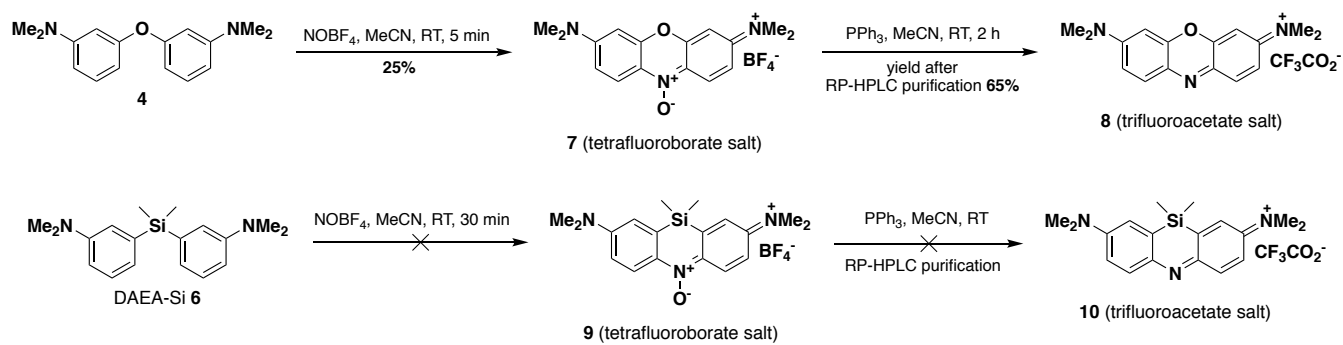
Scheme 2. Synthesis of phenoxazine dye 8 and its silicon analog 10 through NOBF 4 -mediated nitrosation. [RT = room temperature].
