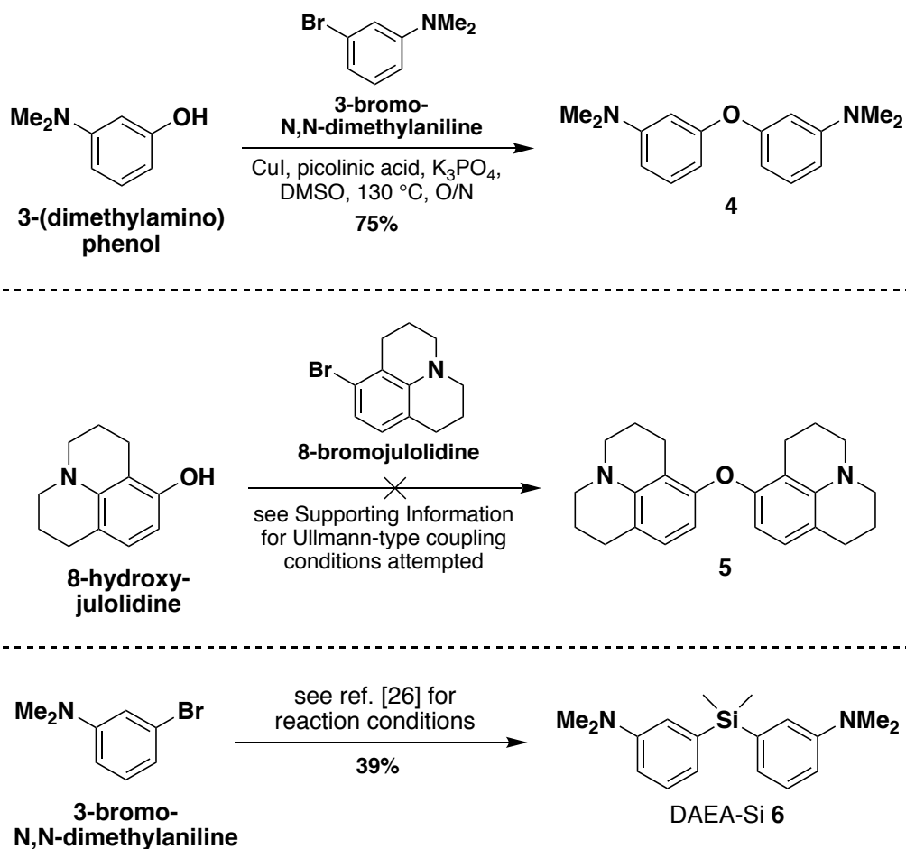
Scheme 1. Synthesis of symmetrical bis-aryl ethers 4 and 5 and the silicon-containing analog DAEA-Si 6 . [O/N = overnight].
