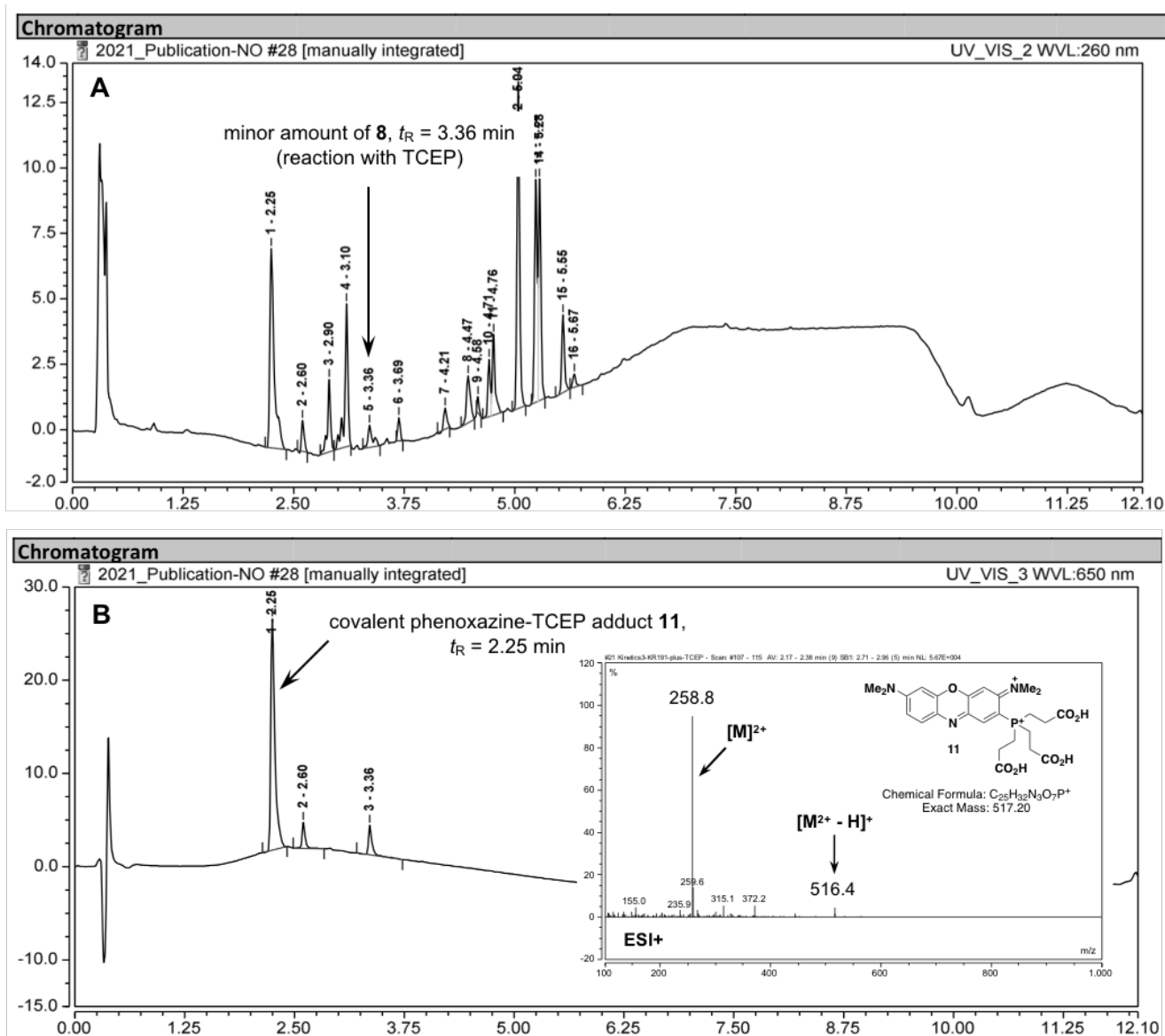
Figure 9. RP-HPLC elution profiles (system D) of "covalent-assembly" fluorogenic probe 4 after sequential incubation with NO (50 equiv., 25 min of incubation) and TCEP (170 equiv., 60 min of incubation) in ultrapure water, at 25 °C. (A) UV detection at 260 nm. (B) Visible detection at 650 nm and ESI+ mass spectrum of peak at t_R = 2.25 min (inset).
