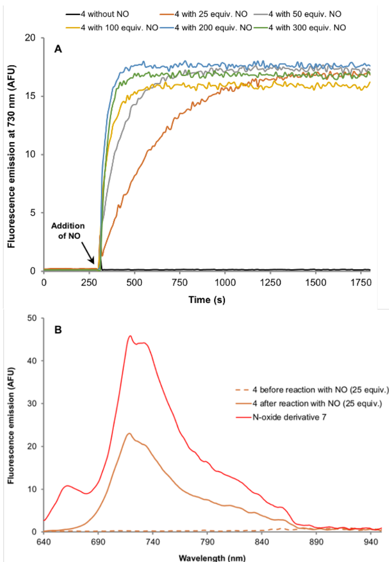
Figure 5. (A) Fluorescence emission time course (Ex/Em 685/730 nm, bandwidth 5 nm, PMT voltage 600 V) of "covalent-assembly" fluorogenic probe 4 , concentration: 10 \mu M, in the presence of various amounts of NO, in ultrapure water at 25 ^{\circ} C. (B) Overlay of fluorescence emission spectra (Ex at 630 nm, bandwidth 5 nm, PMT voltage 600 V) of "covalent-assembly" fluorogenic probe 4 before and after 25 min incubation with NO (25 equiv.), and N-oxide derivative 7 (reference sample synthesized from 4 with \text{NOBF}_4 , see Scheme 2) at the same concentration (10 \mu M) in ultrapure water at 25 ^{\circ} C. Please note: the presented kinetics and emission curves were recorded with a SAFAS Flx-Xenius XC spectrofluorimeter, an instrument that is well suited for high-throughput measurements (e.g., 10 different kinetics at the same time) but providing lower performances than HORIBA Jobin Yvon Fluorolog in the NIR-I spectral range; this explains the poorer quality of emission spectra compared to those presented in Figure 4. The minor band centered at 660 nm and observed in the emission spectrum of reference sample of 7 , is assigned to phenoxazine 8 , formed through a not yet elucidated (photo)reduction process occurring during the prolonged storage of 7 in solution ( i.e. , 1.0 mg/mL stock solution in DMSO).
