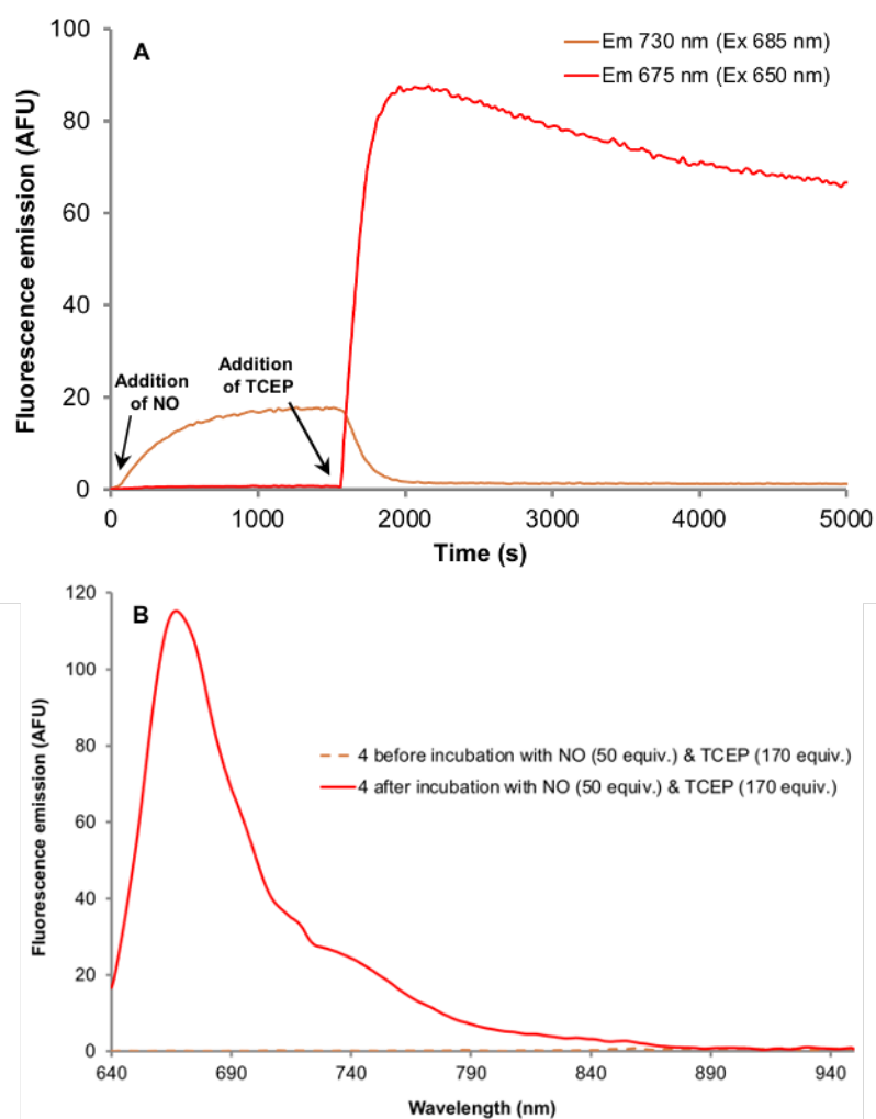
Figure 6. (A) Fluorescence emission time course (channel 1: Ex/Em 685/730 nm for 7 , channel 2: Ex/Em 650/675 nm for 8 ; bandwidth 5 nm, PMT voltage 600 V) of "covalent-assembly" fluorogenic probe 4 , concentration: 10 \mu M, sequentially incubated with NO (50 equiv.) and TCEP (170 equiv.), in ultrapure water at 25 ^{\circ} C. (B) Fluorescence emission spectra (Ex at 630 nm, bandwidth 5 nm, PMT voltage 600 V) of "covalent-assembly" fluorogenic probe 4 , concentration: 10 \mu M, before and after sequential incubation with NO (50 equiv.) and TCEP (170 equiv.), in ultrapure water at 25 ^{\circ} C.
