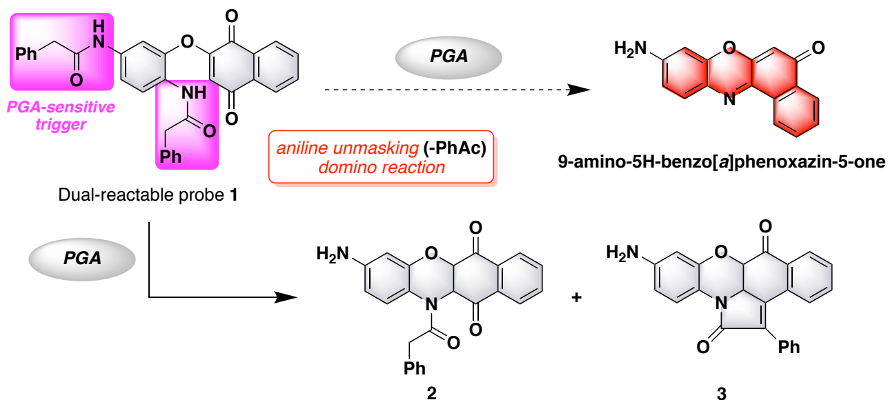
Figure 2. Overview of "covalent-assembly" fluorescent probes reported in the literature, whose activation leads to the in situ formation of phenoxazine dyes or related analogs [ \text{ClO}^- = hypochlorite anion, \text{OONO}^- = peroxyxynitrite anion, PGA = penicillin G acylase, PhAc = phenylacetyl, X - = counter ion not specified]. a Please note: the proneness of probe NO670 to auto-oxidation mitigated its potential for practical applications. Synthesis of NO670 and mechanistic studies related to its conversion into Ox-1 were not published by the Yang group but only mentioned in their review on the "covalent-assembly" principle for fluorescent probe design [16] .
