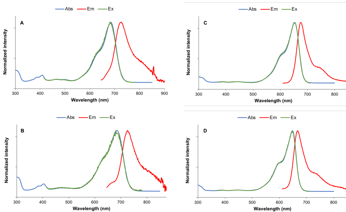
Figure 4. Normalized absorption, fluorescence emission (excitation at 630 nm (A-B) or 600 nm (C-D), Ex/Em slits 5 nm) and excitation (emission at 800 nm (A-B) or 720 nm (C-D), Ex/Em slits 5 nm) spectra of phenoxazine dyes 7 and 8 in DMSO (A, C), and in ultrapure water (B, D) at 25 °C.
