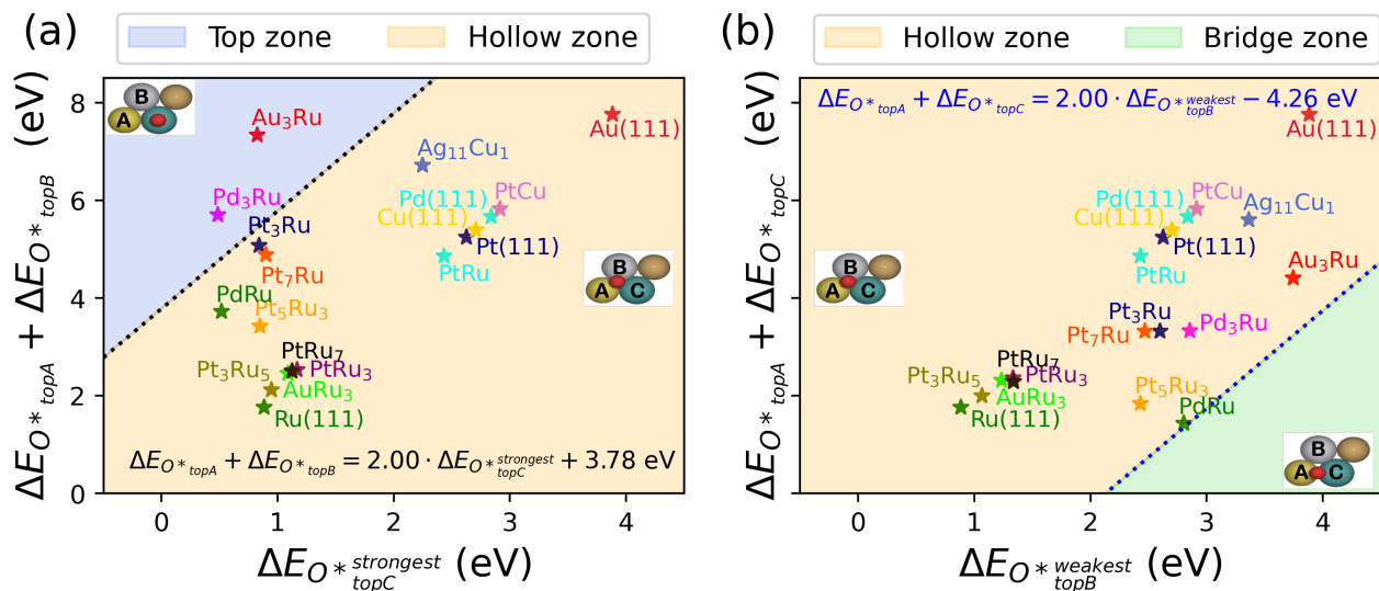
Figure 4: Preferred O* adsorption site. (a) On-top versus hollow sites. The black dotted line is given by eq 14 and represents where on-top and hollow adsorption are equally stable. \Delta E_{O^*_{topC}^{strongest}} is the most stable O* adsorption energy of the three adjacent top sites. (b) Bridge versus hollow sites. The blue dotted line is given by eq 15 and represents where bridge and hollow adsorption are equally stable. \Delta E_{O^*_{topB}^{weakest}} is the weakest O adsorption energy of the three adjacent top sites.
