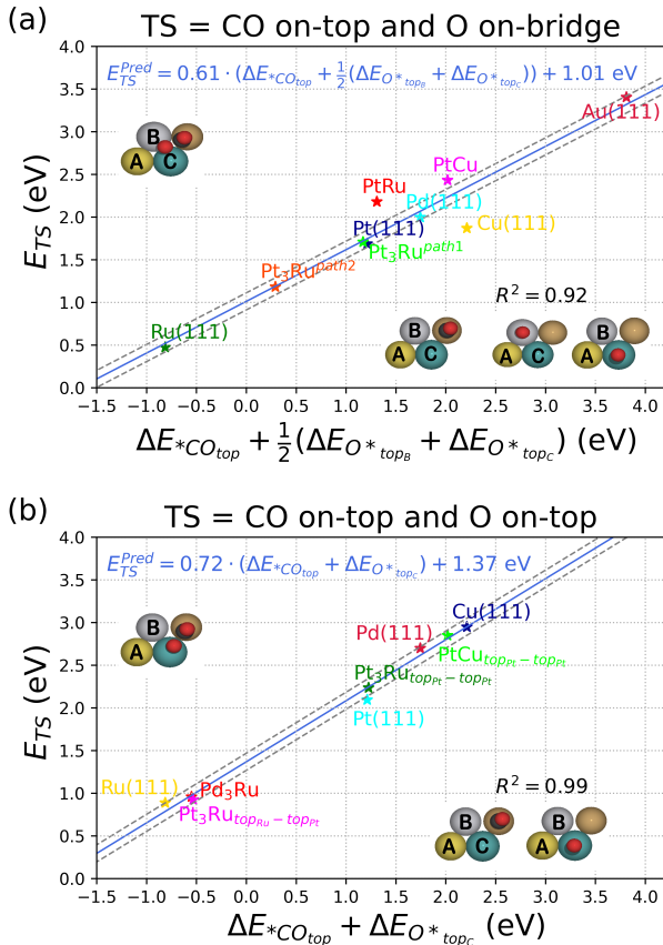
Figure 5: (a) BEP relation between the *CO-top and O*-bridge E_{\text{TS}} and the sum of the *CO on-top adsorption energy and the average of two O* on-top adsorption energies. Figure S6 and S7 in the SI show the NEB pathways going through *CO-top and O*-bridge TS. \text{Pt}_3\text{Ru}^{\text{path1}} and \text{Pt}_3\text{Ru}^{\text{path2}} are different pathways with O* going through the Pt-Pt and Pt-Ru TS, respectively. (b) BEP relation between the *CO-top and O*-top E_{\text{TS}} and the sum of the *CO on-top adsorption energy and the O* on-top adsorption energy. Figure S8 and S9 in the SI shows the NEB pathways going through *CO-top and O*-top TS. The dashed lines are \pm 0.1 eV offset from the blue lines.
