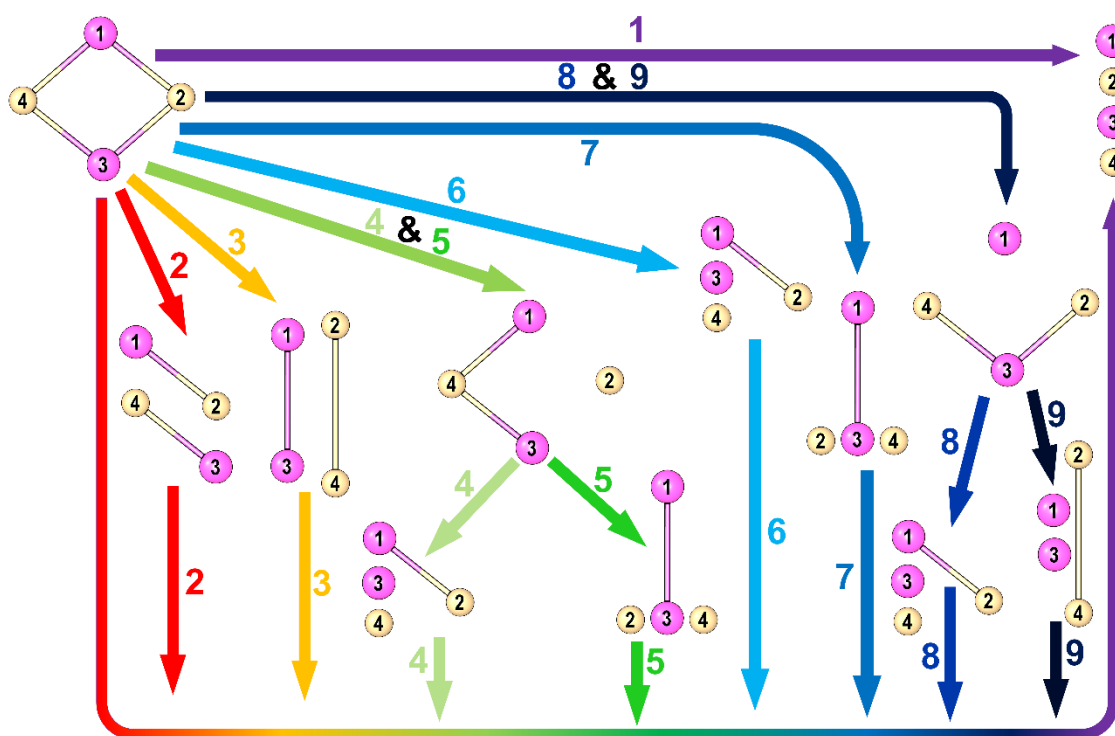
Figure 1. Schematic representation of nine pathways for breaking \text{M}_2\text{X}_2 into four isolated ions. Here, 1 and 3 represent metal atoms, and 2 and 4 denote nonmetals.
