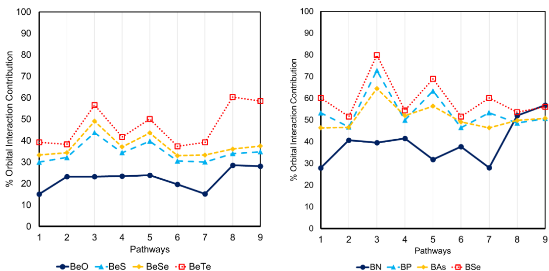
Figure 2. The percentage of the contribution of \Delta E_{oi} in total interaction energy in dimers of beryllium chalcogenides and boron pnictogenides obtained from nine different pathways.
