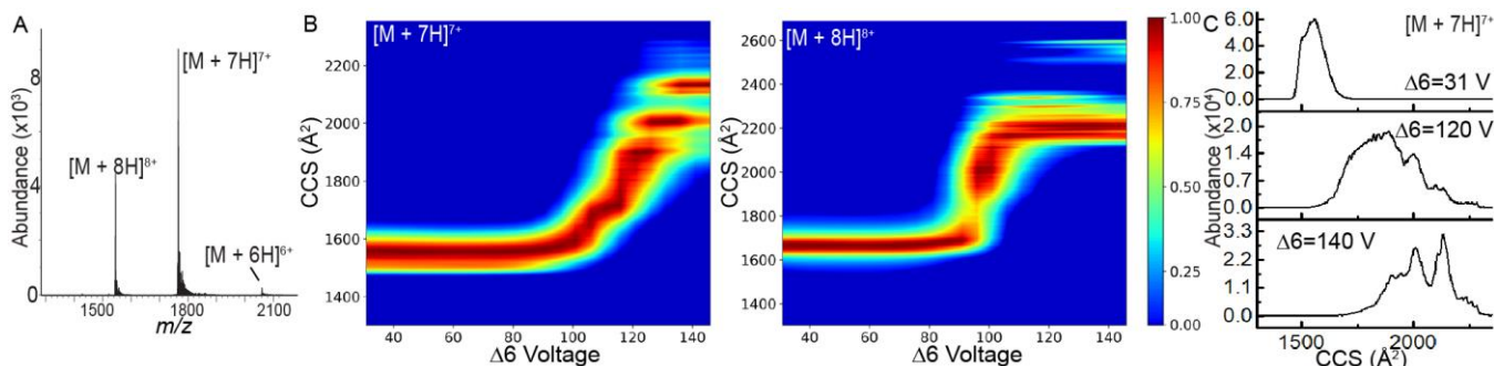
Figure 3. A) Native mass spectrum of cytochrome C. B) CIU fingerprints of the 7+ and 8+ charges states of cytochrome C. C) Mass resolved mobility spectra of the 7+ charge state of cytochrome C following activation at the indicated \Delta 6 . Tunnel-in pressure=2.5 mbar.
