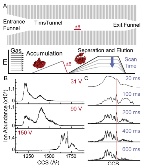
Figure 1. A) Diagram of TIMS device and plot of the applied electric field at various steps of the TIMS analysis with the location of the \Delta 6 DC voltage indicated on both (PDB accession codes 6EYY and 6LKF). B) Mass resolved mobility spectra of the 6+ charge state of ubiquitin at increasing \Delta 6 values. C) Mobil-
