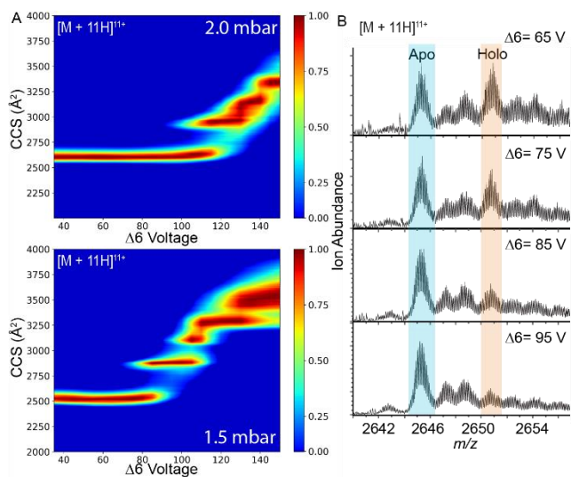
Figure 5. A) CIU fingerprints of the 11+ charge state of Carbonic Anhydrase at tunnel-in pressure= 2.0 mbar (top) and 1.5 mbar (bottom). B) Mass spectra of the 11+ charge state of apo and holo-carbonic anhydrase at indicated \Delta 6 value.
