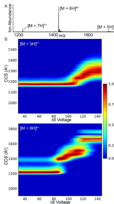
Figure 2. A) Mass spectrum of native-like ions of ubiquitin. B) CIU fingerprints of the 5+ (top) and 6+ (bottom) charge states of ubiquitin (Tunnel-in pressure = 2.5 mbar).
