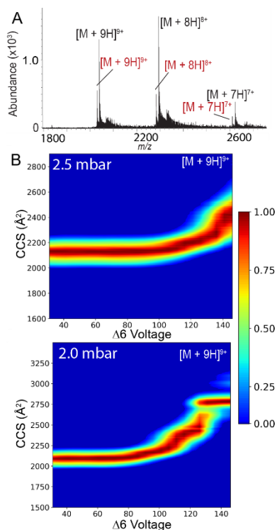
Figure 4. A) Native mass spectrum of \beta -lactoglobulin. The A and B isoforms are indicated in Black and red, respectively. B) CIU fingerprint of BLG A at a tunnel-in pressure of 2.5 (top) and 2.0 (bottom) mbar.
