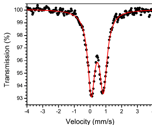
Figure 2. Mössbauer spectra of 3 at 80 K. Simulation in red with \delta = 0.460(2) mm/s and \Delta E_Q = 0.765(3) mm/s. the oxidation state from an Fe(II) complex to an Fe(III) complex (see SI). Numerous unsuccessful attempts were made to grow crystals suitable for X-ray diffraction at -78 °C and the EXAFS region of 3 is unfortunately too noisy for reliable structural determination.
