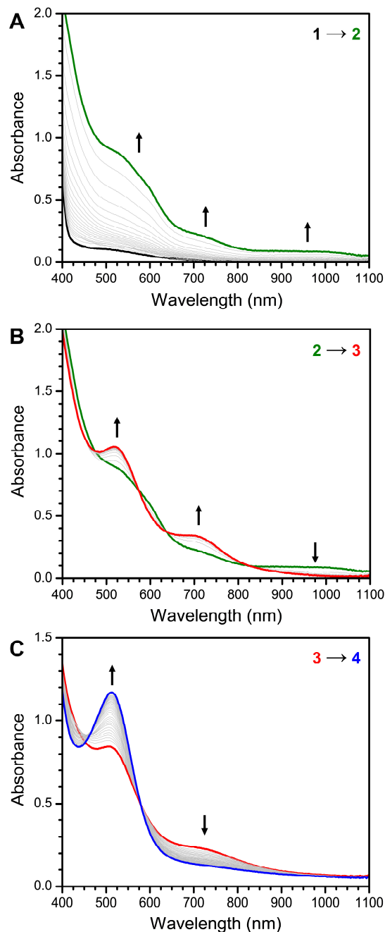
Figure 1. UV-visible spectroscopy of a 0.35 mM solution of 1 in toluene at -60 °C upon addition of 0.5 mL of O 2 where 1 is black, 2 is green, 3 is red, and 4 is blue. (A) Formation of 2 with scans every 1 minute starting 2 minutes after O 2 addition. (B) Formation of 3 from 2 with scans every 5 minutes. (C) Growth of 4 from 3 at -10 °C from a 0.35 mM solution of 1 in toluene. Scans were collected every 10 minutes.
