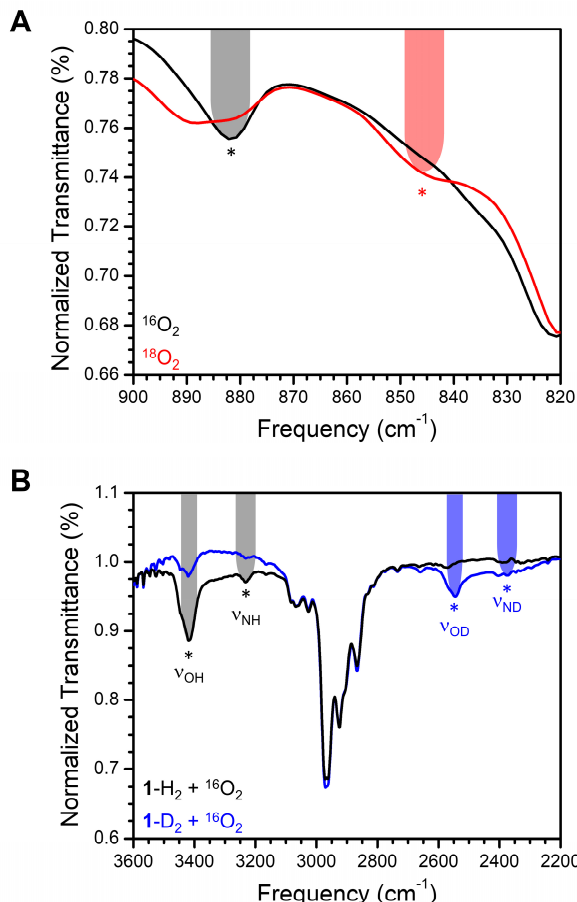
Figure 3. Variable isotope IR spectra of the reaction of 1 with O 2 at RT to form 3 . (A) 16 O 2 vs. 18 O 2 reacted with 1 in the solid state collected as a KBr pellet in the peroxy stretching region. (B) Proteo- vs. deuterio- 1 (83% enriched) reacted with 16 O 2 collected as concentrated solutions in chlorobenzene.
