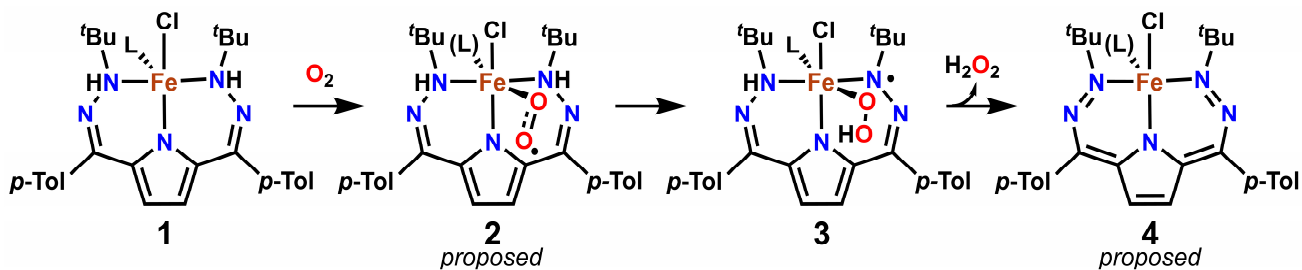
Scheme 2. Reaction of 1 with \text{O}_2 .
