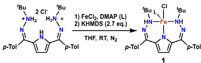
Scheme 1. Metalation of t Bu, Tol DHP-H 2 •2HCl with FeCl 2 .
