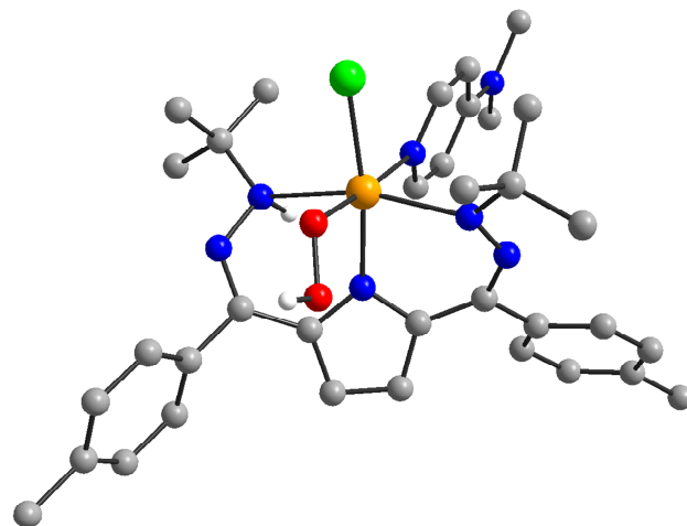
Figure 4. DFT computed structure of 3 with Fe in orange, C in gray, N in blue, O in red, Cl in green, and selected H's in white. Computational Analysis of 3
