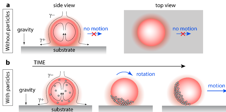
Figure 4. Spontaneous polarization of particles on solubilizing oil droplet interfaces leads to enhanced self-propulsion. a. An oil droplet that solubilizes but does not self-propel can still experience an interfacial tension gradient from top to bottom where the asymmetry is imposed by the substrate. Solubilized oil builds up near the solid surface, generating Marangoni flows that advect oil-free surfactant from above (side view). The droplet does not move laterally because the oil solubilization is axially symmetric about the vector perpendicular to the surface (top view). \gamma^+ indicates an elevated interfacial tension and \gamma^- indicates a lowered interfacial tension. See Video S4 . b. When particles are introduced, advection of the interfacially-adsorbed particles creates a cap. Once the cap rotates, droplets move laterally; droplets move most quickly when the particle cap is oriented perpendicular to the substrate. See Videos S5-S6 .
