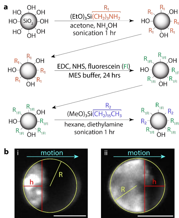
Figure 2. Fluorescence visualization of particles at droplet interfaces. a. Schematic describing the preparation of fluorescent, hydrophobic fumed silica. b. The particle surface coverage of a droplet was estimated using fluorescence micrographs. Fluorescence images of two different droplets, both prepared with 1 wt% fluorescent particles in bromodecane with 0.5 wt% TX, are shown as examples. Overlaid diagrams illustrate how particle surface coverage was estimated by assuming a spherical cap, where h is the height of the cap and R is the radius of the droplet (and cap). For (i), estimated fractional surface coverage = h/2R=32\% , and for (ii) fractional surface coverage = 1-h/2R=70\% . Scale, 50 \mu\text{m} .
