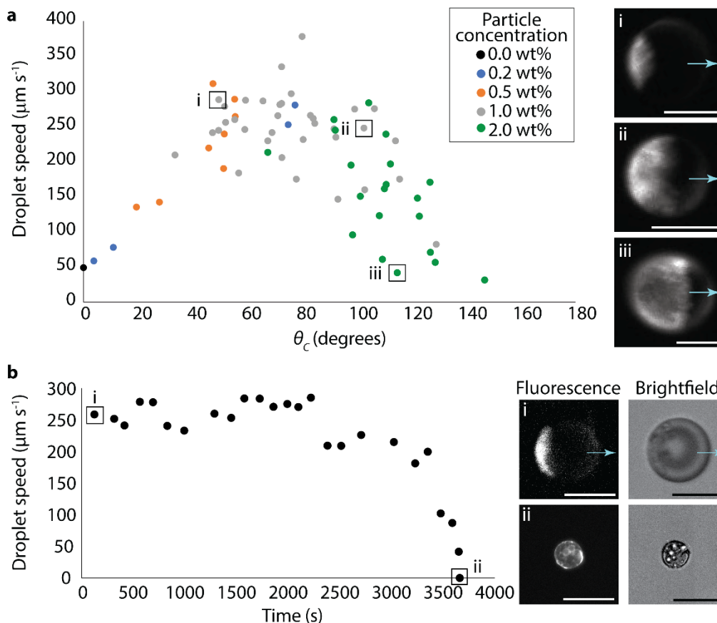
Figure 3. Degree of droplet surface covered by particles affects droplet speed. The scatterplot shows the relationship between bromodecane droplet speed and surface coverage with particles in 0.5 wt% TX. Surface coverage is plotted as coverage cap angle \theta_c , where \theta_c=0^\circ corresponds to no particle coverage and \theta_c=180^\circ corresponds to complete coverage. Each datapoint represents a single droplet's surface coverage and highest speed reached during imaging. The color coding of the datapoints represents the initial concentration of particles used when preparing the droplet. Black = 0.0 wt%, blue = 0.2 wt%, orange = 0.5 wt%, grey = 1.0 wt%, and green = 2.0 wt% fluorescent particles in bromodecane. The initial particle concentration showed a general correlation with droplet surface coverage, where higher particle concentrations were more likely to produce droplets with higher surface coverages. Fluorescence micrographs of three exemplary droplets are shown and the arrows represent direction of droplet motion. Scale, 50 \mu\text{m} . b . The scatterplot shows the evolution of a single bromodecane droplet's speed over its lifetime of about an hour in 0.5 wt% TX. The droplet started with fast speeds and moderate particle coverage ( \theta_c \approx 50^\circ ). Over time, the particle coverage increased while the droplet volume decreased due to solubilization, until eventually the droplet motion ceased with \theta_c \approx 180^\circ . Fluorescence and brightfield micrographs are given at right. The arrows represent the direction of droplet motion. Scale, 100 \mu\text{m} .
