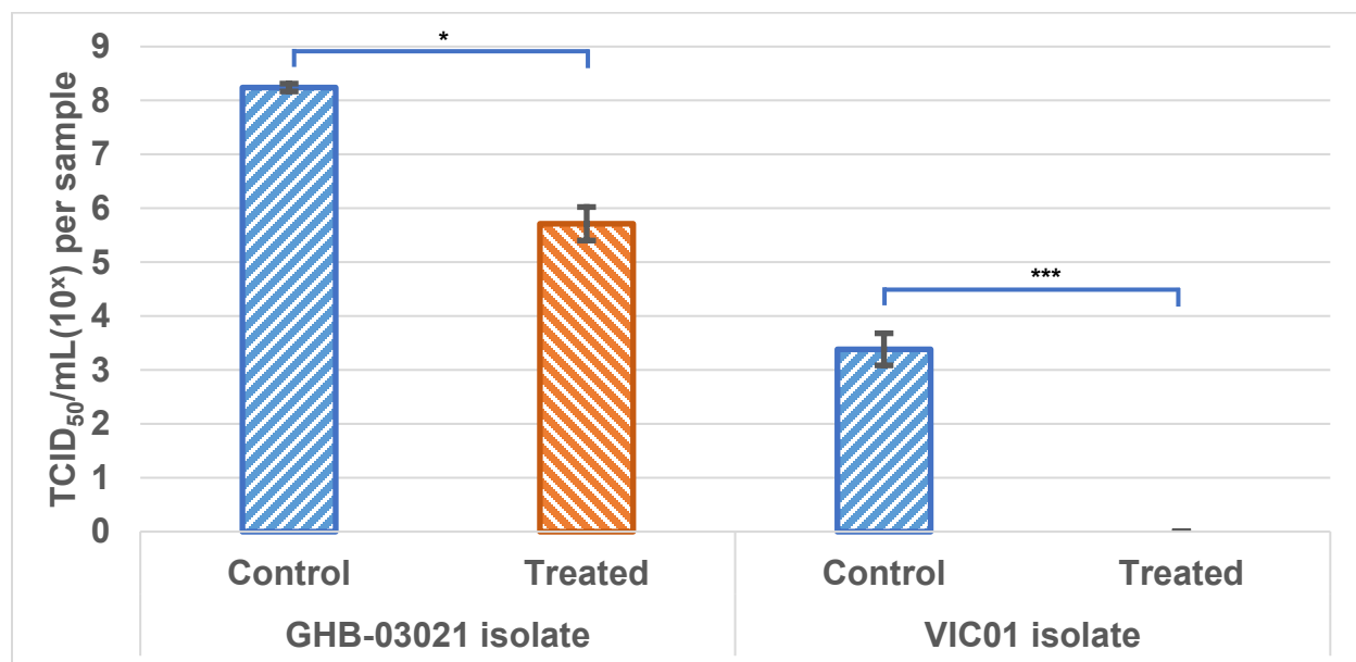
Figure 2 – The carrier surface test was used to evaluate the antiviral activity against SARS-CoV-2 isolates GHB-03021 and VIC01. The treated surfaces for each isolate were prepared by two different methods. An electrostatic sprayer applied SiQAC-C18 to surfaces used for the GHB-03021 exposure, while product was applied using an air brush sprayer for samples exposed to VIC01. After drying and a further contact time of 10 min, surfaces were washed, eluate collected and remaining infectious virus titre determined by a TCID 50 assay.
