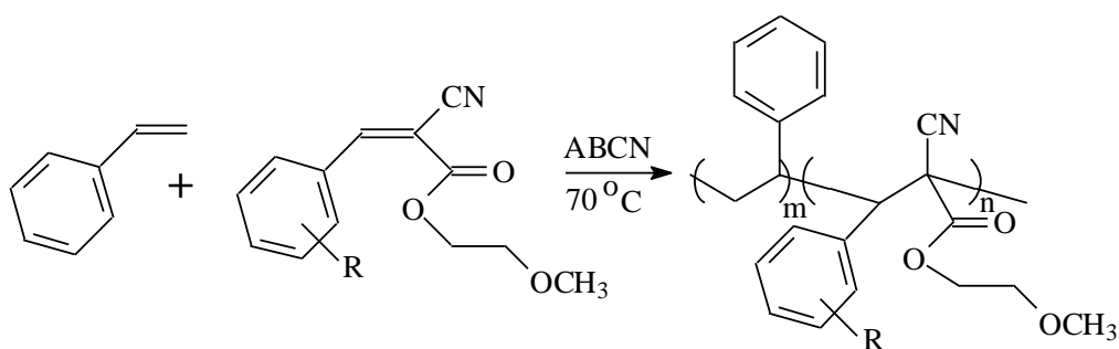
Scheme 2. Copolymerization of ST and phenoxy ring-substituted 2-methoxyethyl phenylcyanoacrylates, RPhCH = C(CN)CO_2CH_2CH_2OCH_3 . R is 2-fluoro-3-methoxy, 2-fluoro-4-methoxy, 2-fluoro-5-methoxy, 2-fluoro-6-methoxy, 3-fluoro-4-methoxy, 4-fluoro-
