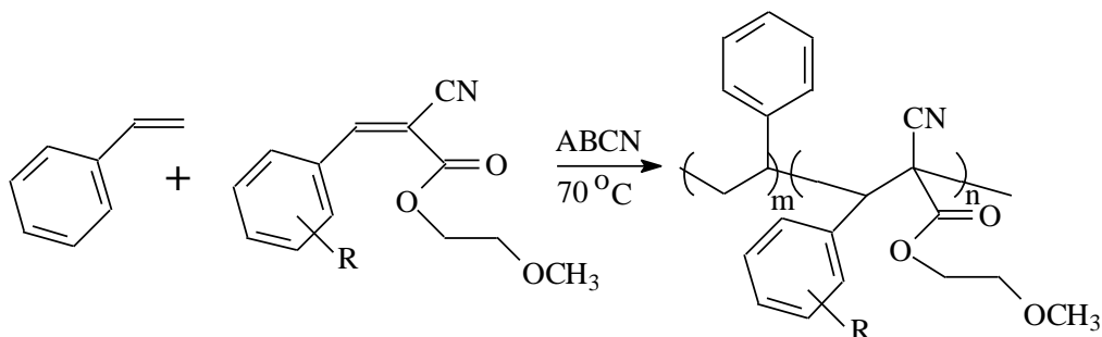
Scheme 2. Copolymerization of ST and phenoxy ring-substituted 2-methoxyethyl phenylcyanoacrylates, RPhCH = C(CN)CO_2CH_2CH_2OCH_3 . R is 4-methoxy-2-methyl, 4-methoxy-3-methyl, 3-ethoxy-4-methoxy, 4-ethoxy-3-methoxy, 3,4-dibenzyloxy, 3-benzyloxy-4-methoxy, 4-benzyloxy-3-methoxy, 2-bromo-5-methoxy, 3-bromo-4-methoxy, 5-bromo-2-methoxy, 2-chloro-3-methoxy, 3-chloro-4-methoxy, 2-chloro-6-methyl, 3-chloro-4-methyl.
