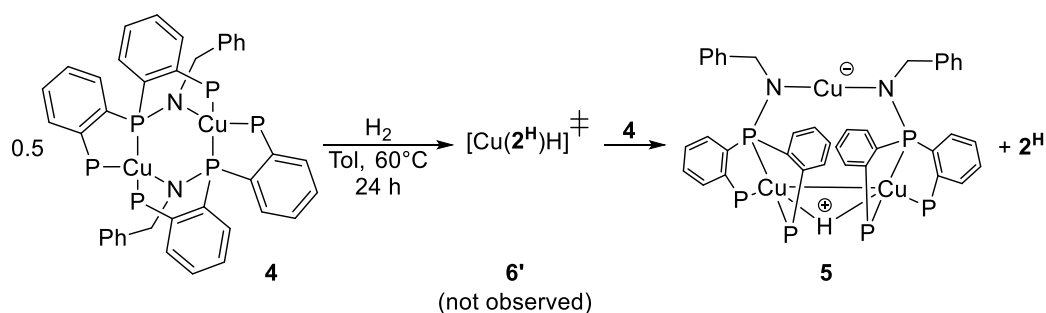
Scheme 4. Formation of 5 through activation of \text{H}_2 on 4 and putative generation of a copper hydride intermediate
