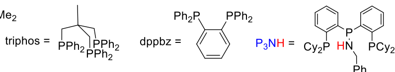
Scheme 1. Copper(I) hydride complexes obtained by hydrogenation methods
