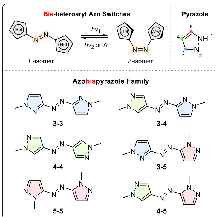
Figure 1. Molecular design of azobispyrazole family. ( N -methylation is necessary to prevent the azo-hydrazone tautomerization that dramatically accelerates thermal Z → E isomerization.)
