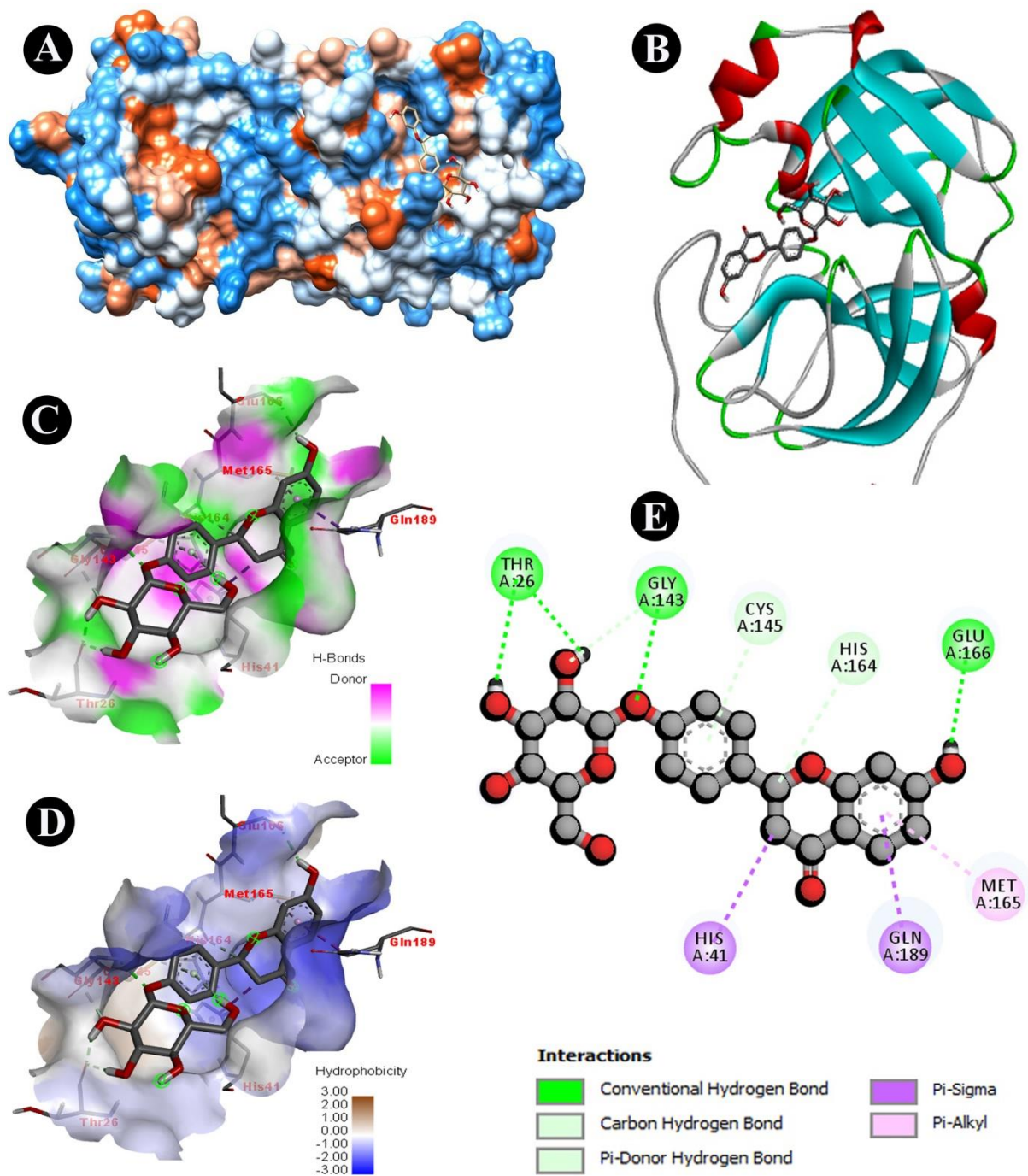
Fig. 3 Docking analysis of SARS-CoV-2 M^{pro} binding with Liquiritin (A) hydrophobicity surface 3D representation (B) 3D representation of Liquiritin-SARS-CoV-2 M^{pro} interaction (C) Interactions of Liquiritin through H-bond in a pocket site of SARS-CoV-2 M^{pro} (D) Interactions of Liquiritin through hydrophobic bond in a pocket site of SARS-CoV-2 M^{pro} (E) 2D representation of Liquiritin in active site of SARS-CoV-2 M^{pro}
