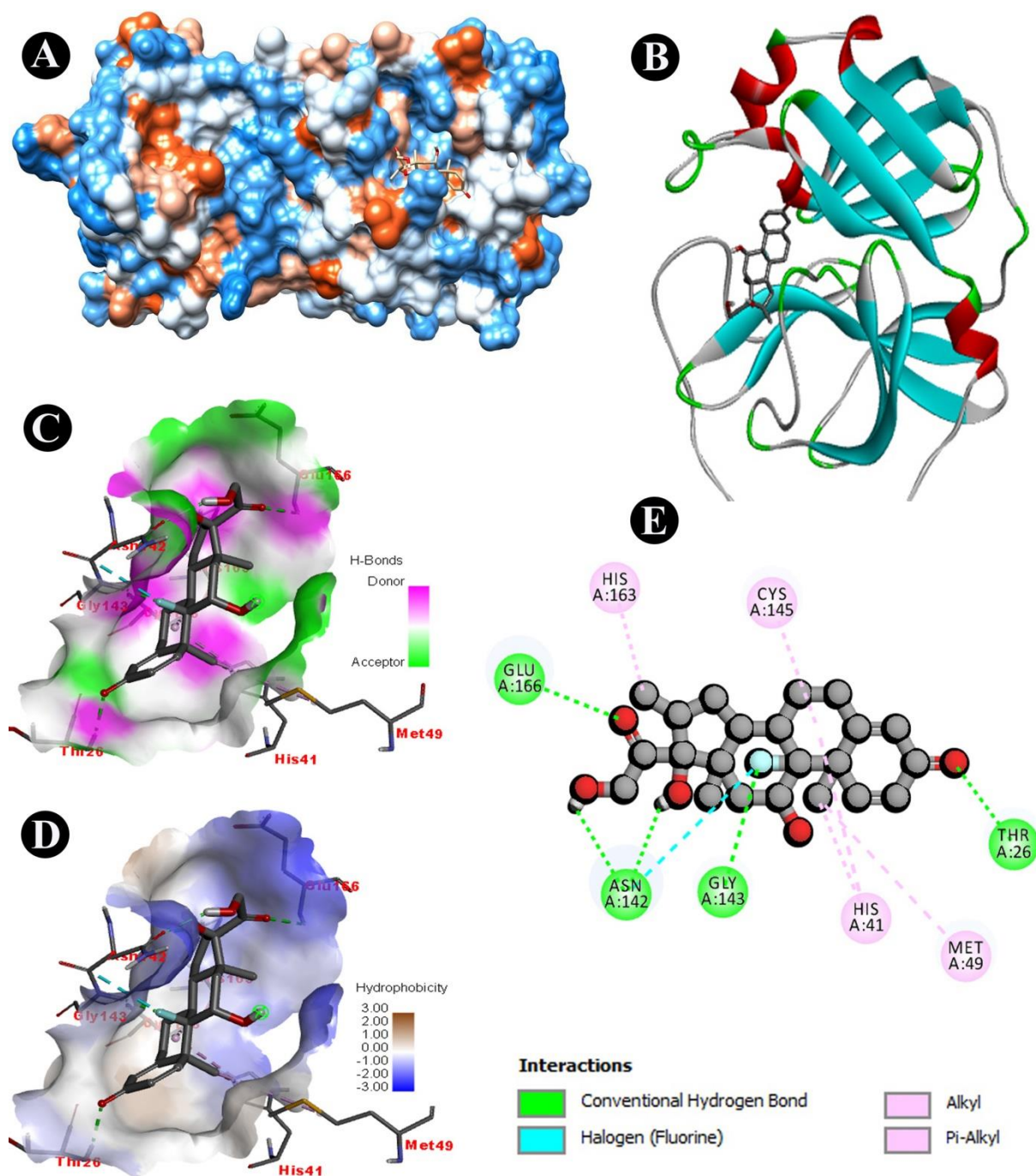
Fig. 2 Docking analysis of SARS-CoV-2 M pro binding with Dexomethasone (A) hydrophobicity surface 3D representation (B) 3D representation of Dexomethasone -SARS-CoV-2 M pro interaction (C) Interactions of Dexomethasone through H-bond in a pocket site of SARS-CoV-2 M pro (D) Interactions of Dexomethasone through hydrophobic bond in a pocket site of SARS-CoV-2 M pro (E) 2D representation of Dexomethasone in active site of SARS-CoV-2 M pro
