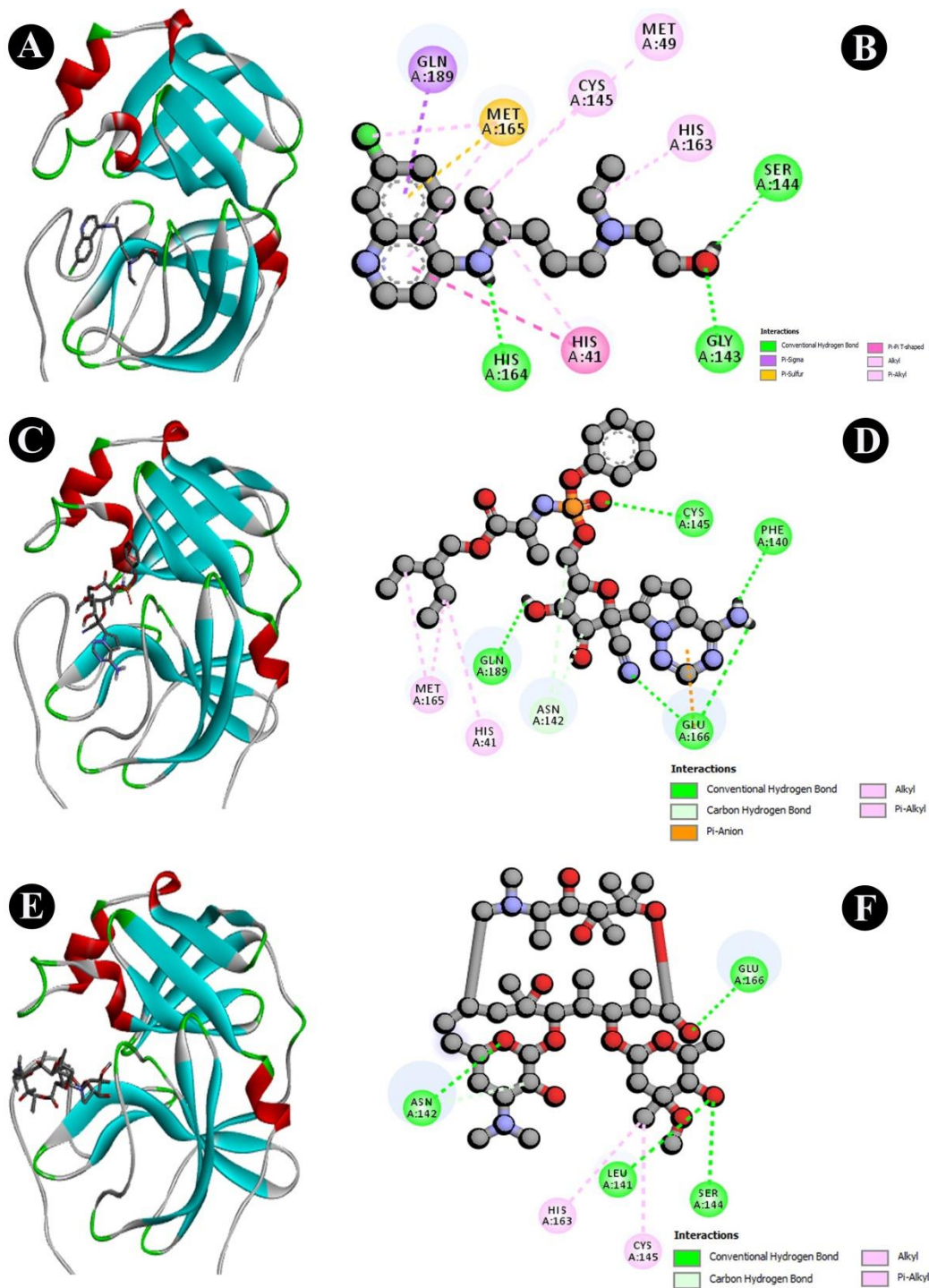
Fig. 1 Docking analysis of SARS-CoV-2 M pro binding with Hydrochloroquine, Remdesivir and Azithromycin (A) 3D representation of Hydrochloroquine-SARS-CoV-2 M pro interaction (B) 2D representation of Hydrochloroquine in active site of SARS-CoV-2 M pro (C) 3D representation of Remdesivir-SARS-CoV-2 M pro interaction (D) 2D representation of Remdesivir in active site of SARS-CoV-2 M pro (E) 3D representation of Azithromycin-SARS-CoV-2 M pro interaction (F) 2D representation of Azithromycin in active site of SARS-CoV-2 M pro
