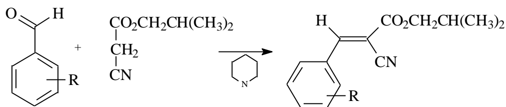
Scheme 1. Synthesis of isobutyl R-phenylcyanoacrylates, where R is 2,3,4-trimethoxy, 2,4,5-trimethoxy, 2,4,6-trimethoxy, 3,4,5-trimethoxy, 4-benzyloxy-3,5-dimethyl, 2-chloro-3,4-dimethoxy, 3-chloro-4,5-dimethoxy, 5-chloro-2,3-dimethoxy.
