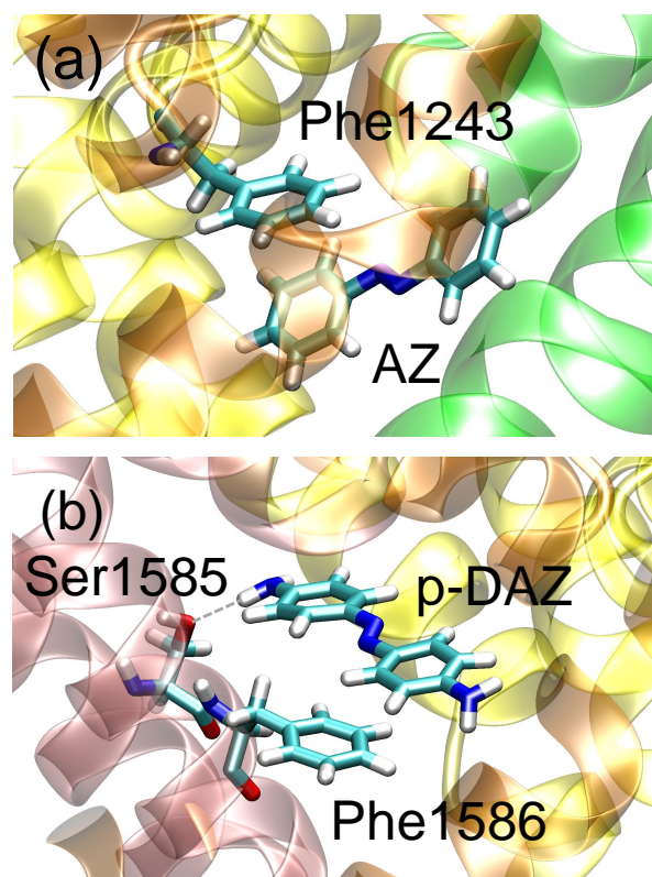
Fig. 6 (a) Stacking interaction between AZ and Phe1243 in the pocket p2. (b) Interaction of p-DAZ with Phe1586 and Ser1585 by stacking and hydrogen bonding, respectively, in the pocket p1. Color code for atoms: cyan for C, red for O, blue for N, and white for H.
