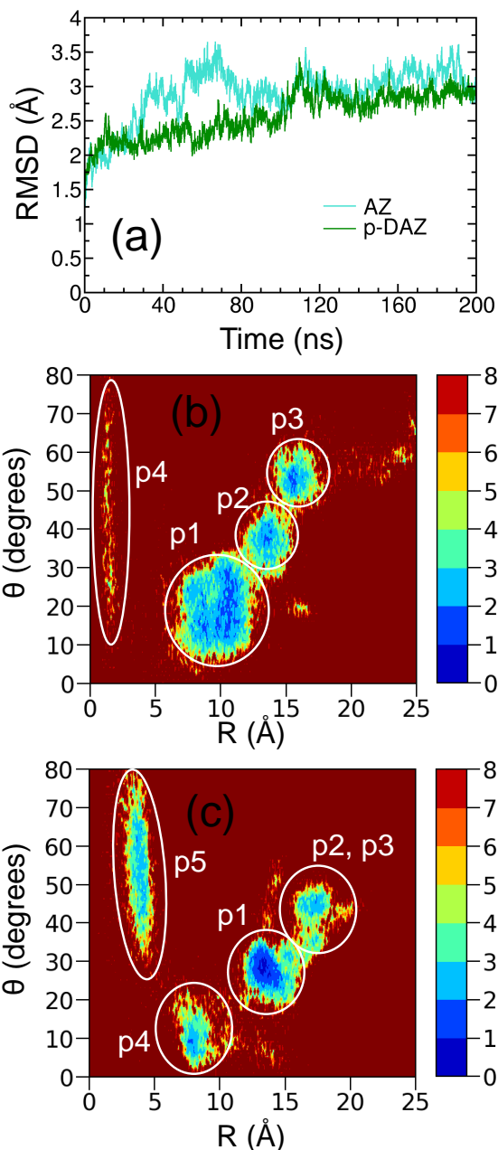
Fig. 2 (a) Root mean squared displacement (RMSD) of the non hydrogen atoms of the the human Na \gamma 1.4 channel interacting with AZ (light blue) and p-DAZ (green) in cMD simulations. Binding pockets for (b) AZ and (c) p-DAZ on the free-energy surfaces computed from the GaMD simulations.
