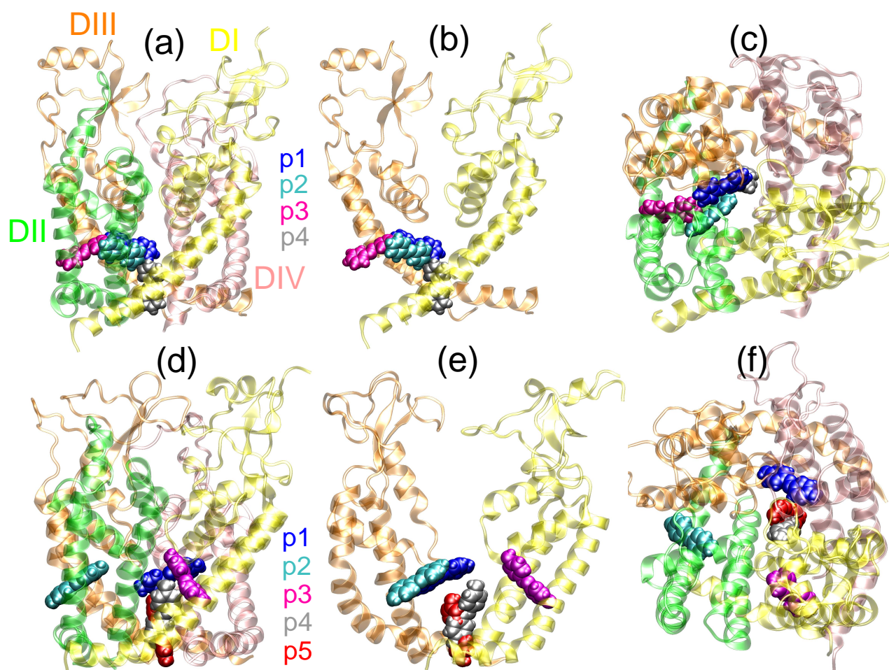
Fig. 3 One representative snapshot for each of the binding pockets of (a)-(c) AZ and (d)-(f) p-DAZ on the human Nav v 1.4 channel from different perspectives. The panels (a) and (d) are side views from the plane of the lipid membrane where the the four protein domains are shown, while the panels (b) and (e) display a similar side view but from a different orientation and only the DII and DIV domains are shown. The panels (c) and (f) show a top down view. The photoswitches located in the binding pockets p1, p2, p3, p4 and p5 are shown in blue, cyan, magenta, grey and red, respectively.
