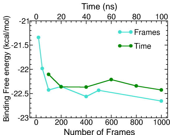
Fig. 4 Variation of the binding free energy of p-DAZ inside the binding pocket 5 of the \text{Na}_v1.4 channel with time and number of snapshots.
