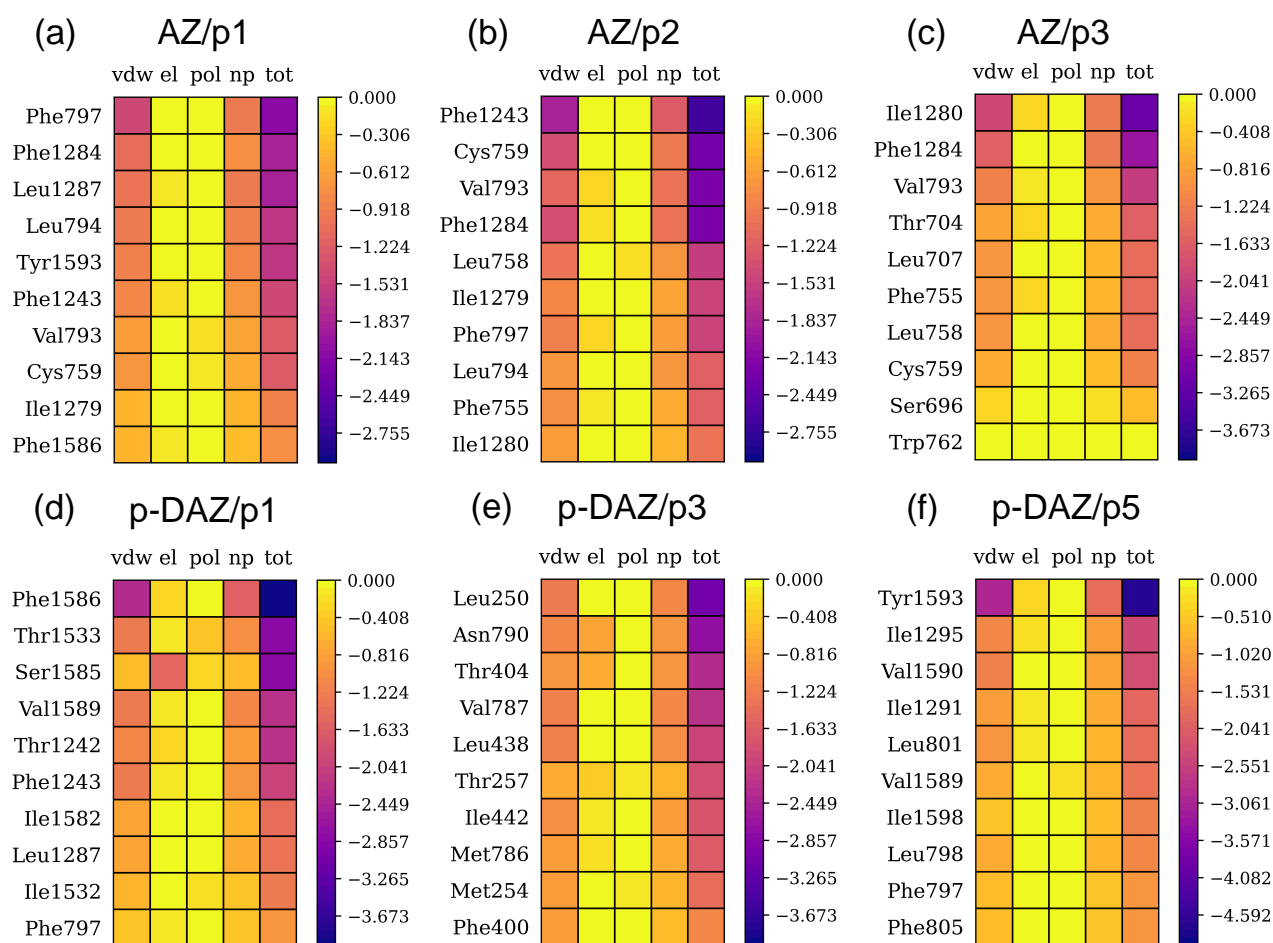
Fig. 5 Pairwise residue decomposition of the binding free energy for the pockets p1 (a), p2 (b) and p3 (c) of AZ and p1 (d), p3 (e) and p5 (f) of p-DAZ. Each residue contribution is in turn decomposed into ligand/protein van der Waals (vdW) and electrostatic (el) contributions and polar (pol) and nonpolar (np) solvation contributions to the total residue binding energy (tot).
