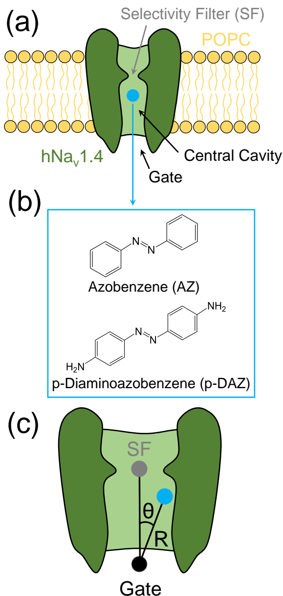
Fig. 1 (a) Schematic representation of the human Nav v 1.4 channel (green) integrated into a solvated POPC bilayer (yellow) with a photoswitch (cyan circle) interacting with the protein inside its central cavity. (b) Chemical formula of the two photoswitches investigated, namely, azobenzene (AZ) and p-diaminoazobenzene (p-DAZ). (c) Reaction coordinates employed to represent the free-energy surface: Distance R between the centers of mass of the photoswitches (cyan circle) and of the gate (black circle), and angle \theta formed by the centers of mass of the photoswitch, of the gate and of the selectivity filter (grey circle). The center of mass of the gate is defined as the center of mass of the \alpha carbons of residues Val446, Leu800, Val1293, and Ile1596 located at the gate. The center of mass of the selectivity filter is defined as the center of mass of the \alpha carbons of the residues that compose the so-called DEKA filter, namely, Asp406, Glu761, Lys1244, and Ala1536.
