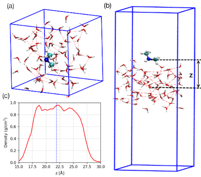
Fig. 1 Representative (a) bulk and (b) slab configurations of dimethylamine in explicit water. (c) Mass density profile of the water slab investigated in this work. The blue dashed line indicates the center of the slab.
