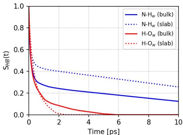
Fig. 5 Continuous hydrogen bond auto-correlation functions for \text{N-H}_w and \text{H-O}_w pairs.
