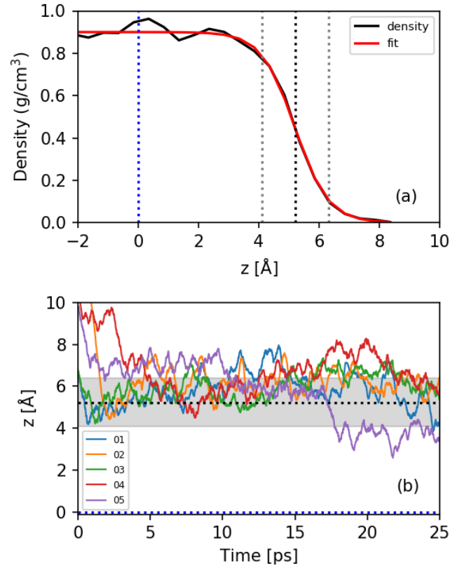
Fig. 2 (a) Fitted density profile of the water slab. The vertical black dotted line indicates the position of z_{\text{GDS}} , and grey dotted lines indicate the interfacial thickness, z_{\text{GDS}} \pm \delta (b) Distance between the center of mass of the slab and the N atom of dimethylamine. The Gibbs dividing surface is denoted by the horizontal black dotted line, and the grey area is the interfacial thickness within \pm\delta of the slab. The dotted blue lines in both panels indicate the center of the slab, which is set to zero in our calculations.
