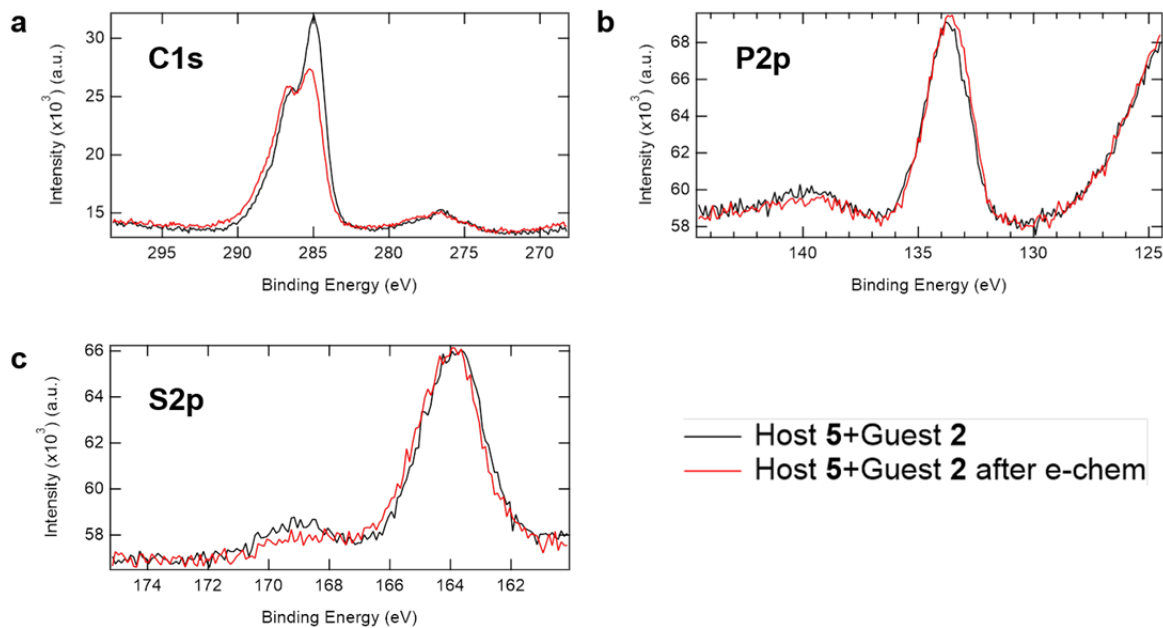
Figure 5. XP spectra of ITO electrodes functionalized with host 5 and HGC-bound guest 2 before and after electrocatalytic measurements ( \text{NH}_3 oxidation in THF solution). a) C1s spectra. b) P2p spectra. c) S2p spectra. For S2p and P2p, no difference between the sample before and after electrocatalysis is observed, showing no change in oxidation state or decrease in surface coverage for either of the elements. In the case of C1s, a decrease in signal intensity is only observed for the peak at 285 eV which is attributed to adventitious carbon, with the signal from host C-O carbon species remains unchanged. Overall the data indicate that no degradation of the host takes place under operating conditions.
