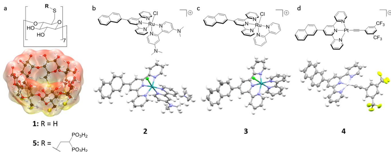
Figure 1. Structures of the main compounds used in this paper: a) host 1 (thiolated cyclodextrin) and host 5 (bisphosphonated cyclodextrin), along with a depiction of the host cavity; b) guest 2 c) guest 3 d) guest 4 . The crystal structures of guests are displayed showing the 50 % thermal ellipsoids. Solvent and counterions ( \text{PF}_6^- for guests 2 and 3 ; \text{ClO}_4^- for guest 4 ) are omitted for clarity.
