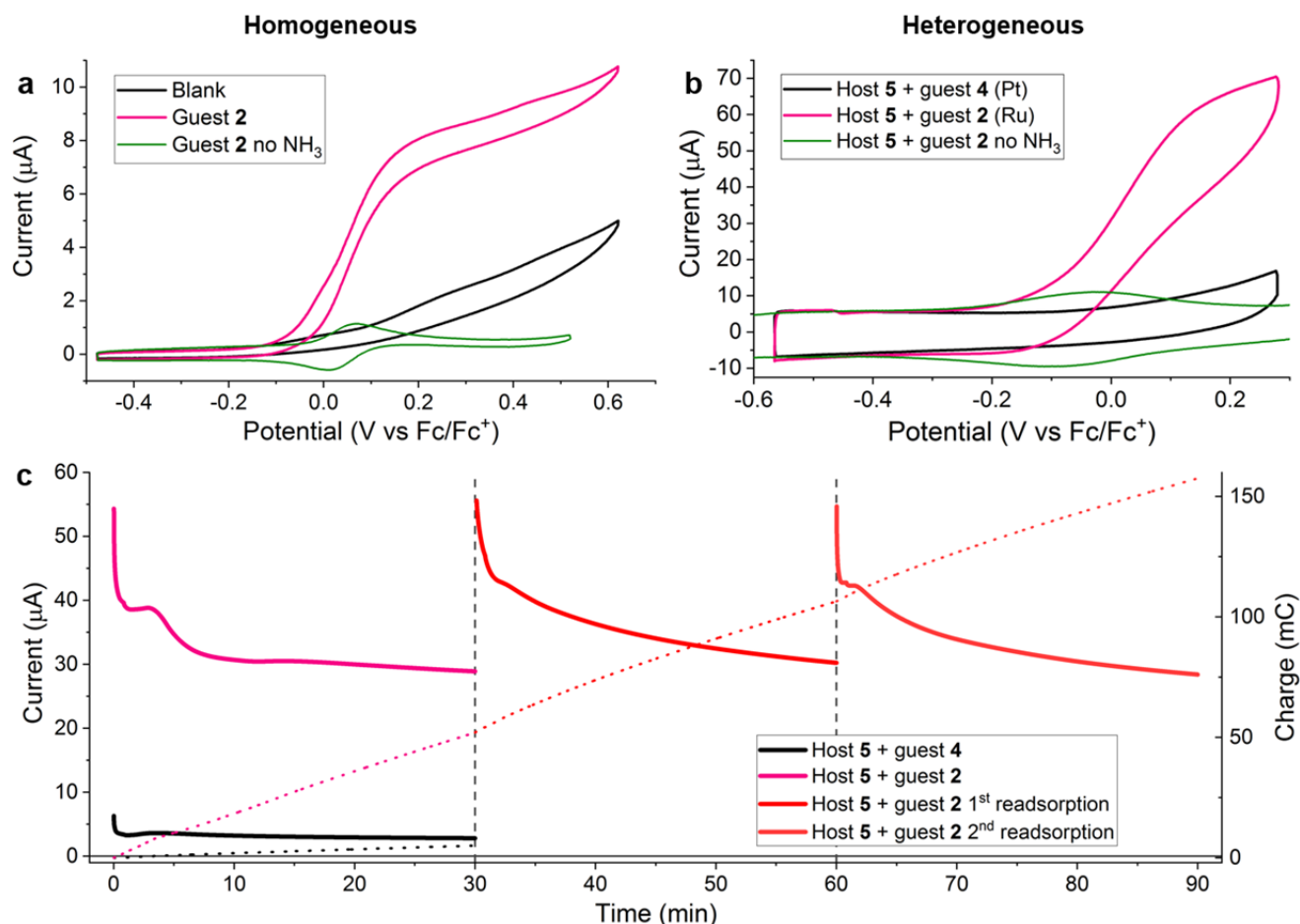
Figure 4. Electrocatalytic oxidation of \text{NH}_3 in THF solution. a) CV scan under homogeneous reaction conditions using an ITO working electrode in \text{NH}_3 saturated THF solution (0.2 M \text{TBAPF}_6 and 0.1 M \text{NH}_4\text{PF}_6 as conducting salt and proton source; 10 mV/s scan rate). Without catalyst (black) shows low activity. For a 0.1 mM solution of guest 2 in the absence of \text{NH}_3 , the \text{Ru(II)}/\text{Ru(III)} redox peak is observed (green). Upon addition of ammonia, a catalytic onset for ammonia oxidation is observed at the \text{Ru(II)}/\text{Ru(III)} oxidation potential (magenta). b) CV scans of HGC-bound guests 2 (magenta) and 4 (black) with host 5 on mesoporous ITO show the same catalytic behaviour in the presence of the ruthenium catalyst, with onset at the \text{Ru(II)}/\text{Ru(III)} oxidation potential measured for HGC-bound 2 without \text{NH}_3 (green). The conditions are the same as for (a). c) Chronoamperometry at 0.08 V vs \text{Fc}/\text{Fc}^+ using host 5-bound catalyst guests 2 and 4
