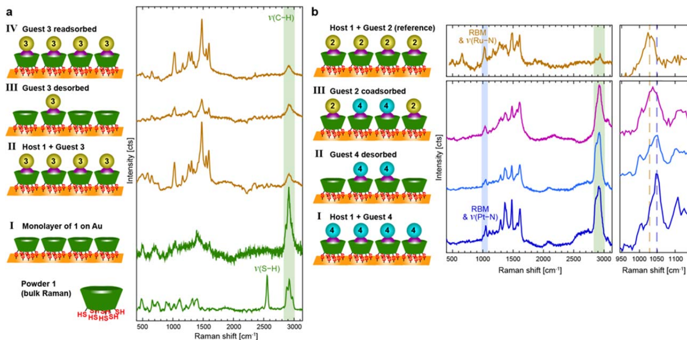
Figure 3. Regeneration and exchange of the catalysts on the host-functionalized Au surface. a) The binding of 1 to Au via all seven thiolate groups is confirmed by the complete absence of the S-H stretching vibration in the TERS spectrum I of 1 -functionalized gold. Reversible adsorption and desorption of 3 on host-functionalized gold is reflected in the varying intensity of the peaks at 1000-1600 cm -1 in spectra II-IV. The spectra are normalized with respect to the C-H stretching band of 1 at 2900 cm -1 (highlighted in green). b) Desorption and subsequent exchange of 4 by 2 on host-functionalized gold is confirmed by the shift of the ring breathing modes (RBM) of the metal-coordinated pyridyl rings from 1050 cm -1 for Pt toward 1030 cm -1 for Ru (highlighted in blue). The incomplete desorption of 4 is reflected in the residual intensity of 4 in spectrum II and in the mixed signals of 4 and 2 in spectrum III.
