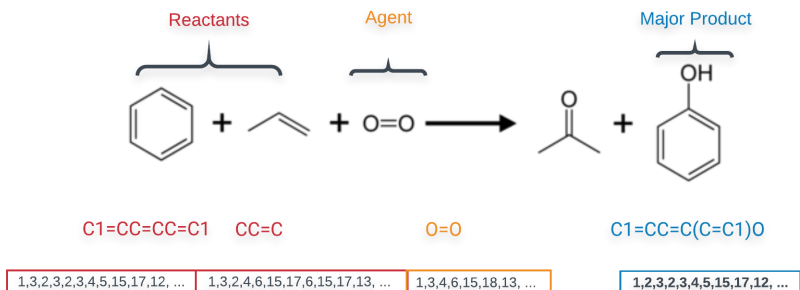
Figure 3: An overview of the proposed grammar-based reaction encoding strategy
