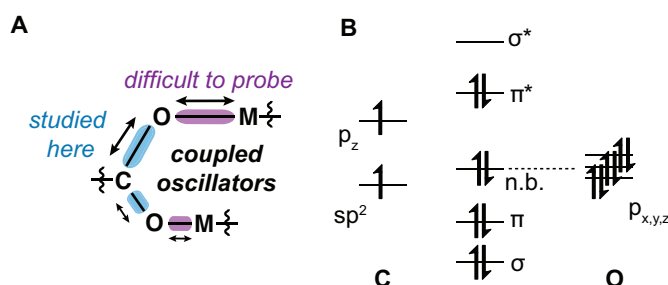
Scheme 1: Molecular orbital (MO) description of MOF metal-carboxylate interactions. (A) Schematic representation of C–O and M–O coupled anharmonic oscillators in metal-carboxylate complexes. (B) MO diagram of carbonyl bond in a carboxylate group.
