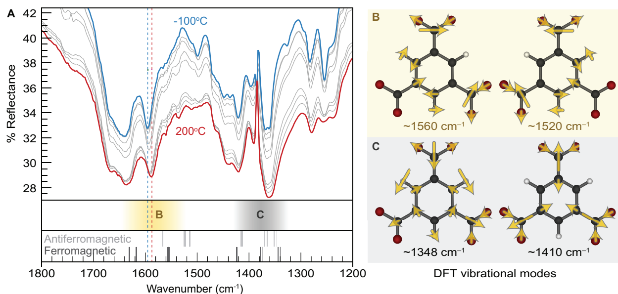
Figure 1: Variable-temperature diffuse reflectance infrared Fourier transform spectra (VT-DRIFTS) and computed phonon modes of HKUST-1. (A) (Top) Experimental spectra collected between -100\text{ }^{\circ}\text{C} and 200\text{ }^{\circ}\text{C} under dynamic vacuum. (Bottom) Simulated peak positions of phonon modes with carboxylate character denoted by color intensity and labeled according to modes show in panel B. (B) Representation of “asymmetric” and (C) “symmetric” carboxylate-based phonon modes projected at the \Gamma q -point.
