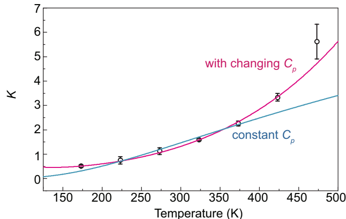
Figure 4: van't Hoff analysis of MOF metal-linker dynamic equilibrium. Inverse stability constants K ([loose]/[tight]) were determined as the ratio of integrated spectral components determined by global curve fitting of the HKUST-1 asymmetric stretch. Data points represent average values from three temperature ramp cycles, with error bars denoting standard deviations. Data were fit to a standard van't Hoff equation assuming constant material specific heat (blue) and an equation with changing specific heat (pink).
