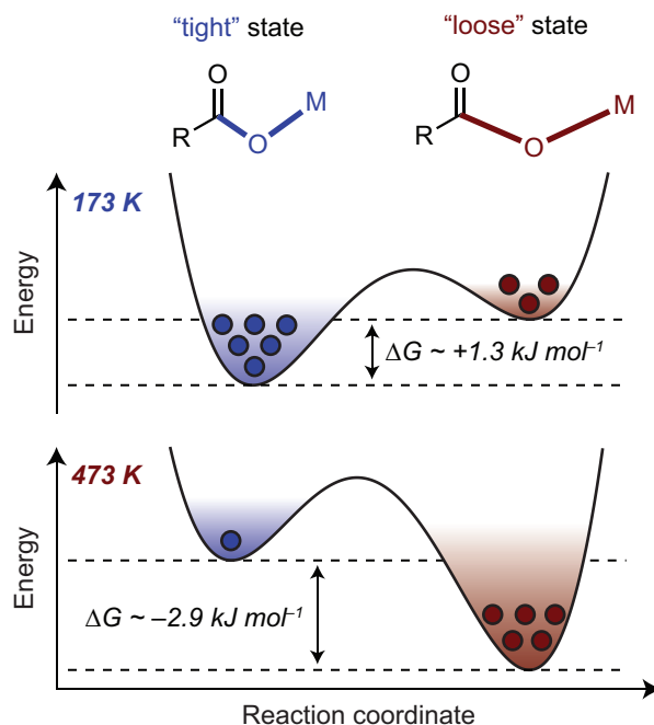
Scheme 2. Equilibrium between “tight” and “loose” ensembles of MOF metal-carboxylate populations existing near thermoneutral equilibrium. (Top) Conversion of MOF metal-linker bonds between two ensemble-averaged states. (Bottom) Temperature-dependent free energies ( \Delta G ) and relative population according to equilibrium constants derived from experimental data.
