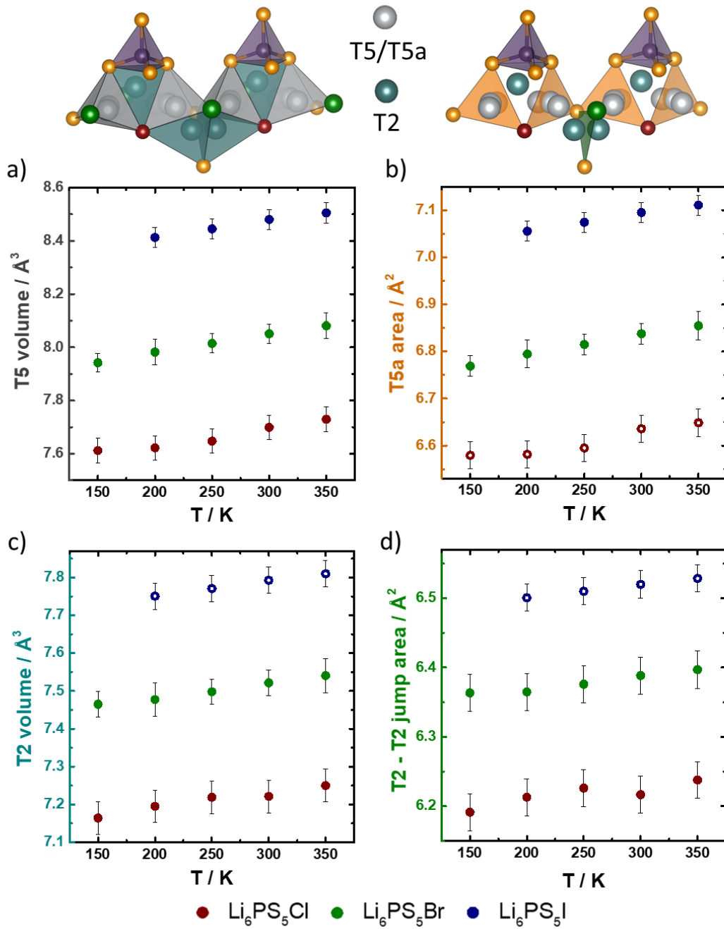
Figure 7: Changing polyhedral volumes and areas along the \text{Li}^+ diffusion pathways with temperature. Closed symbols represent positions that are found occupied, and open symbols site in which no \text{Li}^+ was experimentally found. With increasing temperature, a broadening of the diffusion pathways by expanding \text{Li}^+ polyhedral volumes and transition areas can be found, likely facilitating easier ionic transport.
