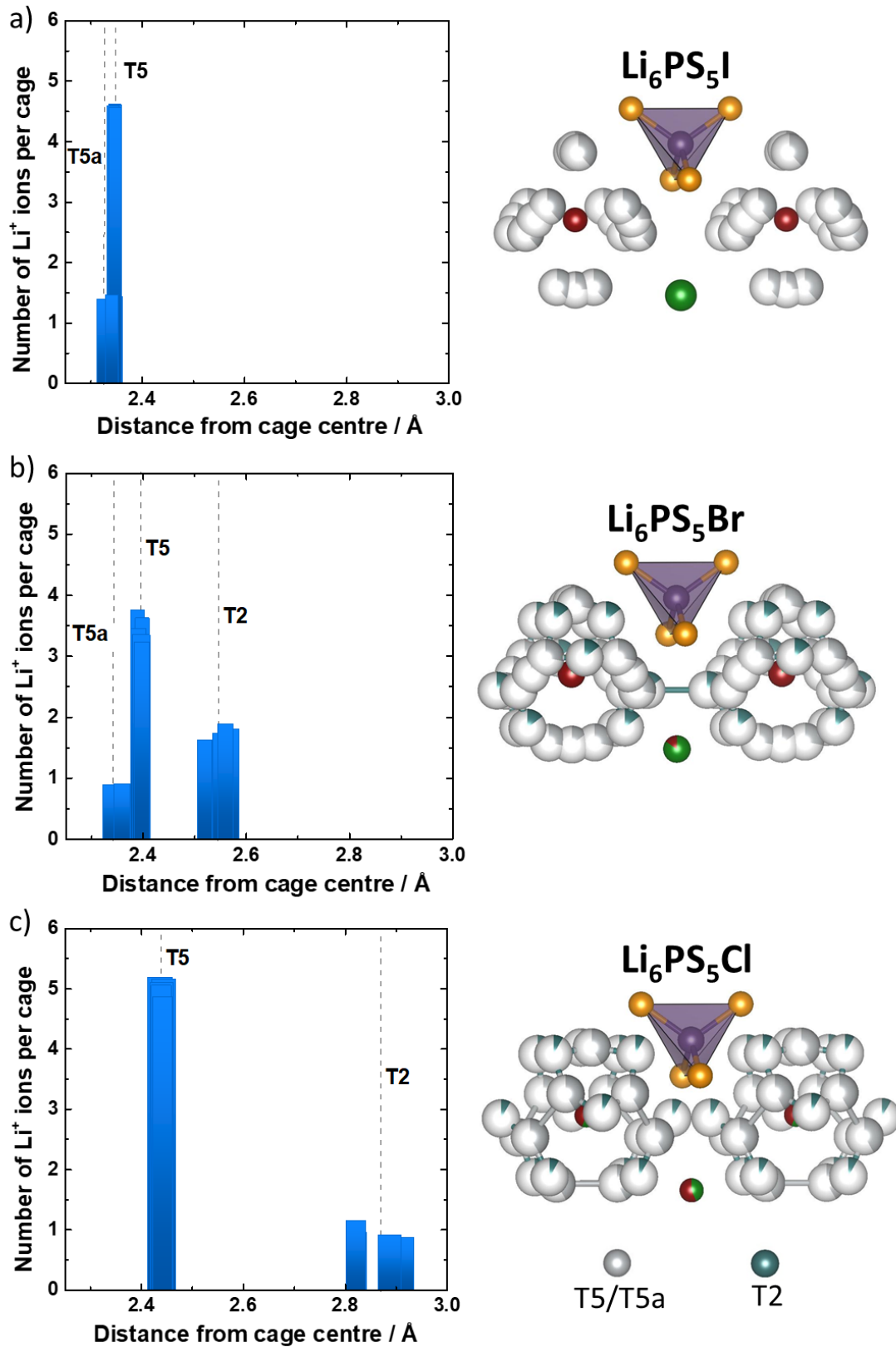
Figure 5: Radial distribution of \text{Li}^+ around the center anion \text{X}^-/\text{S}^{2-} (Wyckoff 4d) in the lithium cage for all temperatures, along with the lithium positions for \text{Li}_6\text{PS}_5\text{X} at 200 K. The radial distribution shows an increasing \text{Li}^+ cage size from \text{Li}_6\text{PS}_5\text{I} to \text{Li}_6\text{PS}_5\text{Cl} , despite the opposite trend in the lattice volume.
