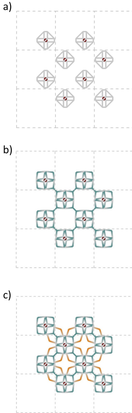
Figure 8: Representation of the \text{Li}^+ connectivity with (a) the T5 and T5a sites (grey) only, (b) including the experimentally found T2 position (blue) and a (c) topologically possible, so far unconfirmed, T4 site (orange). Diffusion trajectories involving T5 sites only form discontinuous face-sharing tetrahedral pathways.
