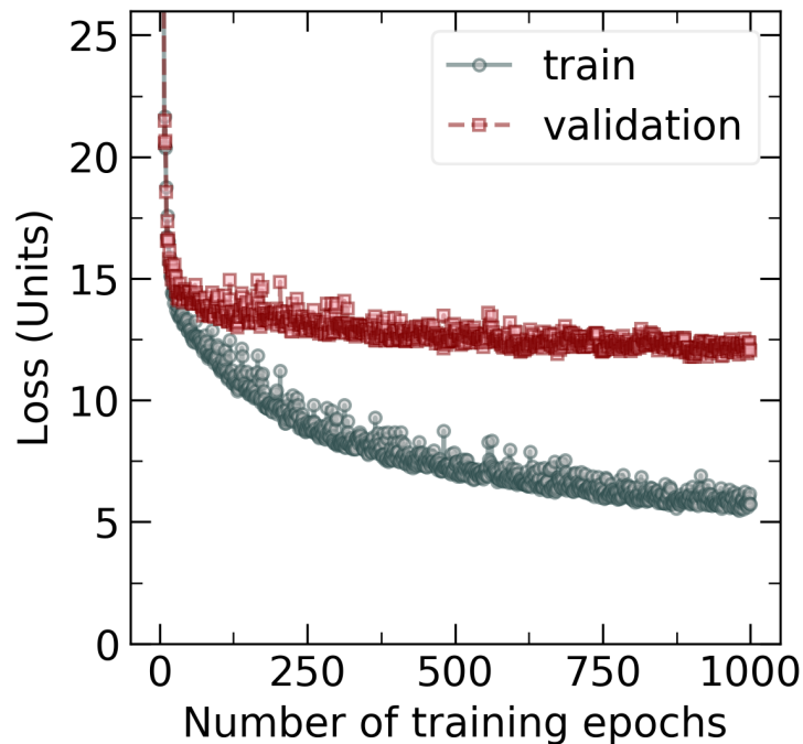
Figure 4: Example loss curve plot of a neural network, showing model performance (loss) evaluated on the train and validation datasets at each epoch throughout the training process. A lower loss indicates a better-performing model.
