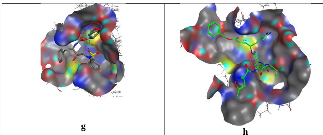
Fig. 4: Surface and maps of compounds aliskiren a , dipyridamole b , mopidamol c , rosuvastatin d , metamizole e , rolitetracycline f , darunavir g , and N3 h into the N3 binding site in the COVID-19 protease.
