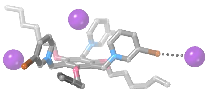
Fig. 5 The asymmetric unit of 3-I 3 . Hydrogen atoms have been omitted for clarity.
