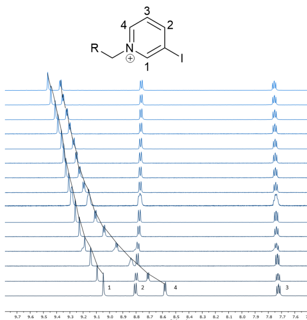
Fig. 2 Truncated ^1\text{H} -NMR spectra of 6\text{-(PF}_6)_3 upon addition of TBA-Cl (9:1 \text{CD}_3\text{CN}:\text{d}_6\text{-DMSO} , 600 MHz, 298 K). 40
