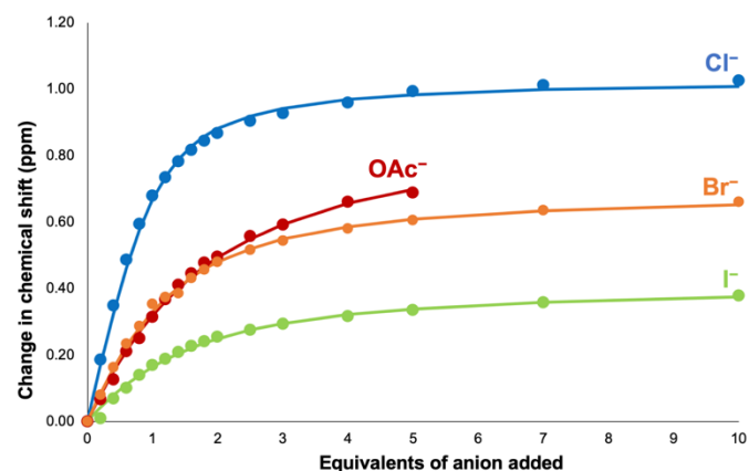
Fig. 3 ^1\text{H} NMR binding curve for addition of TBA-Cl, TBA-Br, TBA-I and TBA-OAc to 5\text{-(PF}_6)_3 , showing the change in chemical shift of \text{H}_4 (9:1 \text{CD}_3\text{CN}:\text{d}_6\text{-DMSO} , 298 K). Dots represent the observed points and the line represents 1:1 binding isotherms fitted using Bindfit. 41 Precipitation was observed after addition of five equivalents of TBA-OAc.
