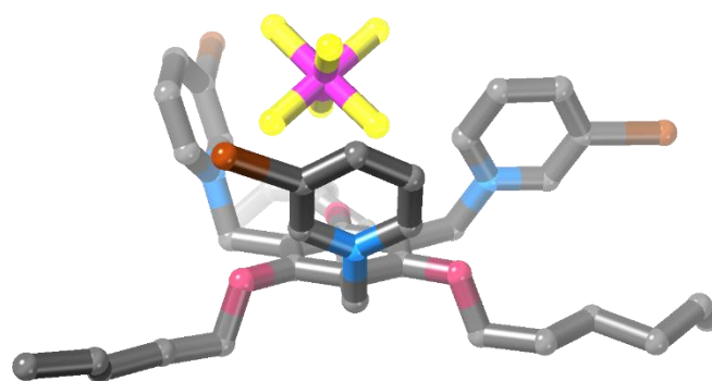
Fig. 4 Crystal structure of 3\text{-(PF}_6)_3 . Hydrogen atoms, disorder of one bromopyridinium ring and counter ions omitted for clarity.
