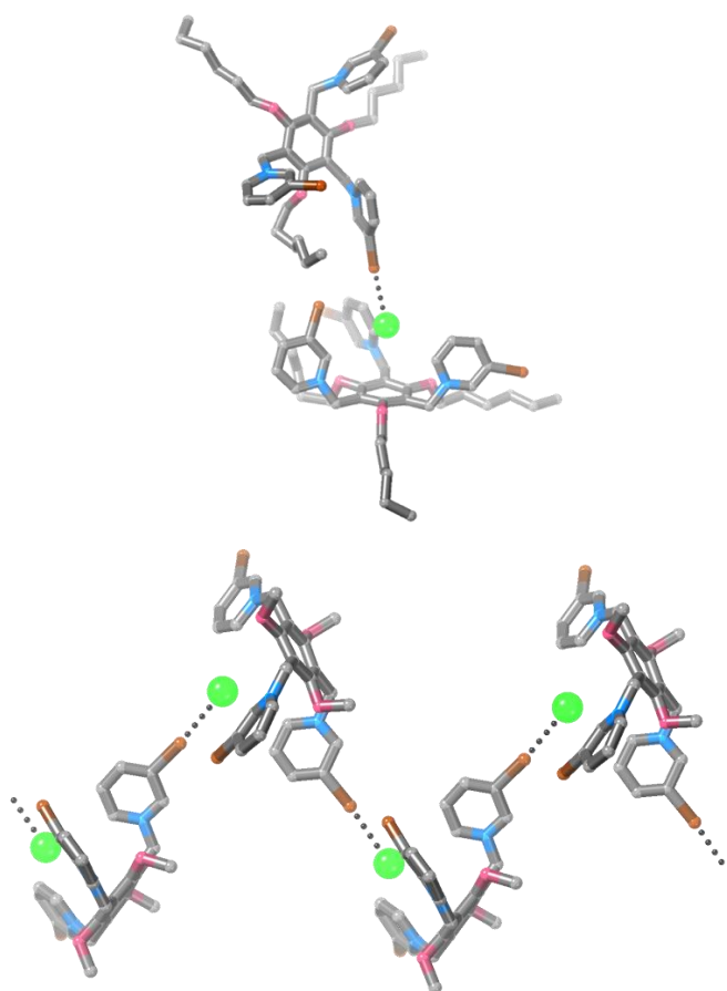
Fig. 7 Two views of the structure of 3-Cl 3 showing the 1D polymeric structure. Hydrogen atoms, disorder, solvent molecules and some chloride anions have been omitted for clarity.
