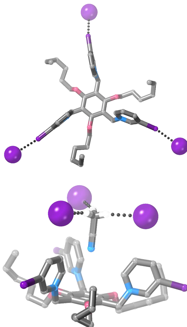
Fig. 6 Two views of the crystal structure of 4-I 3 (most hydrogen atoms are omitted for clarity, as is the acetonitrile solvent molecule in the top view of the structure).
