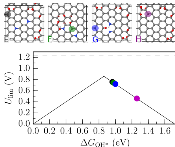
Figure 8. Volcano plot for the 4e^- ORR where the limiting potential is plotted as a function of the free energy of the adsorbed \text{OH}^* intermediate (incl. the estimated solvation correction of -0.4 eV). Colored circles describe different adsorption sites that are marked correspondingly on the NrGO-4 model structures in panels E-H. The equilibrium ORR potential is depicted by the dashed line at 0.86 V_{\text{RHE}} , while the top of the volcano at 0.86 V_{\text{RHE}} represents the ideal catalyst with a minimum overpotential of 0.37 V due to \text{OOH}^*/\text{O}^*/\text{OH}^* scaling relations.
