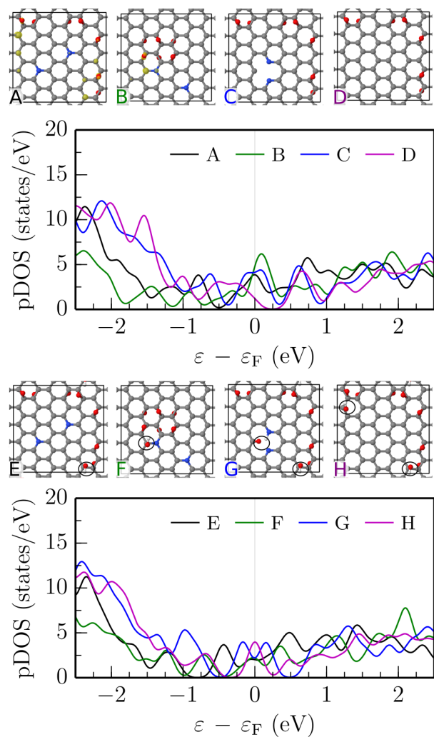
Figure 7. Theoretical models for the catalytic NrGO-4 surface. Panels A-H show the (A-D) clean and (E-H) corresponding saturated structures with overlaid isosurface of the spin electron density (cutoff 0.05 \text{ \AA}^3 ) in yellow. The box shows the repeated unit cell in the DFT calculations, while gray, red, yellow, and white spheres represent C, O, N, and H atoms respectively. Circles identify the adsorbed OH(aq) in panels E-H due to alkaline conditions. Plotted below each set of structures is the corresponding projected density of states (pDOS) in eV^{-1} vs energy relative to the Fermi level.
