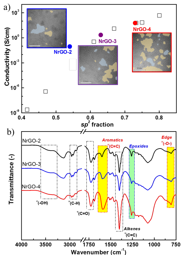
Figure 1. Physical and chemical results of NrGO catalysts. (a): Solid circles represent the electrical conductivity of 50 nm films of NrGO catalysts vs. the sp^2 fraction of the total number of carbon atoms as determined by XPS. White squares are the electrical conductivity of three-monolayer films of rGO vs the carbon sp^2 fraction, from the work of Chhowalla and coworkers (data reproduced with permission from John Wiley and Sons). 20 The insets show representative HR-TEM of the three catalysts (larger versions of these images can be found in Figure S3). The orange regions cover the largest nm-sized sp^2 carbon patches and the blue regions indicate holes in the platelet. The gray regions are mostly sp^3 carbon. (b): IR spectra of the three NrGO catalysts. Assumed functional group assignments are labeled. The alkyl C-N frequencies are in the broad structureless feature around 1050 cm^{-1} .
