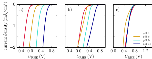
Figure 3. ORR cathodic linear sweep voltammetry (current density in \text{mA/cm}^2 vs applied U in volts relative to the reversible hydrogen electrode) at the pH values indicated in the figure's legend. Panels (a), (b), (c) refer to measurements at the NrGO-2, NrGO-3, NrGO-4 catalysts respectively.
