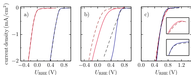
Figure 4. ORR cathodic linear sweep voltammetry (current density in \text{mA}/\text{cm}^2 vs applied potential U in volts relative to the reversible hydrogen electrode in protonated (solid lines) and deuterated (dashed lines) solutions. Colored lines are for \text{pH}(\text{D})=1 in crimson (dark red) and \text{pH}(\text{D})=13 in blue (black). Panels (a), (b), (c) refer to measurements at the NrGO-2, NrGO-3, NrGO-4 catalysts respectively. Insets in panel (c) zoom in to magnify the small H/D isotope effect in NrGO-4 for \text{pH}(\text{D})=1 (top) and \text{pH}(\text{D})=13 (bottom).
