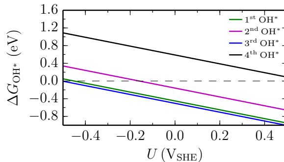
Figure 6. Pourbaix diagram (free energy of adsorption vs potential U in volts relative to the standard hydrogen electrode) depicting the relative stability for the sequential adsorption of OH^-(aq) species at the NrGO-2 model structure depicted in Figure 5A in alkaline solution, pH=13. In each case the most favorable adsorption sites are considered and the estimated OH^* solvation correction of -0.4 eV is included.
