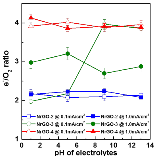
Figure 2. Electron transfer number ( e^-/\text{O}_2 ) for the three NrGO catalysts as a function of pH at both low overpotential and higher overpotential. The overpotentials were selected so that ORR current density corresponds to 0.1 \text{ mA/cm}^2 and 1.0 \text{ mA/cm}^2 . The e^-/\text{O}_2 ratio is obtained by in-situ pressure decay measurement of the calibrated volume \text{O}_2 headspace during chronoamperometry.
