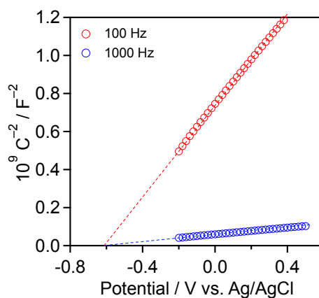
Figure S3. Mott-Schottky plot of the \text{MgCr}_2\text{S}_4/\text{FTO} electrode measured in aqueous \text{NaH}_2\text{PO}_4\text{-Na}_2\text{HPO}_4 solution ( \text{PO}_4^{3-} = 0.1 \text{ M} ) at pH 7.0. The electrode was prepared by electrophoretic deposition in a 50 mL acetone solution (>99.5%, Kanto Chemical) containing 0.05 g \text{MgCr}_2\text{S}_4 powder (synthesized under \text{Na}_2\text{S} excess condition) and 10 mg iodine (>99.8%, Wako Pure Chemicals). Two parallel FTO electrodes were immersed in the solution with ca. 15 mm separation, and a 20 V bias was applied between them for 30 s using a potentiostat (PSW 80-13.5, GW Instek). The \text{MgCr}_2\text{S}_4 -coated area was fixed ca. 1.5 \text{ cm} \times 3.5 \text{ cm} .
