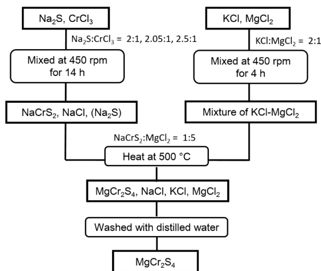
Scheme 1. Two-step metathesis flux synthesis of \text{MgCr}_2\text{S}_4 .
