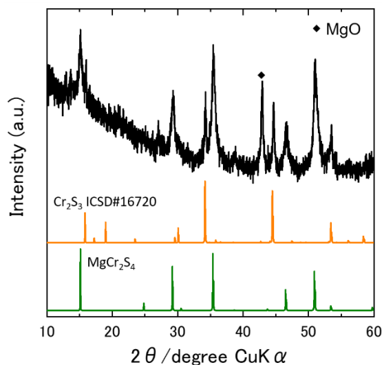
Figure S1. XRD pattern of \text{MgCr}_2\text{S}_4 synthesized from \text{NaCrS}_2 and \text{MgBr}_2\text{-KBr} flux with excess \text{Na}_2\text{S} and subsequent washing with methanol.
