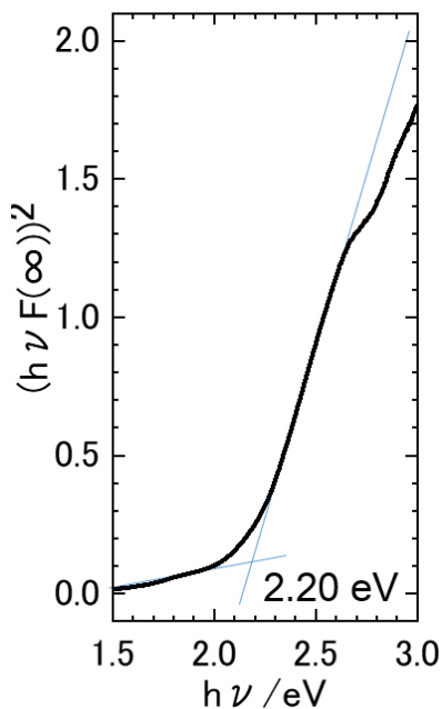
Figure S2. Tauc plot of \text{MgCr}_2\text{S}_4 powders synthesized under \text{Na}_2\text{S} excess condition.
