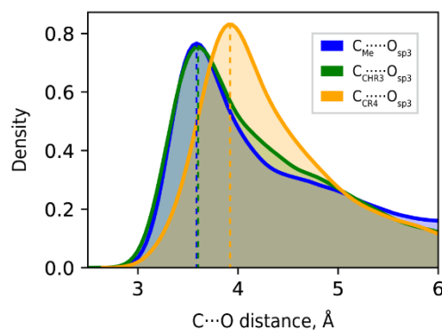
Figure 4. Distance distribution of C...O sp3 line-of-sight contacts for different carbon types. Gaussian kernel density estimations used instead of histograms for the purpose of clarity.
