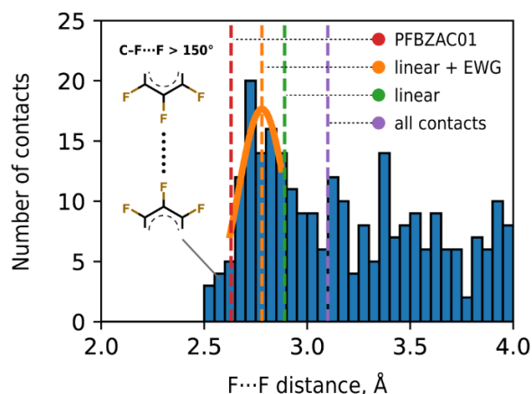
Figure 6. Distance distribution for linear ( C-F\cdots F > 150^\circ ) intermolecular F\cdots F contacts between two electron-withdrawing fragments. From left to right: red dashed line denotes the shortest F\cdots F intermolecular distance in PFBZAC01; orange line stands for D_{max} of linear F\cdots F contacts between two aromatic fragments; green and purple lines stand for D_{max} of linear and all F\cdots F contacts, respectively.
