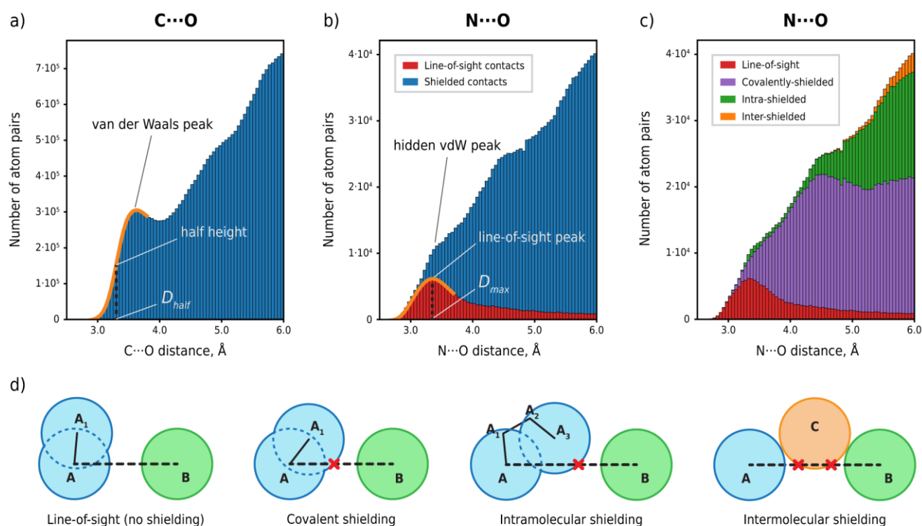
Figure 1. Distance distributions for all intermolecular C...O (a) and N...O (b,c) intermolecular contacts from molecular crystals in CSD. The contacts between atom pairs are classified (c) as the line-of-sight and various shielded contacts. The respective contributions to the overall contact distance distributions of r(\text{N}\cdots\text{O}) are presented in parts (b,c).
