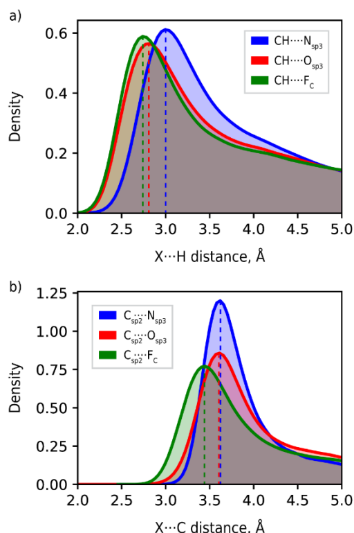
Figure 3. Distance distribution of C-H...X line-of-sight contacts for X = N, O, F. Gaussian kernel density estimation [19] is used instead of histograms for the purpose of clarity.
