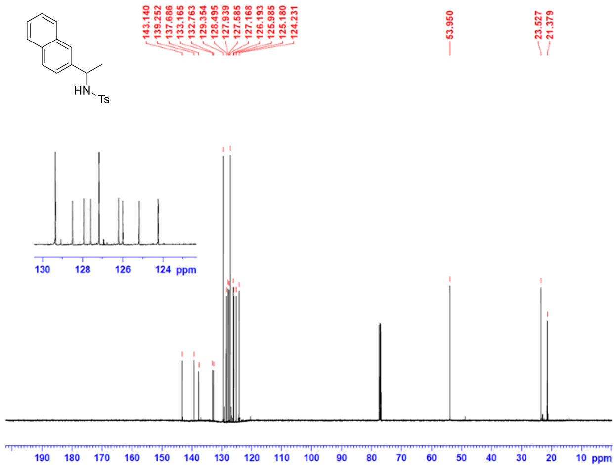
Figure S19. ^{13}\text{C} NMR of 4-Methyl-N-(1-(naphthalen-2-yl)ethyl)benzenesulfonamide in \text{CDCl}_3 .
