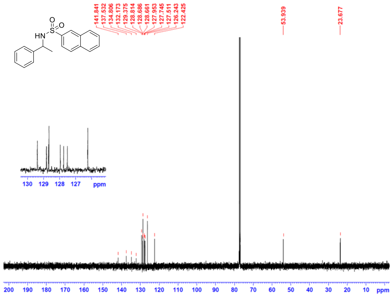
Figure S23. ^{13}\text{C} NMR of N-(1-Phenylethyl)naphthalene-2-sulfonamide in \text{CDCl}_3 .
