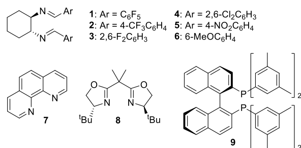
Scheme 2. Ligands Used in Reaction Optimization.
