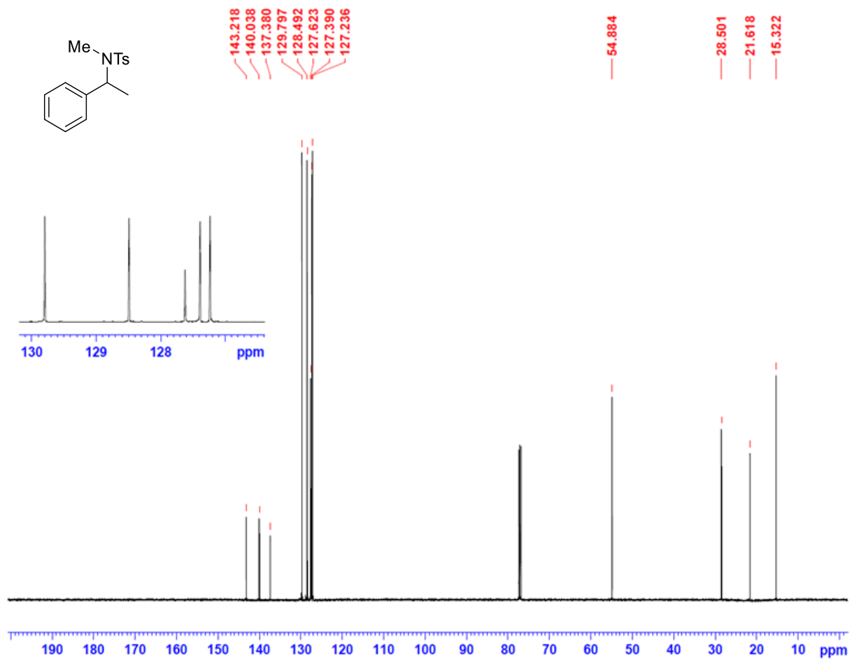
Figure S21. ^{13}\text{C} NMR of N,4-Dimethyl-N-(1-phenylethyl)benzenesulfonamide in \text{CDCl}_3 .
