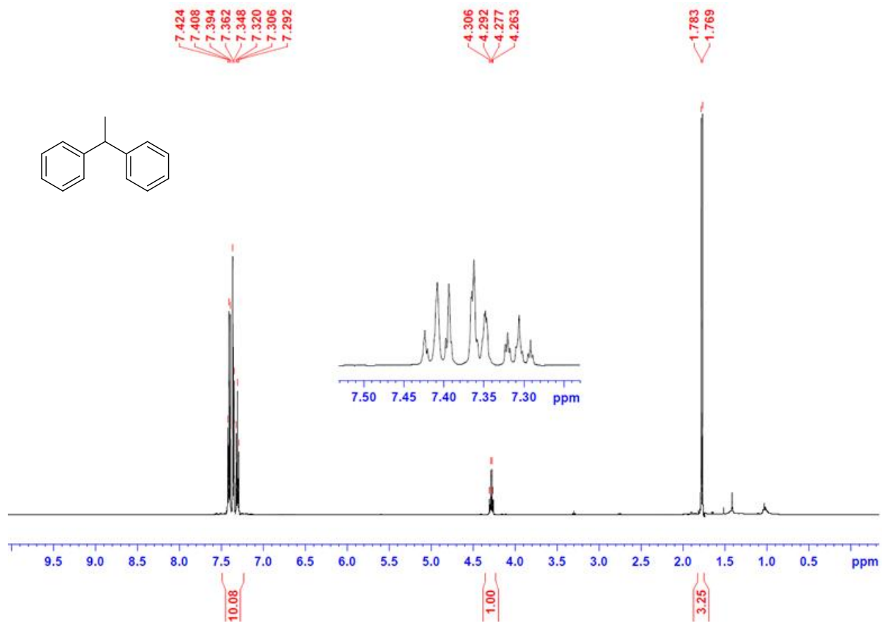
Figure S2. 1 H NMR of Ethane-1,1-diyldibenzene in CDCl 3 .
