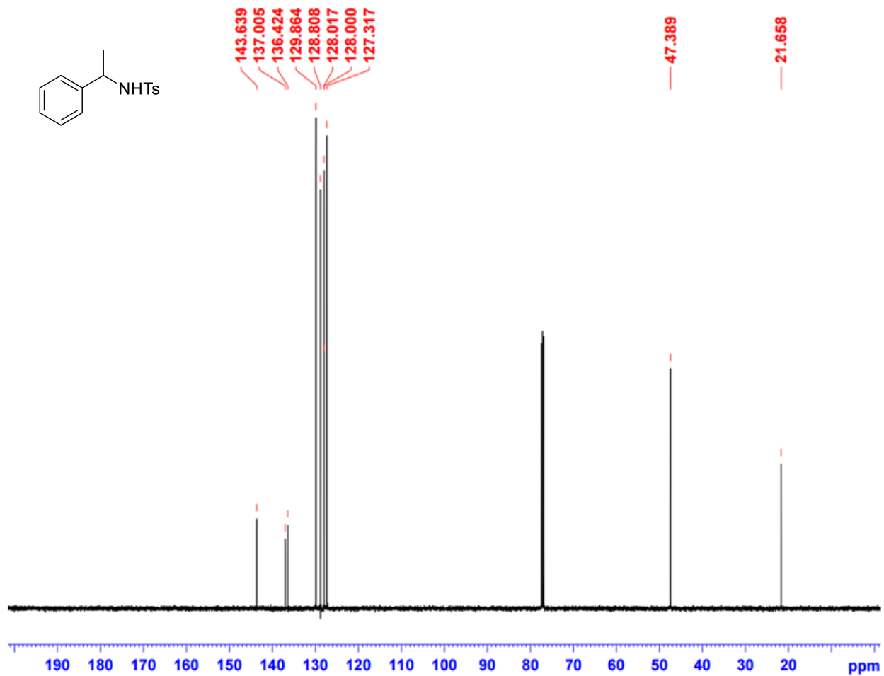
Figure S5. 13 C NMR of N -Benzyl-4-methylbenzenesulfonamide in CDCl 3 .
